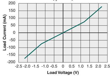
Form-B Typical Load Current vs. Load Voltage ( I_F=5\text{mA} )
