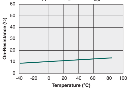
Form-B Typical On-Resistance vs. Temperature ( I_F=5\text{mA} , I_L=170\text{mA}_{DC} )
