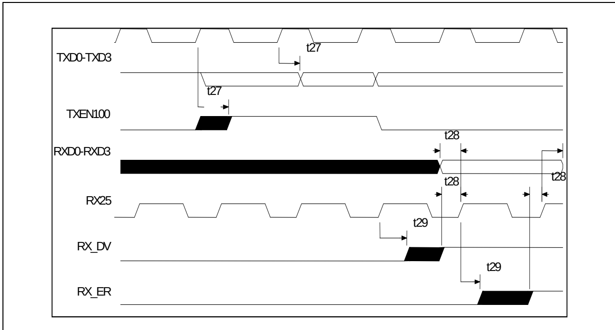
FIGURE 14-10: MII TIMING
