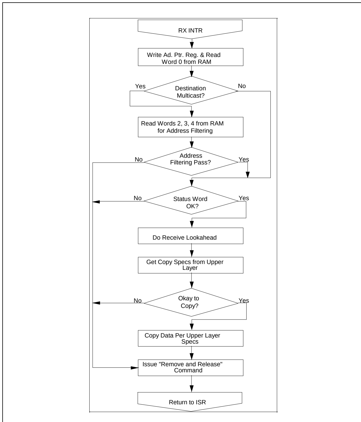
FIGURE 10-2: RX INTR
