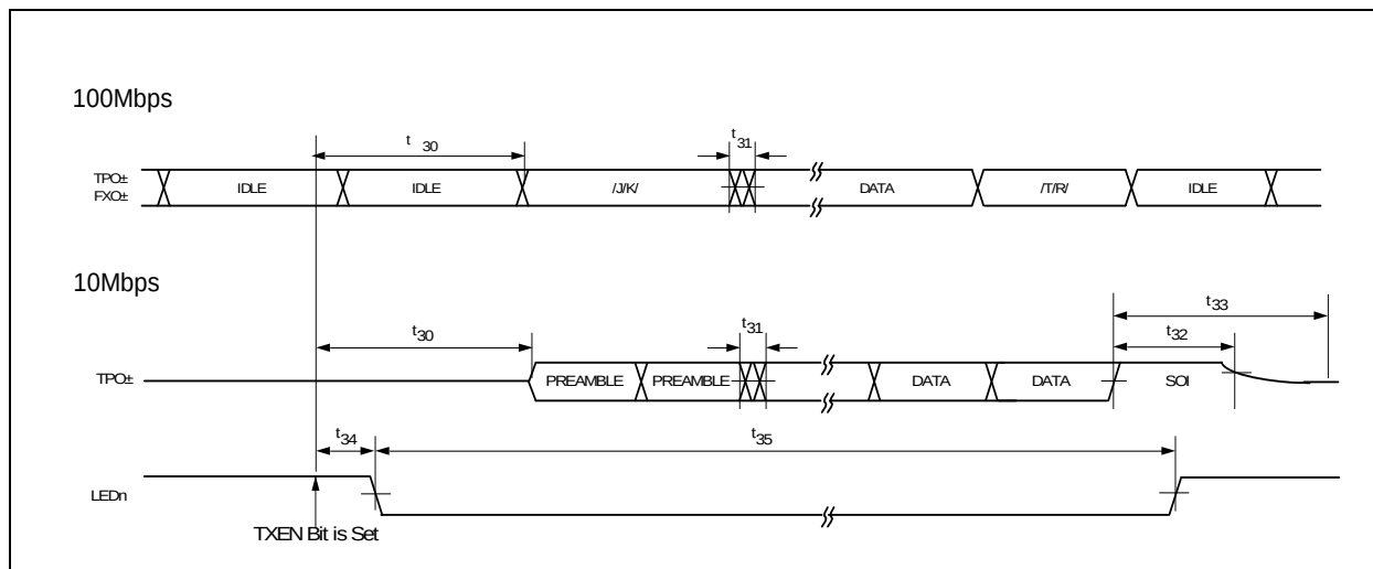
FIGURE 14-11: TRANSMIT TIMING
