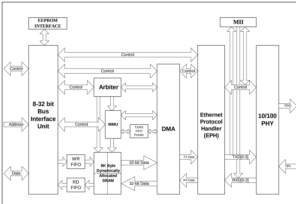
FIGURE 3-2: BLOCK DIAGRAM
