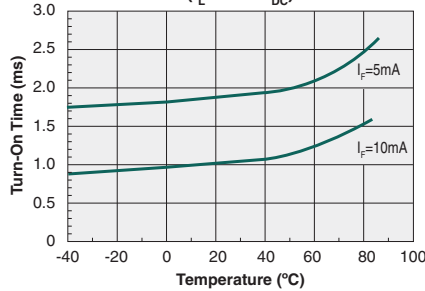
Typical Turn-On Time vs. Temperature ( I_L=80mA_{DC} )
