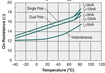
Typical On-Resistance vs. Temperature ( I_L=170mA_{DC} )
