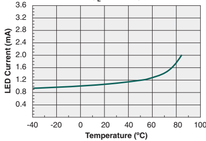
Typical I_F for Switch Operation vs. Temperature ( I_L=170mA )
