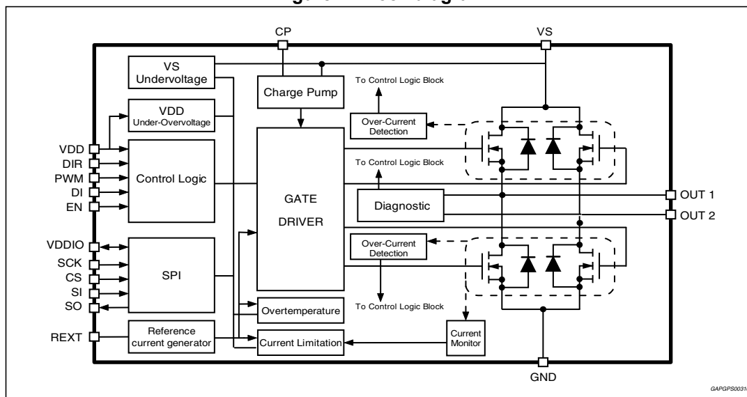
Figure 1. Block diagram
