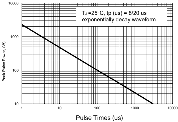
FIG.3- Power Dissipation Versus Pulse Time
