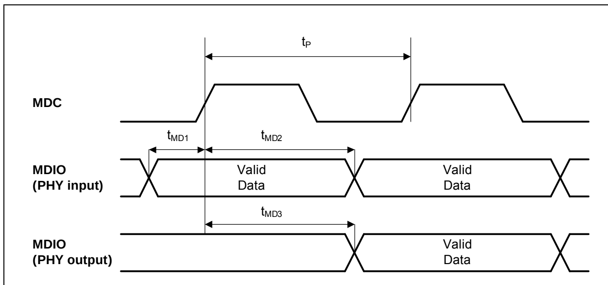
FIGURE 6-3: MDC/MDIO TIMING
