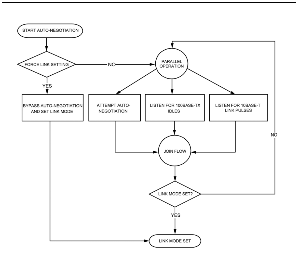
FIGURE 3-3: AUTO NEGOTIATION FLOW CHART
