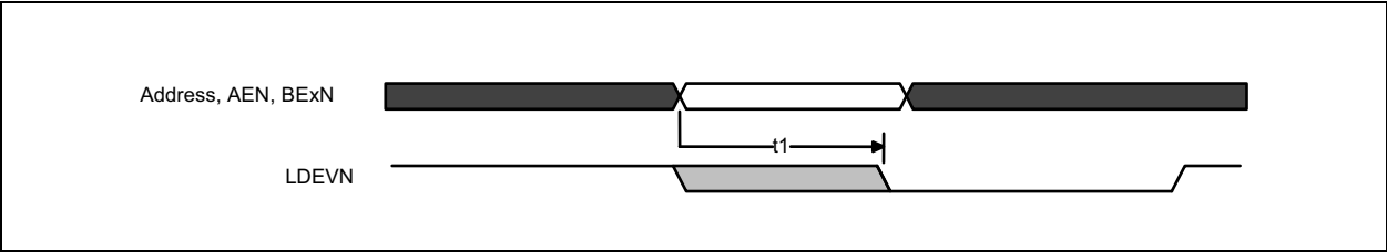
FIGURE 7-2: ADDRESS LATCHING CYCLE FOR ALL MODES
