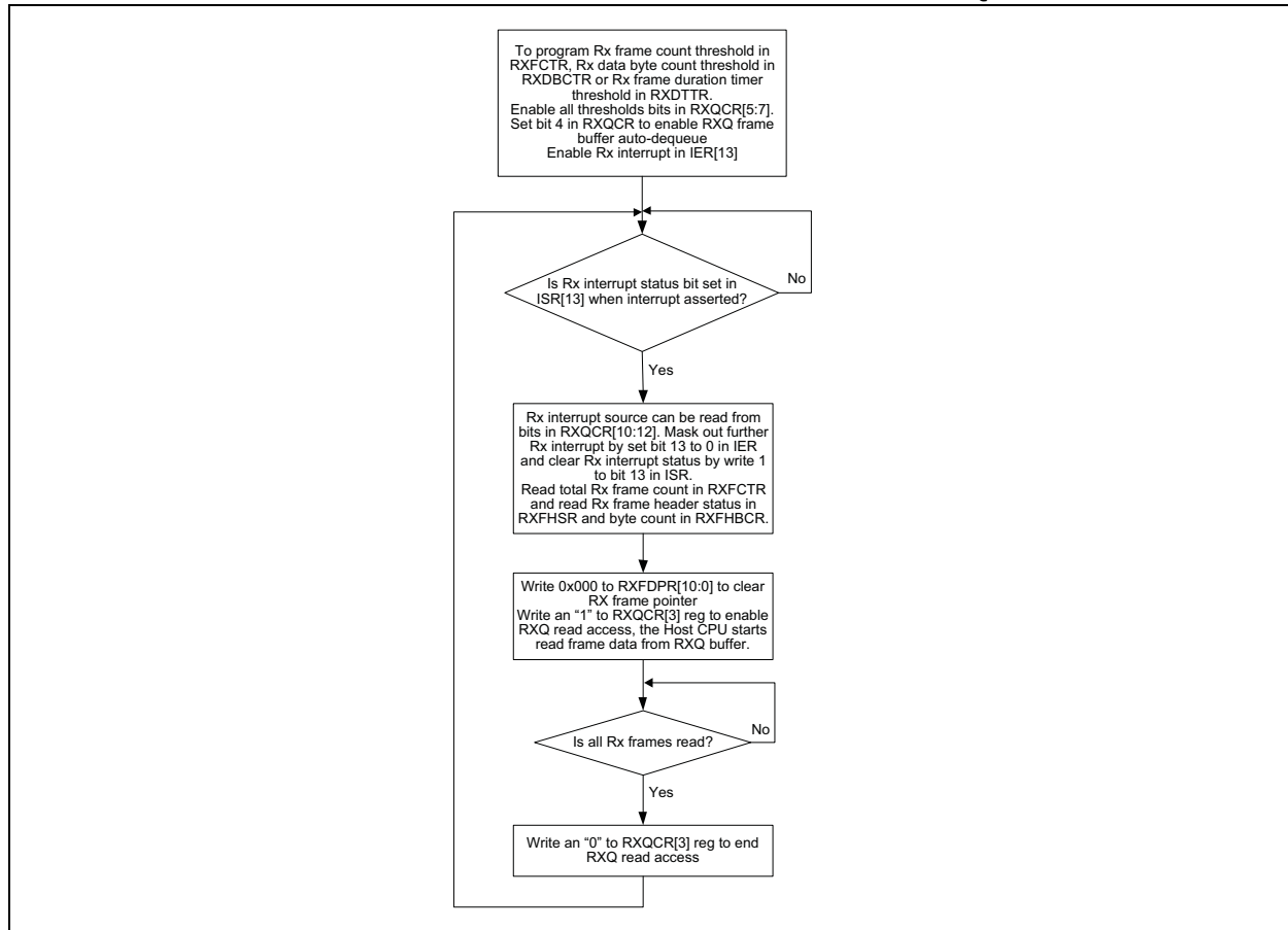
FIGURE 3-6: HOST RX SINGLE OR MULTIPLE FRAMES IN AUTO-DEQUEUE FLOW DIAGRAM
