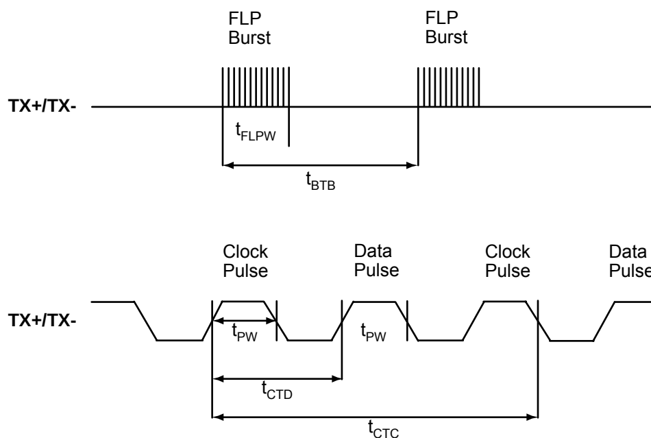
Figure 8. Auto-Negotiation Timing
