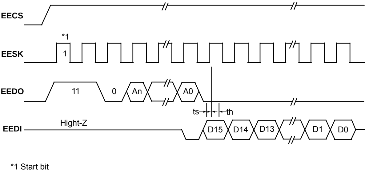
Figure 7. EEPROM Read Cycle Timing Diagram
