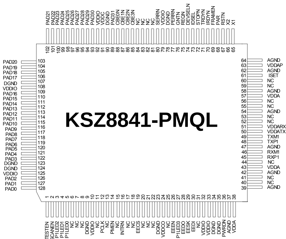
Figure 2. KSZ8841-PMQL 128-Pin PQFP (Top View)
