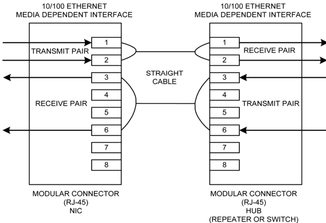
Figure 4. Typical Straight Cable Connection
