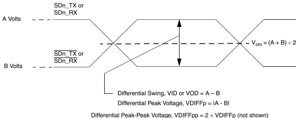
Figure 38. Differential Voltage Definitions for Transmitter or Receiver
