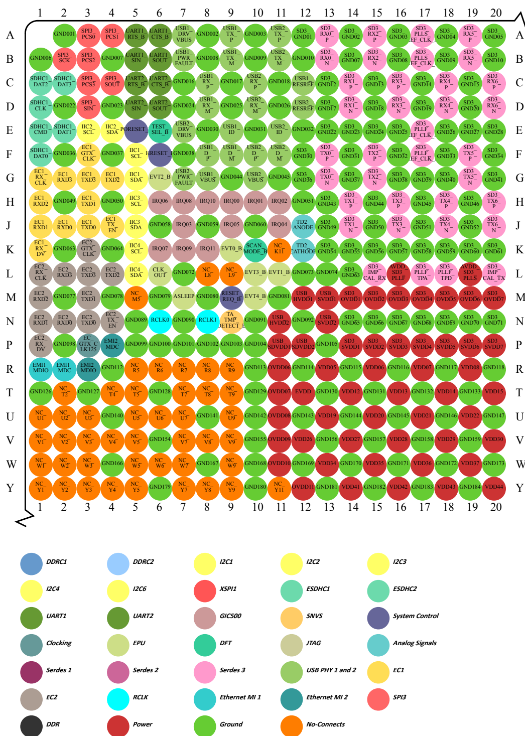
Figure 5. Detail A
