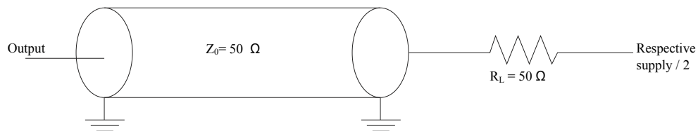
Figure 29. Flextimer AC test load
