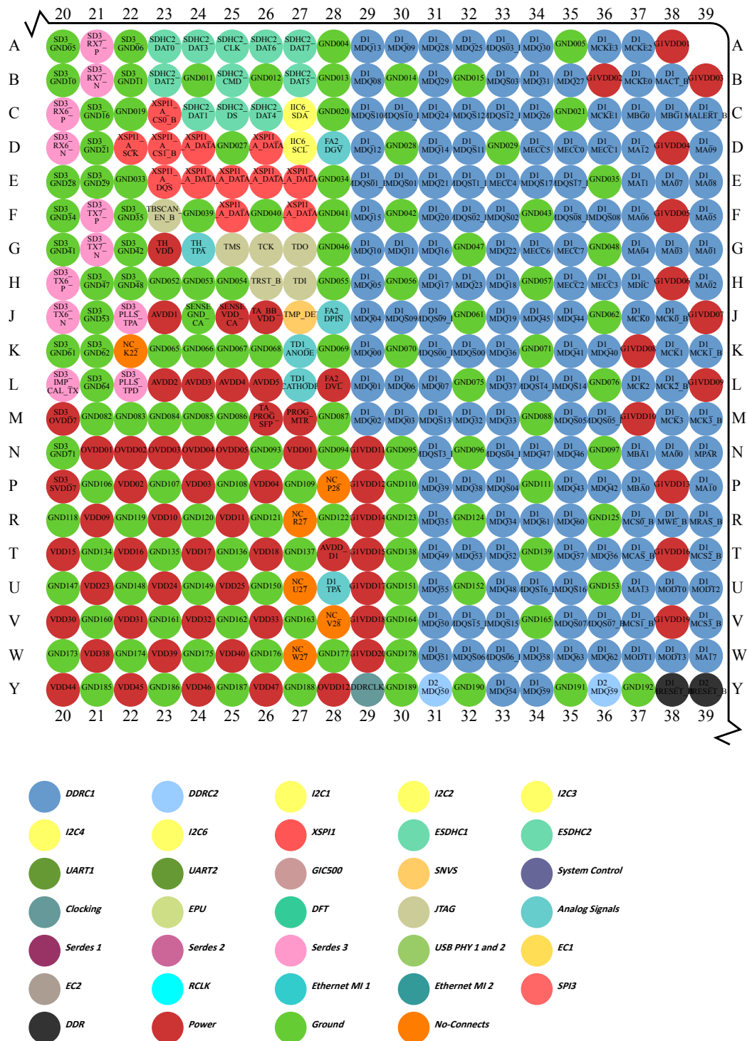
Figure 6. Detail B
