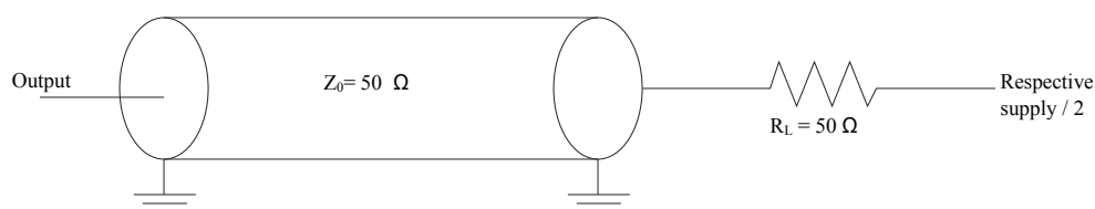
Figure 28. GPIO AC test load
