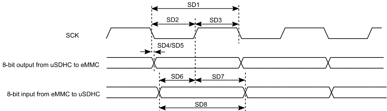
Figure 16. SDR50/SDR104 timing
