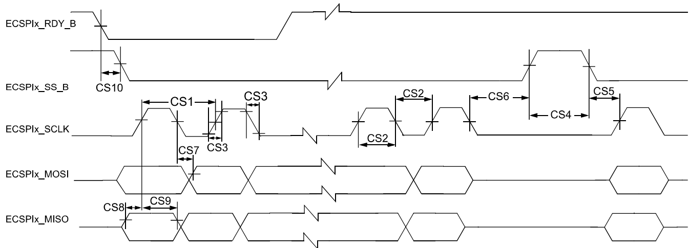
Figure 10. ECSPi Master mode timing diagram
