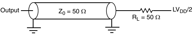
Figure 16. eTSEC AC test load
