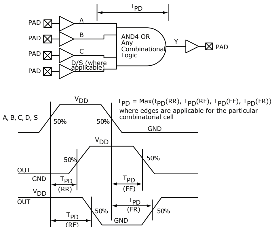
FIGURE 3-14: LUT-4
