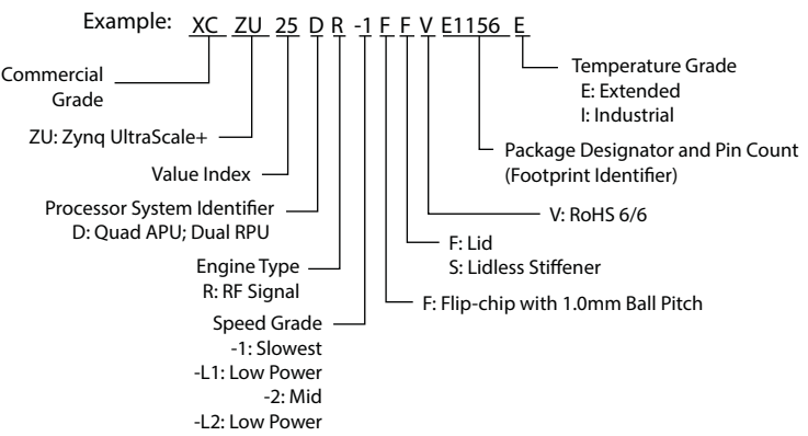
Figure 2: Zynq UltraScale+ RFSoc Ordering Information
