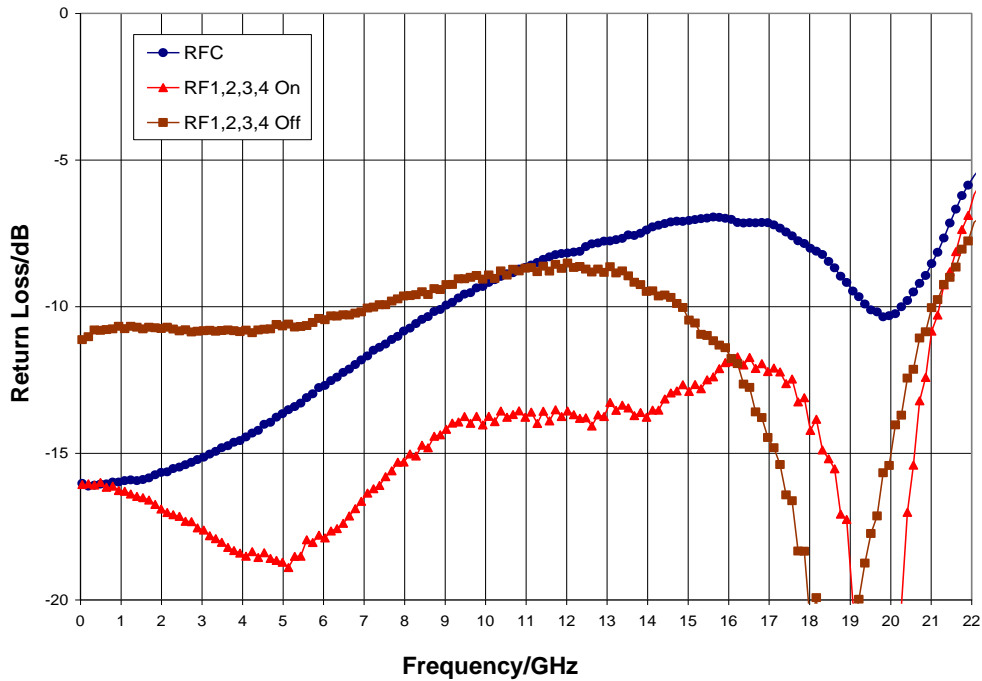
Return Loss
