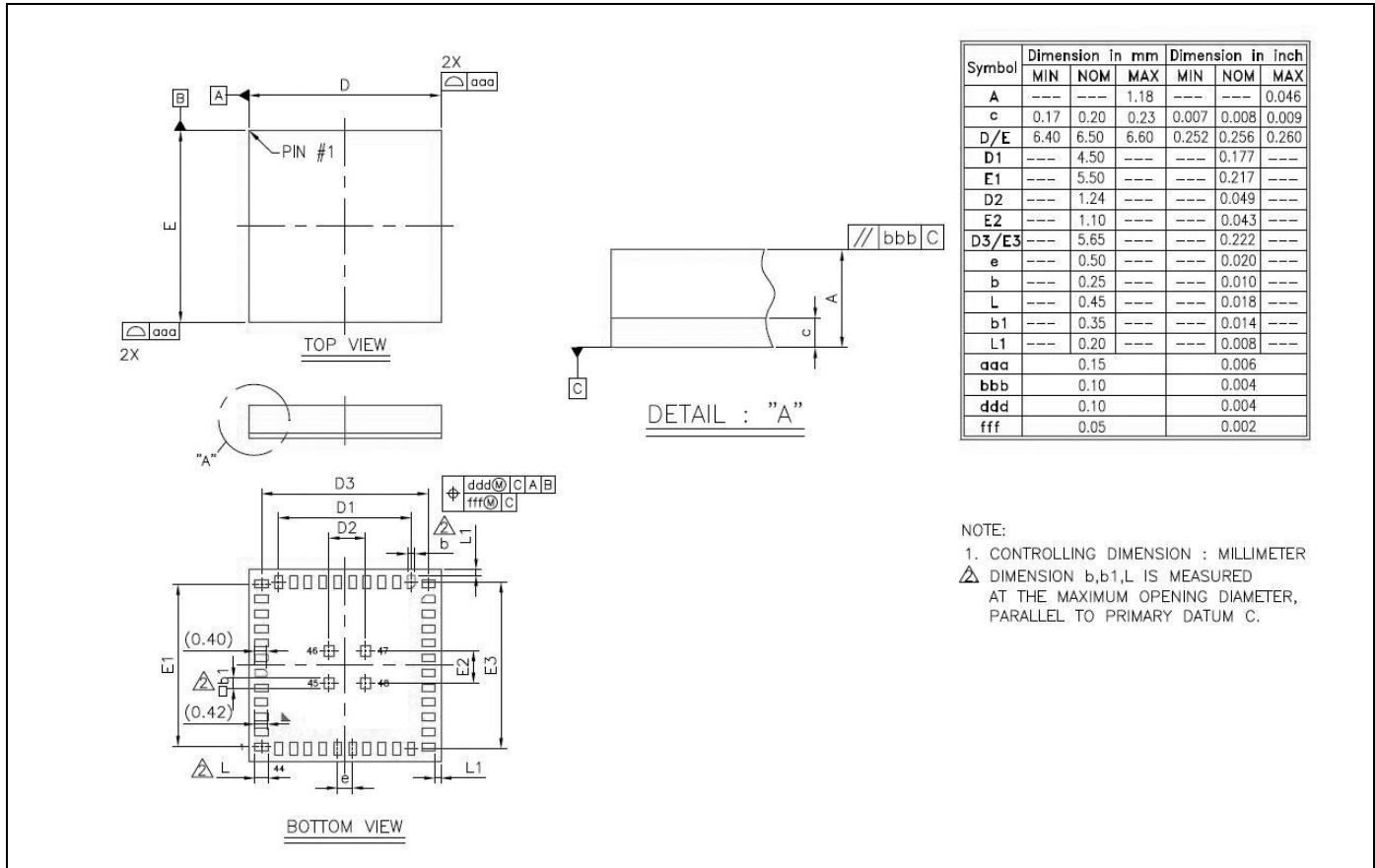
Figure 14. CYW20737L Package Dimensions
