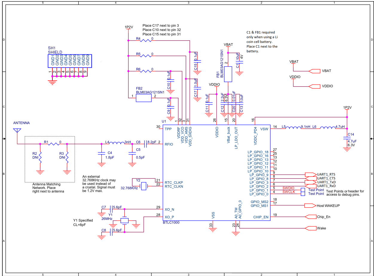
Figure 13-1. ATBTLC1000 QFN Reference Design (4-wire)
