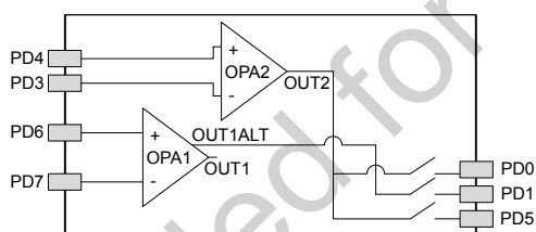
Figure 5.2. Opamp Pinout
