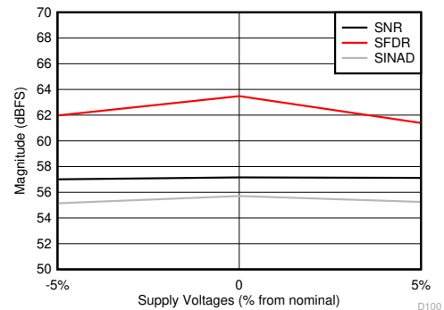
Figure 6-60. SNR, SFDR and SINAD vs Supply Voltage
