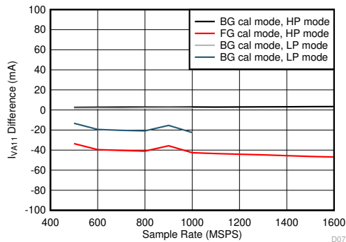
Figure 6-117. Single Channel, I_{VA11} Change with Calibration Mode
