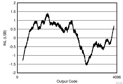
Figure 6-2. INL vs Code
