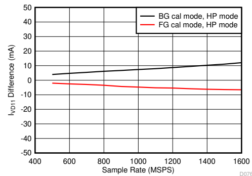
Figure 6-118. Quad Channel, I_{VD11} Change with Calibration Mode
