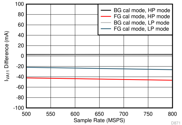
Figure 5-86. Quad Channel, I_{VA11} vs F_S over Modes
