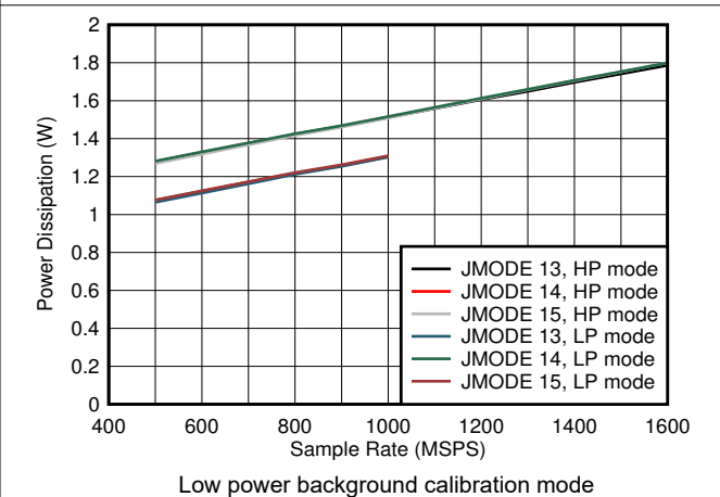
Figure 6-92. Dual Channel, Power Dissipation vs F_S and JMODE 13 - 15
