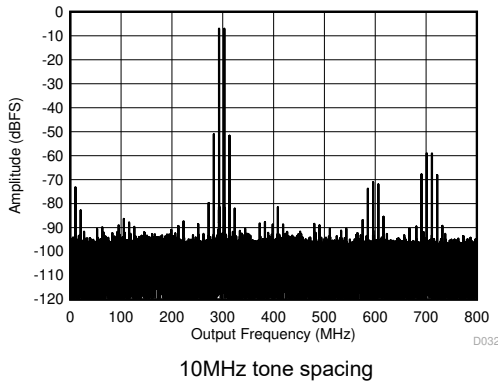
10MHz tone spacing Figure 6-71. Two Tone FFT at 3498MHz
