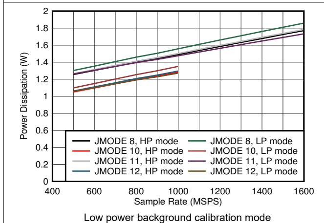
Figure 6-91. Dual Channel, Power Dissipation vs F_S and JMODE 8 - 12
