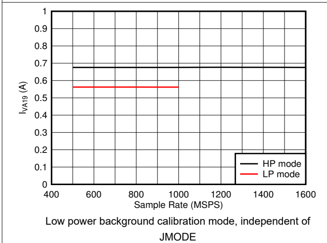
Figure 6-83. Quad Channel, I_{VA19} vs F_S
