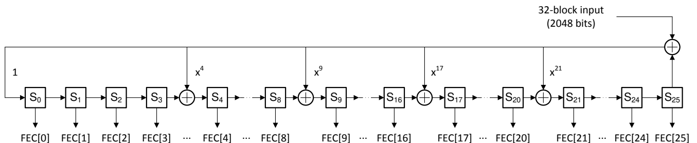
Figure 7-10. FEC Parity Bit Generator
