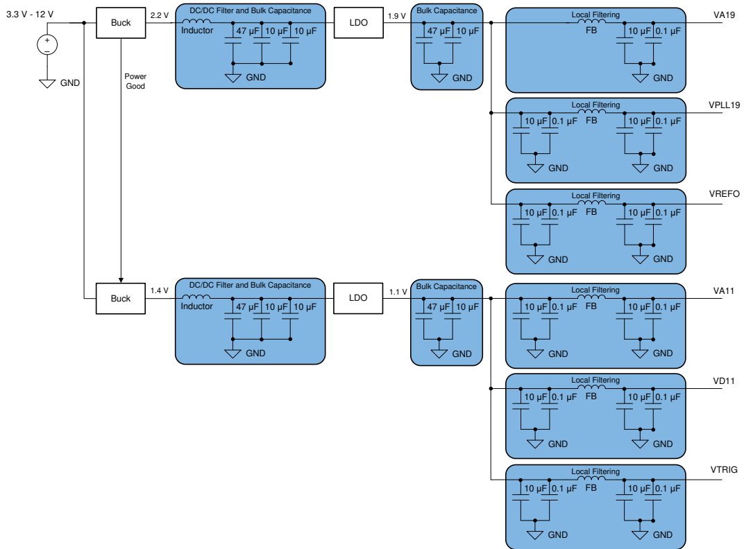
Figure 8-3. LDO Linear Regulator Approach Example
