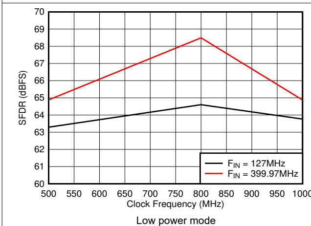
Figure 6-27. SFDR vs Sample Rate
