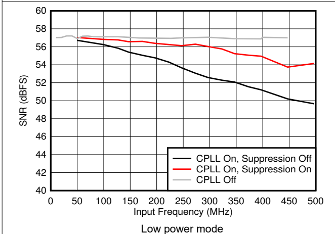
Figure 6-45. SNR vs F_{IN} and C-PLL modes
