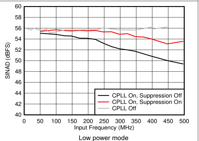
Figure 6-46. SINAD vs F_{IN} and C-PLL modes
