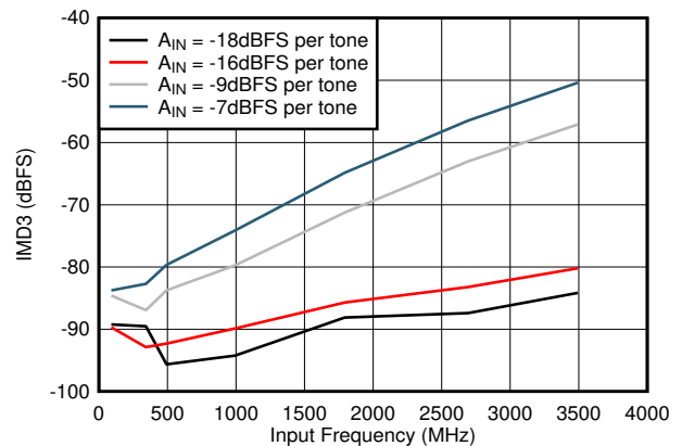
10MHz tone spacing, Low power mode, 1000MSPS Figure 6-76. IMD3 vs F_{IN}
