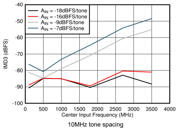
10MHz tone spacing Figure 6-75. IMD3 vs F_{IN}
