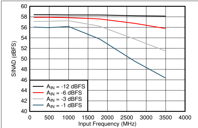
Figure 6-19. SINAD vs Input Frequency
