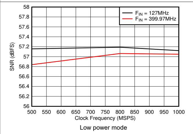
Figure 6-28. SNR vs Sample Rate
