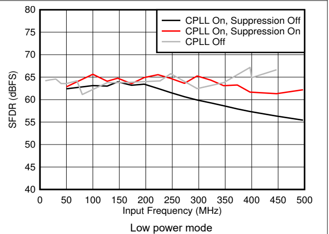
Figure 6-44. SFDR vs F_{IN} and C-PLL modes
