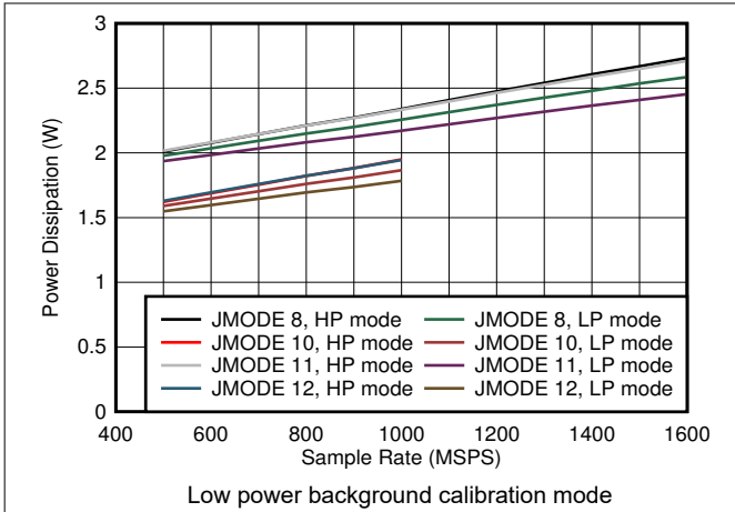
Figure 6-81. Quad Channel, Power Dissipation vs F_S and JMODE 8 - 12
