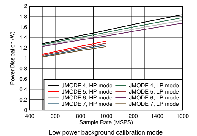
Figure 6-90. Dual Channel, Power Dissipation vs F_S and JMODE 4 - 7
