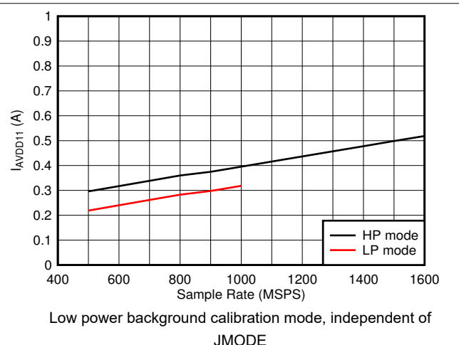
Figure 6-104. Single Channel, I_{VA11} vs F_S
