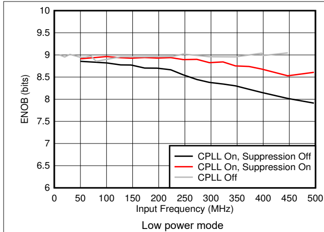
Figure 6-47. ENOB vs F_{IN} and C-PLL modes
