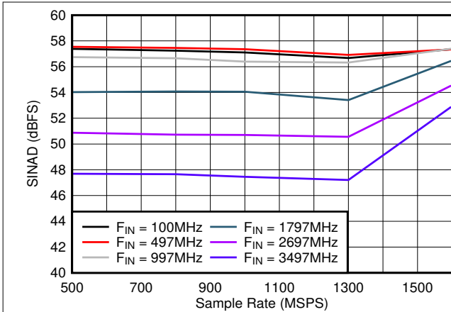
Figure 6-25. SINAD vs Sample Rate
