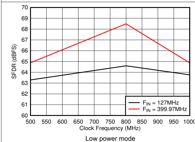
Figure 6-29. SFDR vs Sample Rate
