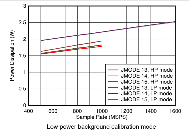
Figure 6-82. Quad Channel, Power Dissipation vs F_S and JMODE 13 - 15
