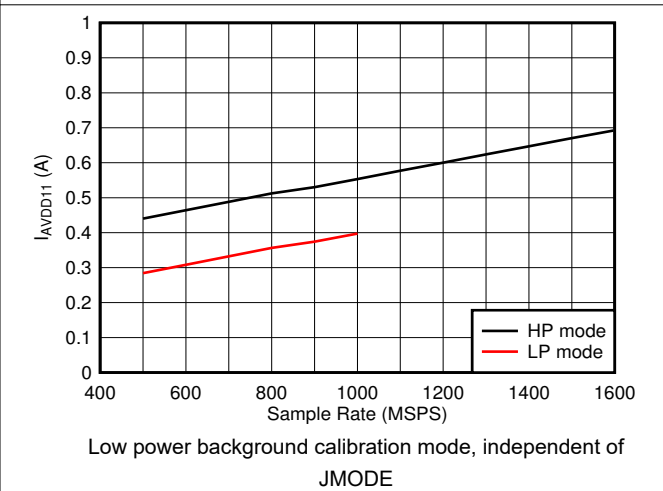
Figure 6-84. Quad Channel, I_{VA11} vs F_S
