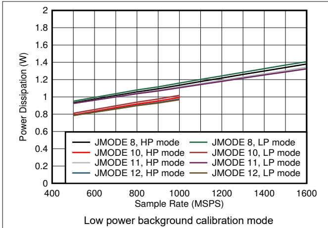
Figure 6-101. Single Channel, Power Dissipation vs F_S and JMODE 8 - 12
