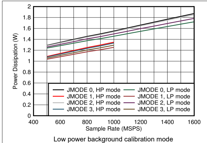
Figure 6-89. Dual Channel, Power Dissipation vs F_S and JMODE 0 - 3
