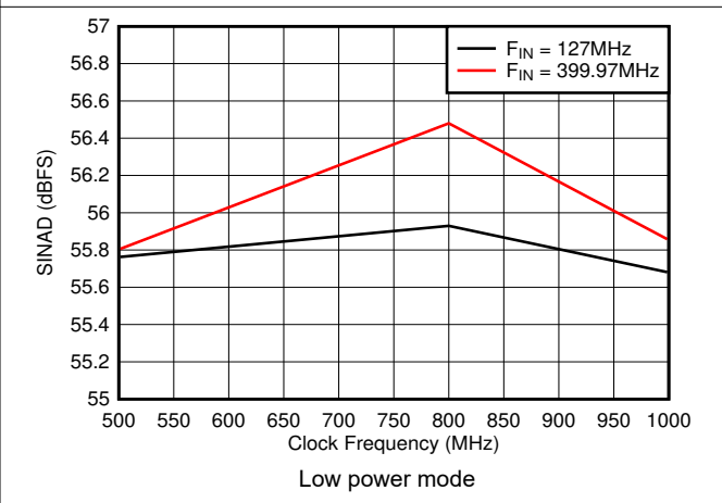
Figure 6-30. SINAD vs Sample Rate
