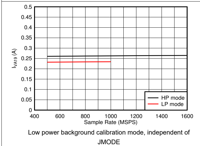
Figure 6-103. Single Channel, I_{VA19} vs F_S
