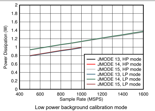
Figure 6-102. Single Channel, Power Dissipation vs F_S and JMODE 13 - 15
