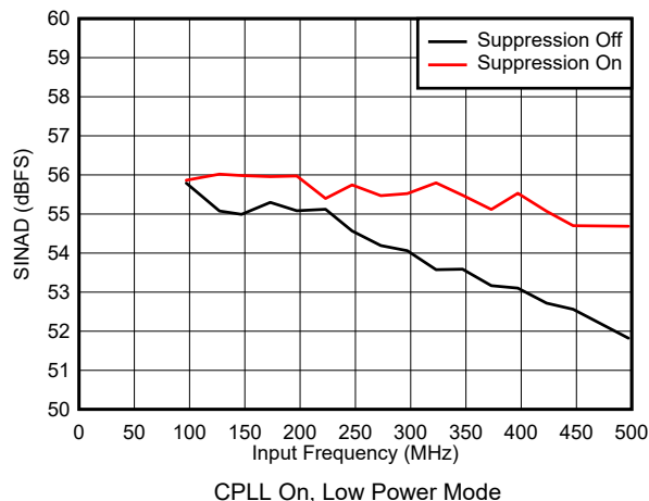
Figure 5-62. SINAD vs Input Frequency
