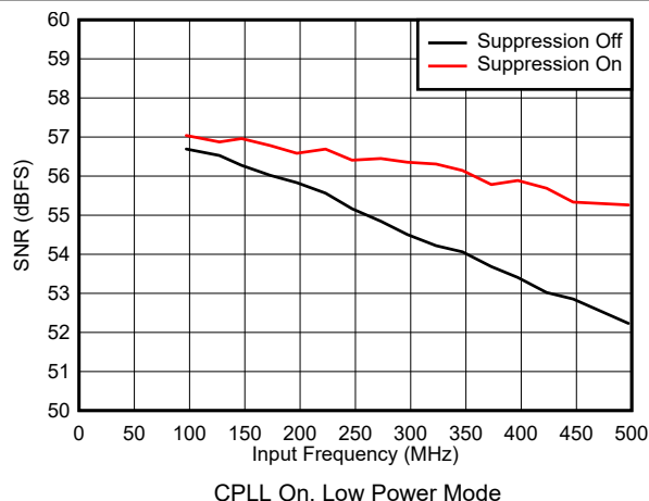
Figure 5-60. SNR vs Input Frequency
