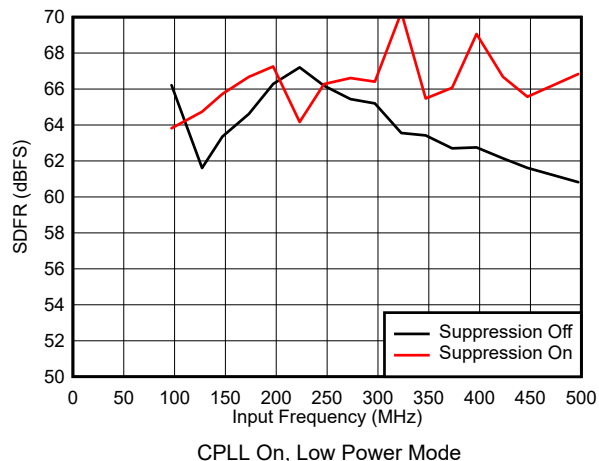
Figure 5-61. SFDR vs Input Frequency
