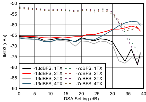
Figure 4-255. TX IMD3 vs DSA Setting at 9.61 GHz
