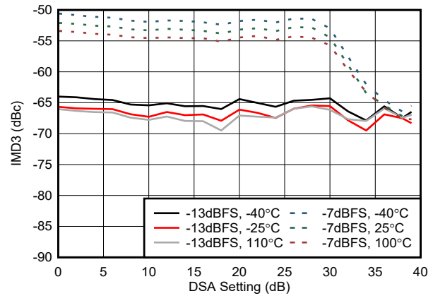
Figure 4-256. TX IMD3 vs DSA Setting at 9.61 GHz
