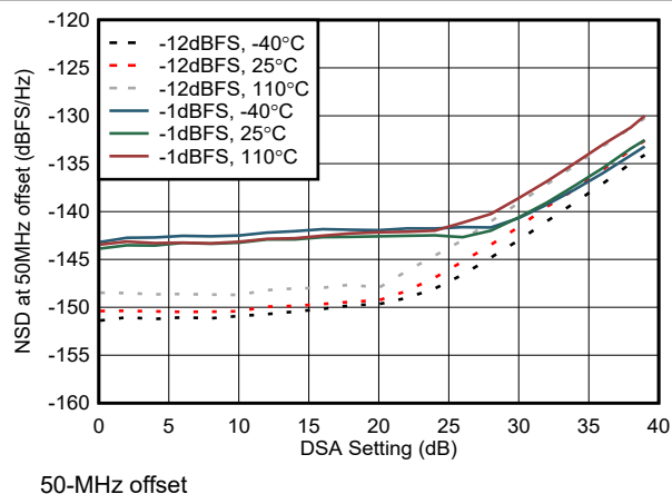
Figure 4-225. TX NSD vs DSA Setting at 8.11 GHz
