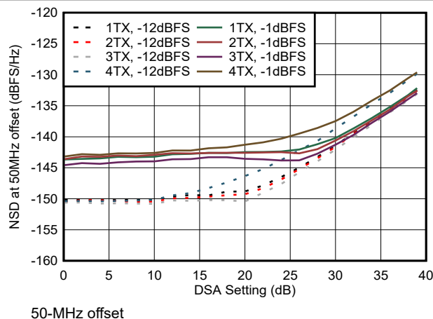
Figure 4-224. TX NSD vs DSA Setting at 8.11 GHz
