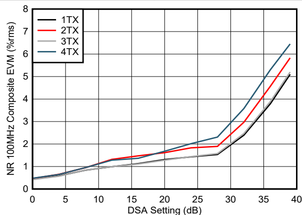
Figure 4-228. TX NR100MHz EVM vs DSA Setting 8.11 GHz
