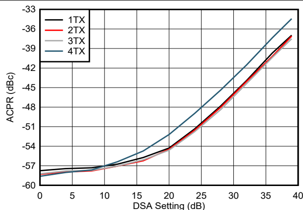
Figure 4-226. TX NR100MHz ACPR vs DSA Setting 8.11 GHz
