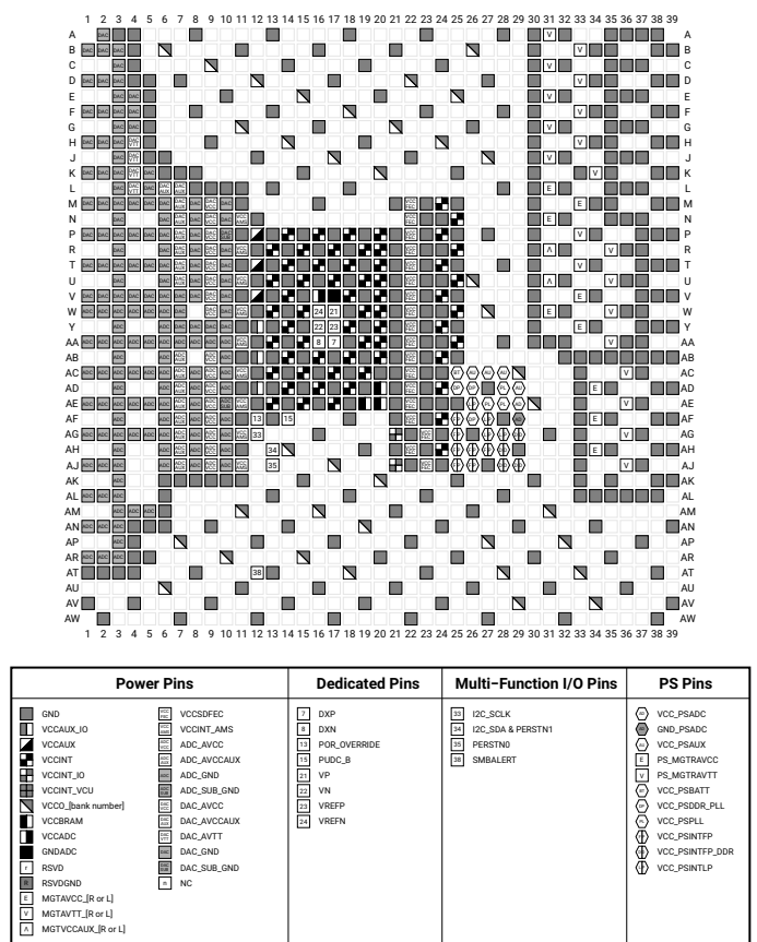
Figure 4-88: FFVG1517, FSVG1517, FSRG1517 Packages—XCZU48DR, XQZU48DR Power, Dedicated, and Multi-function Pin Diagram
