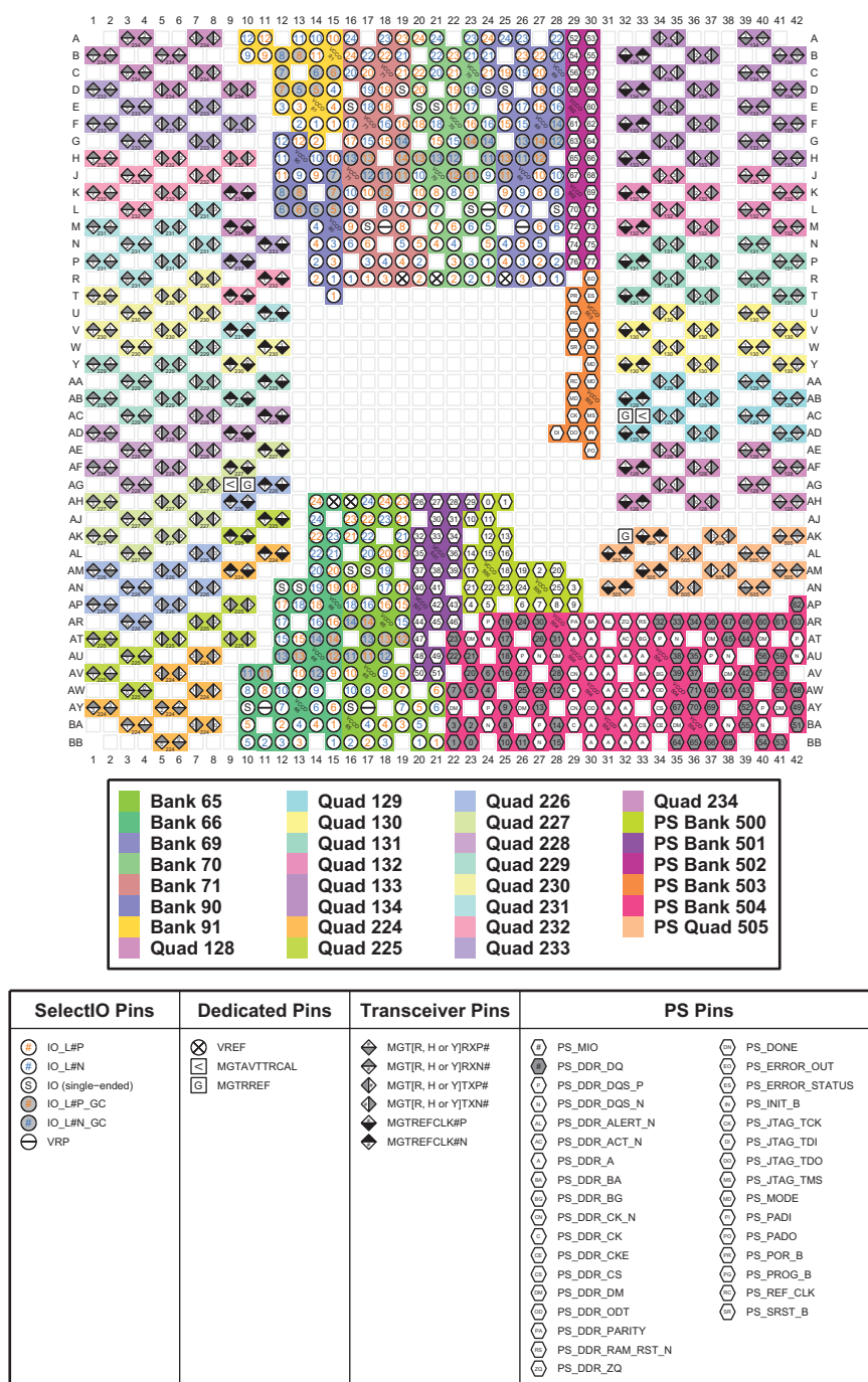
Figure 4-93: FFVD1760 Package—XCZU17EG and XCZU19EG I/O Bank Diagram
