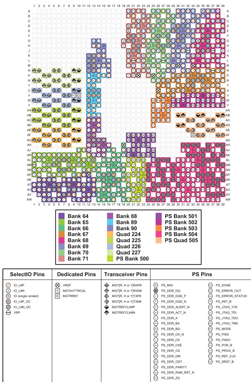
Figure 4-69: FFVB1517 Package—XCZU11EG I/O Bank Diagram
