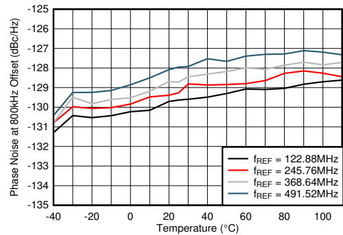
A. PLL enabled, f_{VCO} = 11796.48 MHz, measured at 2TXOUT
