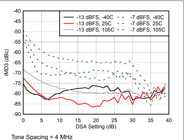
Figure 5-269. IMD3 vs DSA Setting at 400 MHz
