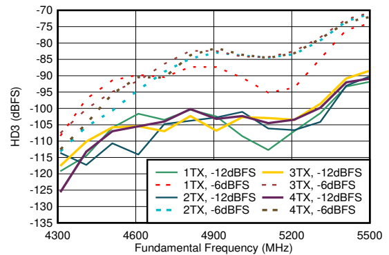
Matching at 4.9 GHz, f_{\text{DAC}} = 11.79648\text{GSPS} , interleave mode, normalized to output power at harmonic frequency Figure 5-514. TX HD3 vs Digital Amplitude and Output Frequency at 4.9 GHz
