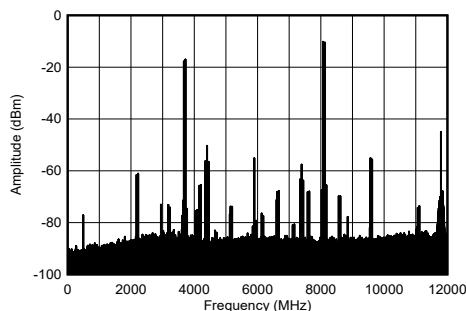
Figure 4-207. TX Single Tone Output Spectrum at 8.1 GHz
