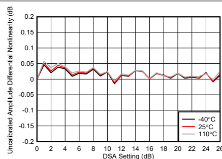
Figure 4-238. TX DSA Uncalibrated Amplitude Differential Nonlinearity
