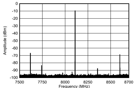
Figure 4-204. TX Single Tone Output Spectrum at 8.1 GHz
