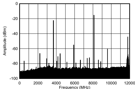
Figure 4-205. TX Single Tone Output Spectrum at 8.1 GHz
