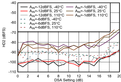
Figure 4-462. RX HD2 vs DSA Setting at 9.6 GHz
