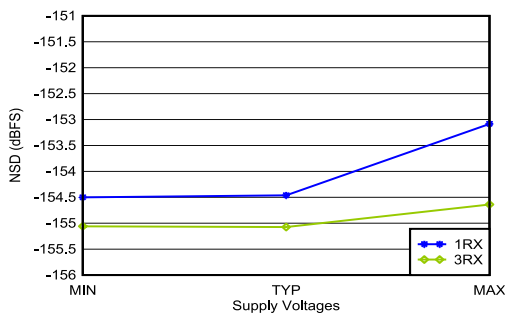
Figure 4-420. RX IMD3 vs Supply and Channel at 4.9 GHz
