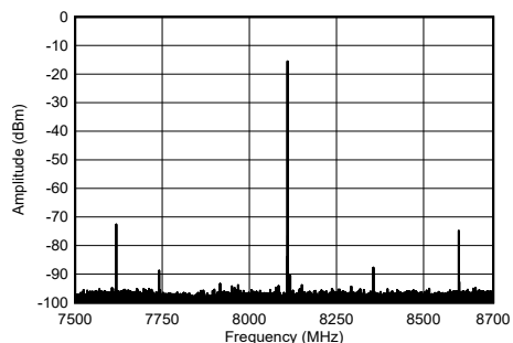
Figure 4-206. TX Single Tone Output Spectrum at 8.1 GHz
