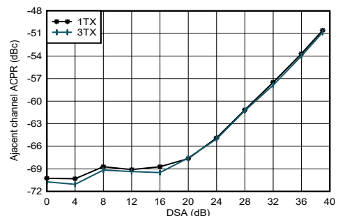
Figure 4-140. TX 20-MHz LTE ACPR vs DSA Setting at 3.5 GHz
