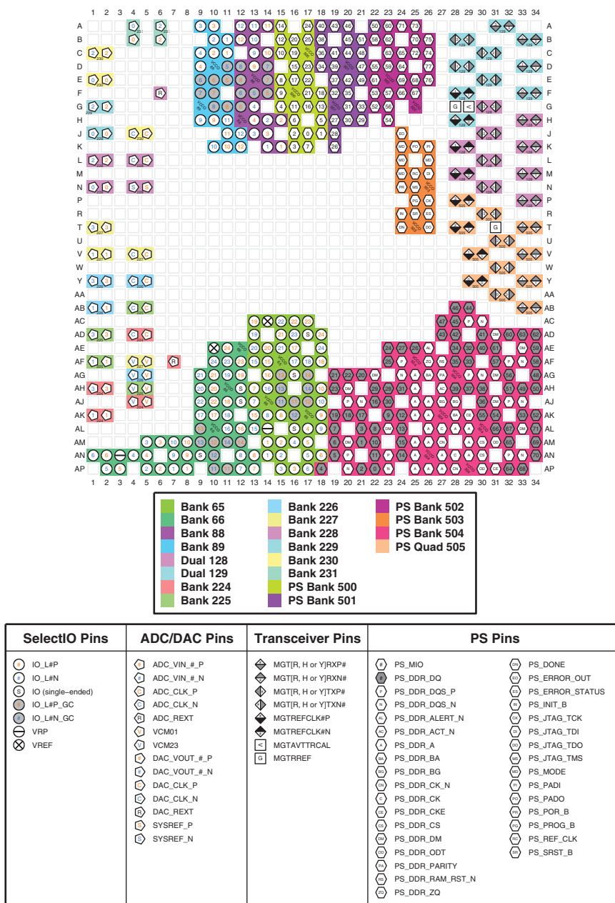
Figure 4-57: FFVE1156 and FSVE1156 Packages—XCZU47DR I/O Bank Diagram
