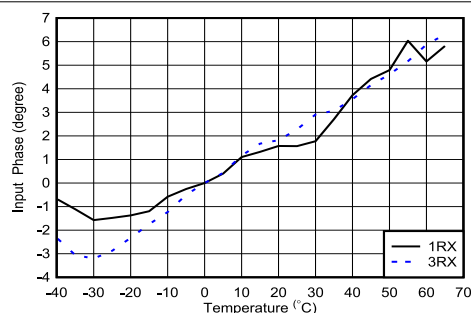
Figure 4-287. RX Input Phase vs Temperature and DSA at f_{\text{OUT}} = 0.8 \text{ GHz}
