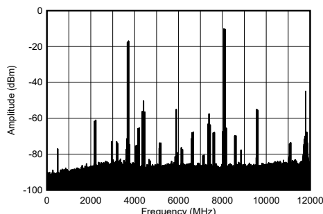
Figure 4-207. TX Single Tone Output Spectrum at 8.11 GHz
