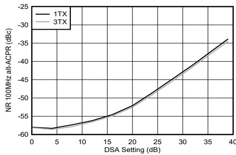
Figure 4-281. TX NR100 MHz alt-ACPR vs DSA Setting at 9.61 GHz
