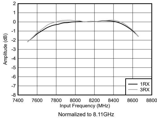
Figure 4-422. RX Amplitude vs Frequency and Channel
