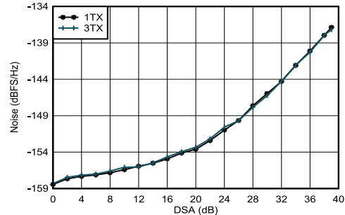
Figure 4-20. TX Output Noise vs Channel and Attenuation at 0.85 GHz
