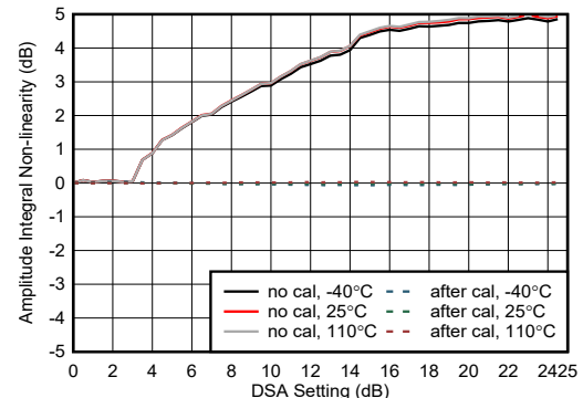
Figure 4-451. RX Amplitude Integrated Non-linearity at 9.6 GHz
