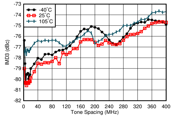
Figure 4-26. TX IMD3 vs Tone Spacing and Temperature at 0.85 GHz
