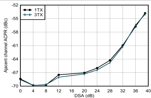
Figure 4-35. TX 20-MHz LTE ACPR vs DSA at 0.85 GHz
