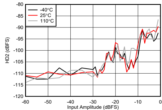
Figure 4-461. RX HD2 vs Digital Level at 9.6 GHz
