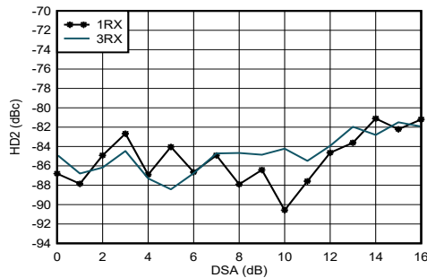
Figure 4-411. RX HD2 vs DSA Setting and Channel at 4.9 GHz
