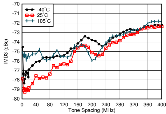
Figure 4-25. TX IMD3 vs Tone Spacing and Temperature at 0.85 GHz
