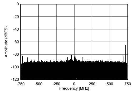
Figure 4-465. RX Single Tone Output FFT at 9.61 GHz
