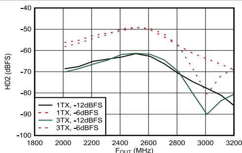
Figure 4-112. TX HD2 vs Digital Amplitude and Output Frequency at 2.6 GHz
