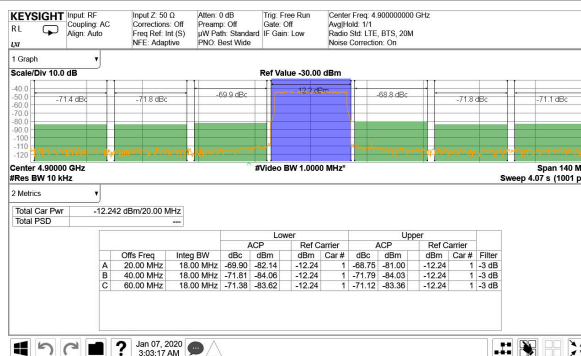
Figure 4-174. TX 20-MHz LTE Output Spectrum at 4.9 GHz
