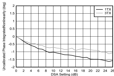
Figure 4-248. TX DSA Uncalibrated Phase Integrated Nonlinearity
