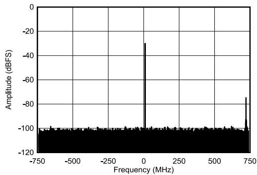
Figure 4-466. RX Single Tone Output FFT at 9.61 GHz
