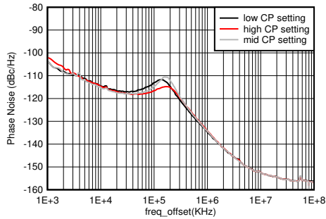
Figure 4-480. Phase Noise for 12-GHz VCO vs Offset Frequency and CP Setting at f_{OUT} = 2.6 GHz
