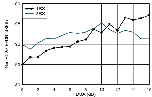
Figure 4-312. RX Non-HD2/3 vs DSA Setting at 0.8 GHz
