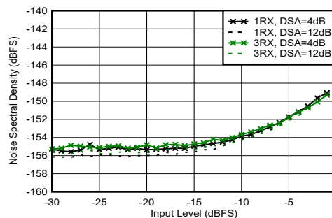
Figure 4-387. RX Noise Spectral Density vs Input Level and DSA Setting at 3.6 GHz
