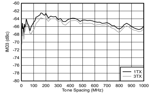
Figure 4-256. TX IMD3 vs Tone Spacing at 9.61 GHz
