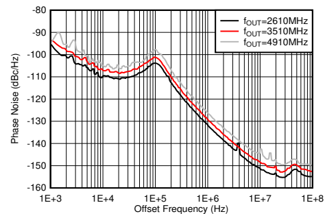
Figure 4-477. Phase Noise for 12-GHz VCO vs Offset Frequency and f_{\text{OUT}} at 25^\circ\text{C}
