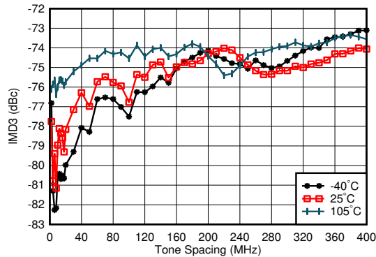
Figure 4-25. TX IMD3 vs Tone Spacing and Temperature at 0.85 GHz
