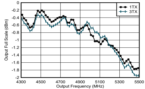
Figure 4-150. TX Full Scale vs RF Frequency and Channel at 5898.24 MSPS, Straight Mode, 2nd Nyquist Zone
