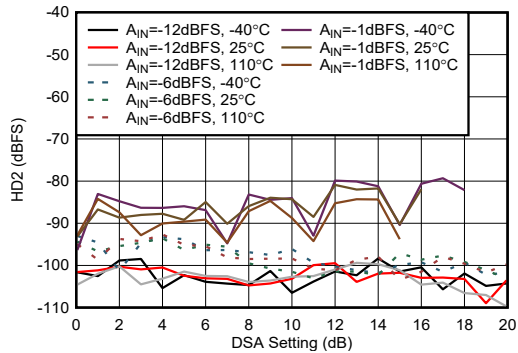
Figure 4-436. RX HD2 vs DSA Setting at 8.1GHz
