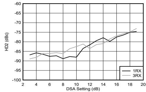
Figure 4-379. RX HD2 vs DSA Setting and Channel at 3.6 GHz
