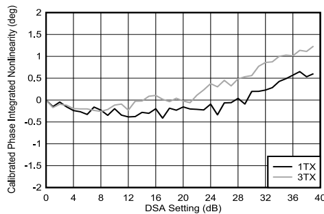
Figure 4-200. TX DSA Calibrated Phase Integrated Nonlinearity at 8.11 GHz
