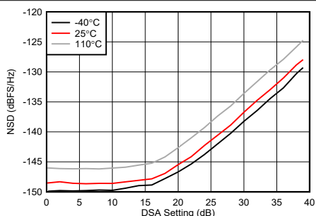
Figure 4-263. TX NSD vs DSA Setting at 9.61 GHz
