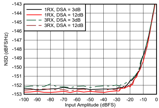
Figure 4-459. RX NSD vs Digital Amplitude at 9.6 GHz
