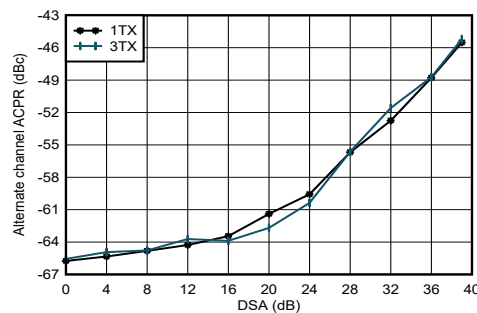
Figure 4-227. TX NR100 MHz alt-ACPR vs DSA Setting 8.1 GHz
