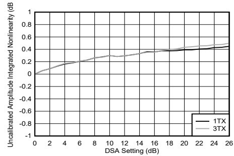
Figure 4-240. TX DSA Uncalibrated Amplitude Integrated Nonlinearity
