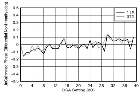
Figure 4-195. TX DSA Uncalibrated Phase Differential Nonlinearity at 8.11 GHz
