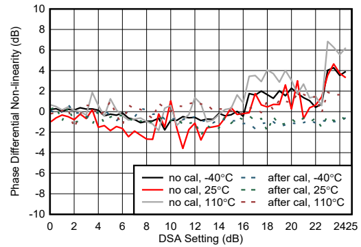
Figure 4-453. RX Phase Integrated Non-linearity at 9.6 GHz
