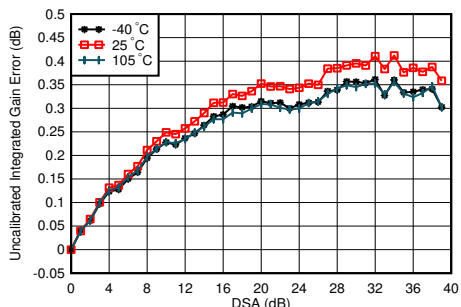
Figure 4-130. TX Uncalibrated Integrated Gain Error vs DSA Setting and Temperature at 3.5 GHz
