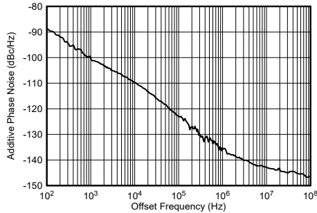
Figure 4-279. TX Additive Phase Noise vs Offset Frequency at 9.61 GHz
