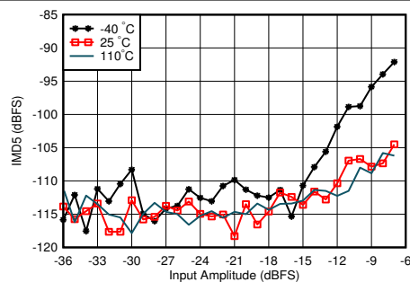
Figure 4-304. RX IMD5 vs Input Level and Temperature at 0.8 GHz
