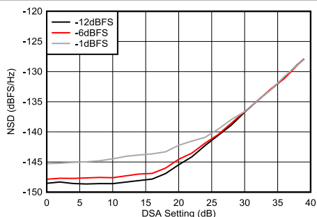
Figure 4-261. TX NSD vs DSA Setting at 9.61 GHz
