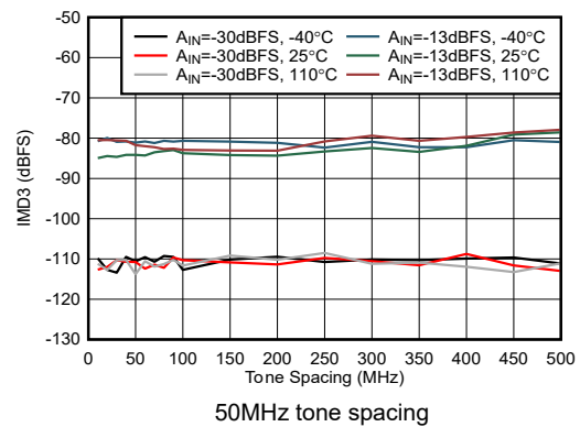
Figure 4-457. RX IMD3 vs Tone Spacing at 9.6 GHz
