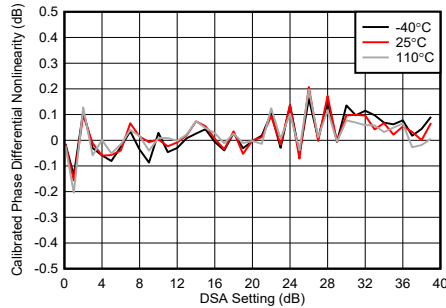
Figure 4-198. TX DSA Calibrated Phase Differential Nonlinearity at 8.11 GHz
