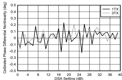
Figure 4-196. TX DSA Calibrated Phase Differential Nonlinearity at 8.11 GHz
