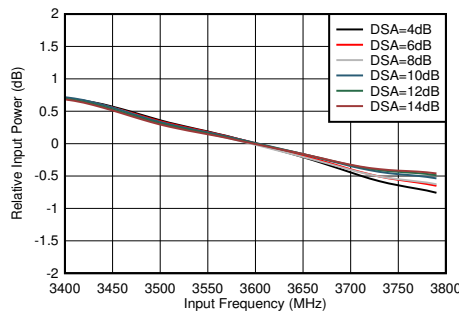
Figure 4-366. RX In-Band Gain Flatness, f_{\text{IN}} = 3600 \text{ MHz}
