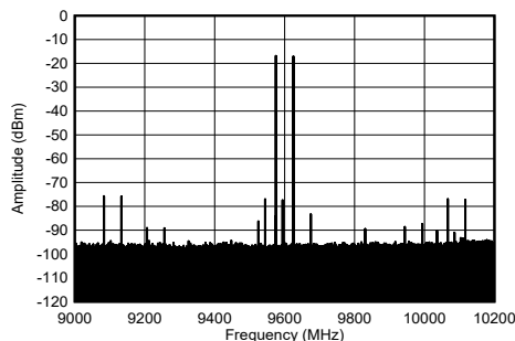
Figure 4-274. TX 2-Tone Spectrum at 9.61 GHz and -13 dBFS (1.2 GHz BW)
