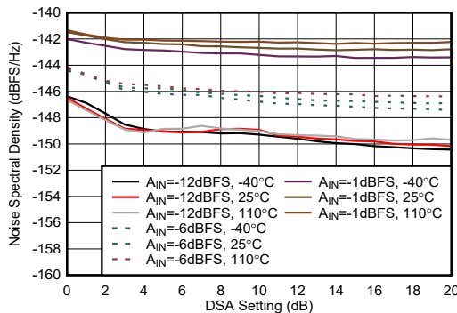
Figure 4-460. RX NSD vs DSA Setting at 9.6 GHz
