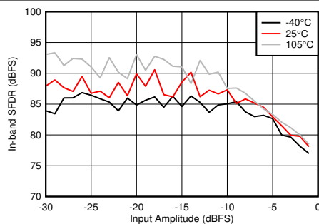
Figure 4-362. RX In-Band SFDR ( \pm 300 \text{ MHz} ) vs Input Amplitude and Temperature at 2.6 GHz
