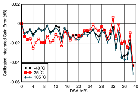
Figure 4-131. TX Calibrated Integrated Gain Error vs DSA Setting and Temperature at 3.5 GHz
