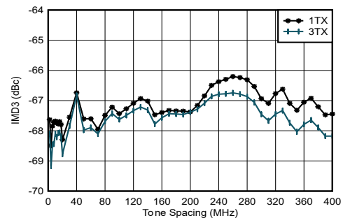
Figure 4-170. TX IMD3 vs Tone Spacing and Channel at 4.9 GHz
