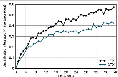
Figure 4-126. TX Uncalibrated Integrated Phase Error vs DSA Setting and Channel at 3.5 GHz
