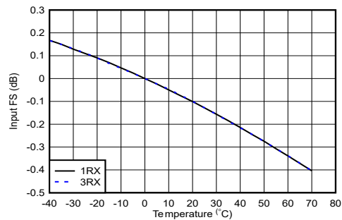
Figure 4-317. RX Input Fullscale vs Temperature and Channel at 1.75 GHz
