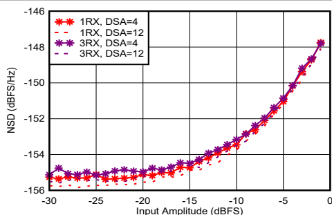
Figure 4-352. RX Noise Spectral Density vs Input Amplitude and Channel at 2.6 GHz
