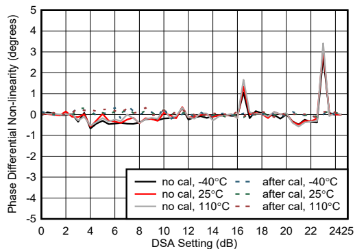
Figure 4-426. RX Phase Differential Nonlinearity at 8.1GHz
