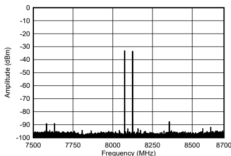
Figure 4-212. TX Dual Tone Output Spectrum at 8.11 GHz
