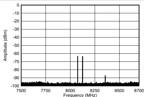
Figure 4-216. TX Dual Tone Output Spectrum at 8.11 GHz
