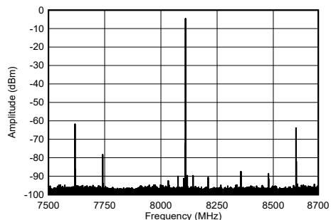
Figure 4-204. TX Single Tone Output Spectrum at 8.11 GHz
