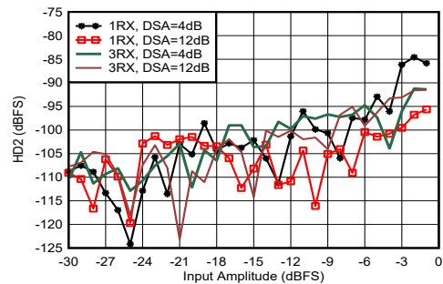
Figure 4-334. RX HD2 vs DSA Setting and Channel at 1.9 GHz
