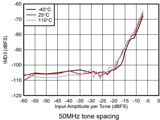
Figure 4-428. RX IMD3 vs Input Amplitude at 8.1GHz
