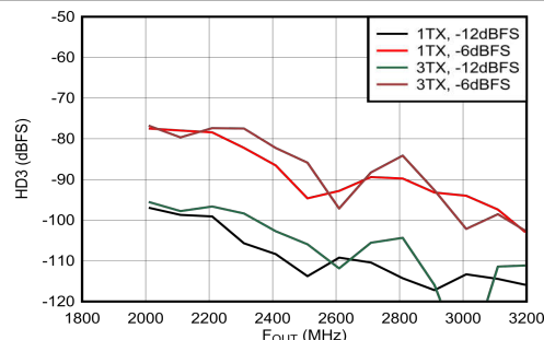
Figure 4-113. TX HD3 vs Digital Amplitude and Output Frequency at 2.6 GHz
