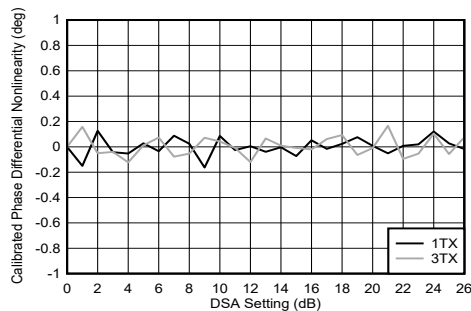
Figure 4-245. TX DSA Calibrated Phase Differential Nonlinearity
