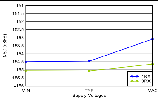
Figure 4-420. RX IMD3 vs Supply and Channel at 4.9 GHz
