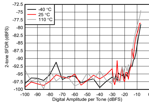
Figure 4-439. RX 2-tone SFDR vs Digital Amplitude at 8.1GHz
