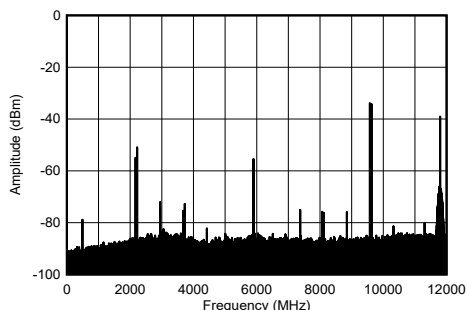
Figure 4-273. TX 2-Tone Spectrum at 9.61 GHz and -13 dBFS (wideband)
