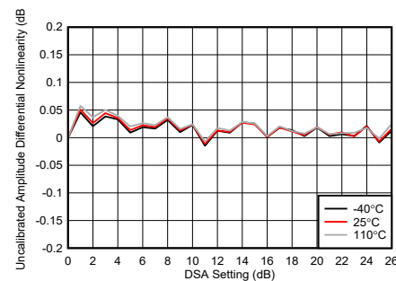
Figure 4-238. TX DSA Uncalibrated Amplitude Differential Nonlinearity
