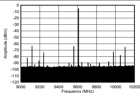
Figure 4-264. TX 2-tone SFDR vs Digital Amplitude at 9.61 GHz
