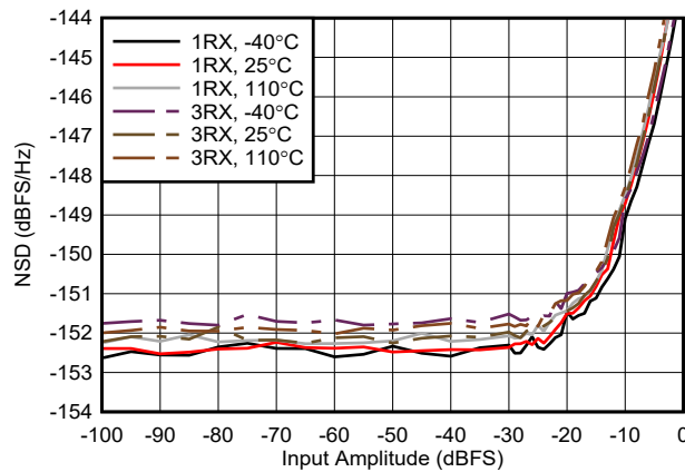
Figure 4-458. RX NSD vs Digital Amplitude at 9.6 GHz
