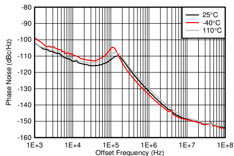
Figure 4-504. Phase Noise for 8-GHz VCO vs Offset Frequency and Temperature at f_{OUT} = 1910 MHz
