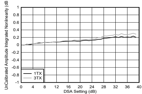
Figure 4-191. TX DSA Uncalibrated Amplitude Integrated Nonlinearity at 8.11 GHz
