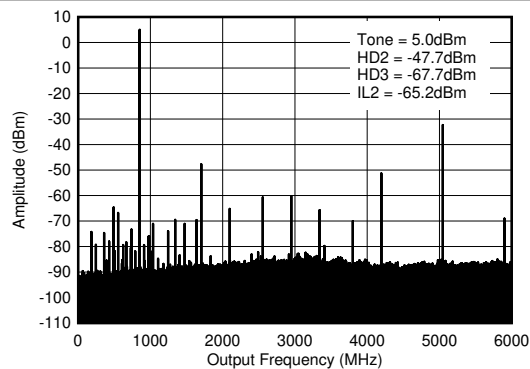
Figure 4-43. TX Single Tone (-1 dBFS) Output Spectrum at 0.85 GHz ( 0-f_{\text{DAC}} )
