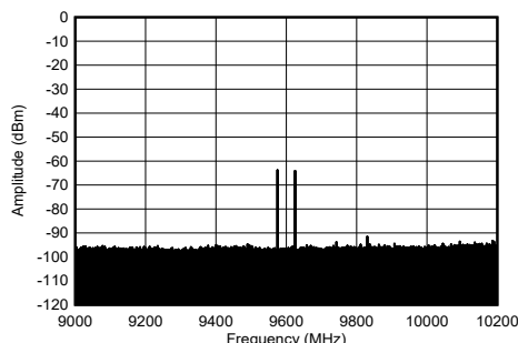
Figure 4-276. TX 2-Tone Spectrum at 9.61 GHz and -30 dBFS Each (1.2 GHz BW)
