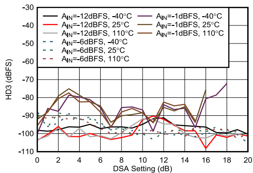
Figure 4-438. RX HD3 vs DSA Setting at 8.1GHz
