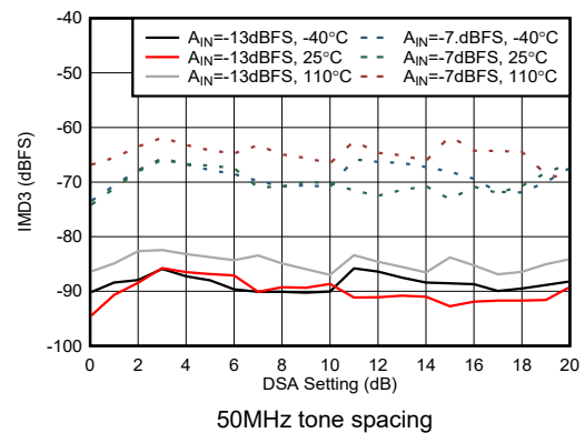
Figure 4-455. RX IMD3 vs DSA Setting at 9.6 GHz
