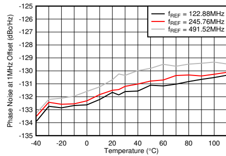
Figure 4-495. Phase Noise for 10-GHz VCO at 1 MHz vs Temperature and f_{REF} at f_{OUT} = 2.6 GHz
