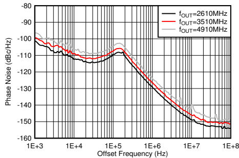
Figure 4-500. Phase Noise for 9-GHz VCO vs Offset Frequency and f_{OUT} at 25°C
