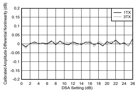
Figure 4-237. TX DSA Calibrated Amplitude Differential Nonlinearity
