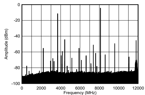
Figure 4-203. TX Single Tone Output Spectrum at 8.11 GHz
