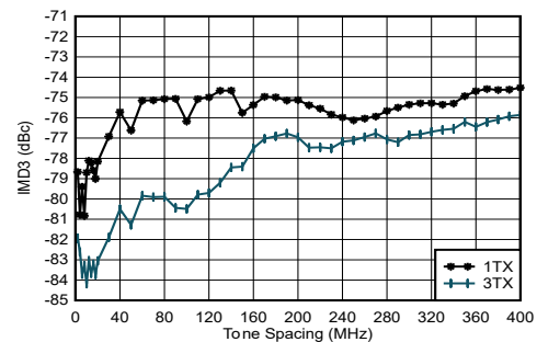
Figure 4-22. TX IMD3 vs Tone Spacing and Channel at 0.85 GHz
