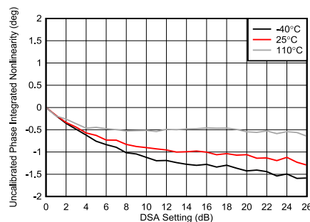
Figure 4-250. TX DSA Uncalibrated Phase Integrated Nonlinearity
