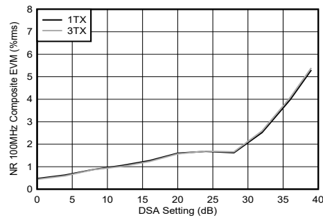
Figure 4-282. TX NR100 MHz EVM vs DSA Setting at 9.61 GHz
