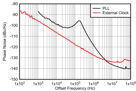
Figure 4-474. Phase Noise vs Offset Frequency for PLL and External Clock at 12 GHz
