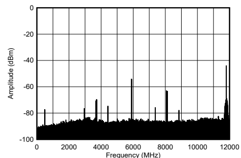
Figure 4-213. TX Dual Tone Output Spectrum at 8.11 GHz
