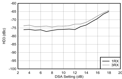
Figure 4-358. RX HD3 vs DSA Setting and Channel at 2.6 GHz
