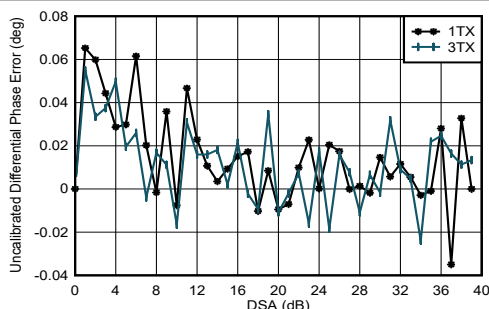
Figure 4-124. TX Uncalibrated Differential Phase Error vs DSA Setting and Channel at 3.5 GHz
