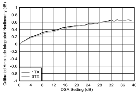
Figure 4-192. TX DSA Calibrated Amplitude Integrated Nonlinearity at 8.11 GHz
