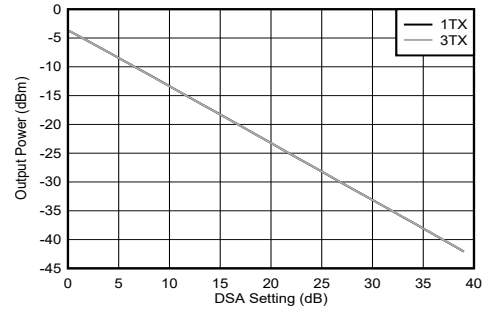
Figure 4-185. TX Output Power vs DSA Setting at 8.11 GHz
