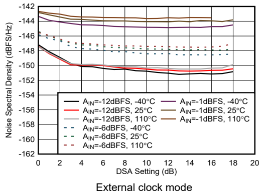
Figure 4-434. RX NSD vs DSA Setting at 8.1GHz
