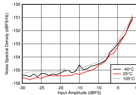
Figure 4-351. RX Noise Spectral Density vs Input Amplitude and Temperature at 2.6 GHz
