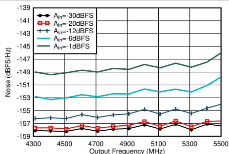
Figure 4-173. TX Single Tone Output Noise vs Frequency and Amplitude at 4.9 GHz
