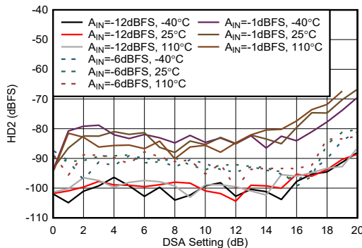
Figure 4-462. RX HD2 vs DSA Setting at 9.6 GHz
