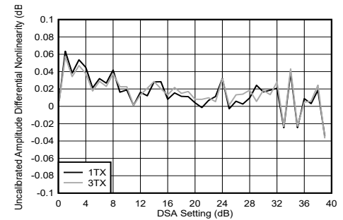
Figure 4-187. TX DSA Uncalibrated Amplitude Differential Nonlinearity at 8.11 GHz
