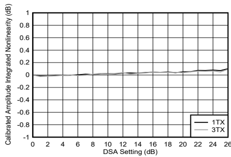
Figure 4-241. TX DSA Calibrated Amplitude Integrated Nonlinearity
