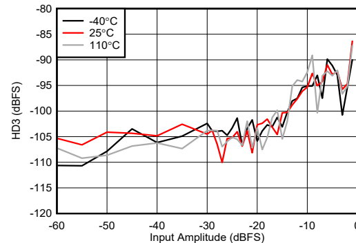
Figure 4-437. RX HD3 vs Digital Amplitude at 8.1GHz
