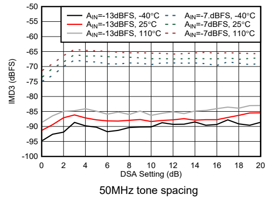
Figure 4-429. RX IMD3 vs DSA Setting at 8.1GHz
