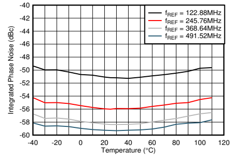
Figure 4-481. Integrated Phase Noise for 12-GHz VCO vs Temperature and f_{REF} at f_{OUT} = 2.6 GHz
