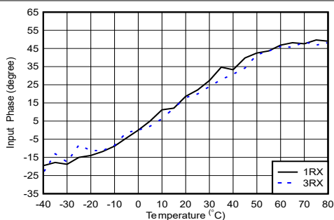
Figure 4-395. RX Input Phase vs Temperature and DSA at f_{\text{OUT}} = 4.9 \text{ GHz}
