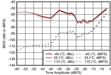
Figure 4-253. TX IMD3 vs Digital Amplitude at 9.61 GHz
