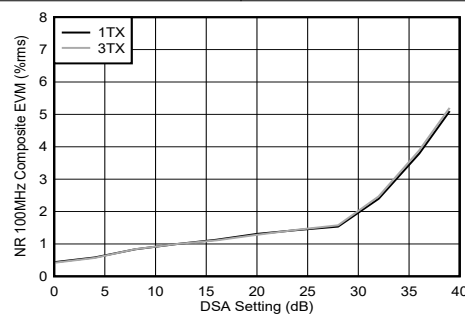
Figure 4-228. TX NR100 MHz EVM vs DSA Setting 8.1 GHz
