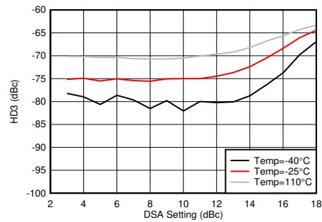
Figure 4-359. RX HD3 vs DSA Setting and Temperature at 2.6 GHz
