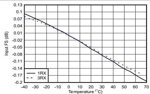
Figure 4-286. RX Input Fullscale vs Temperature and Channel at 800 MHz
