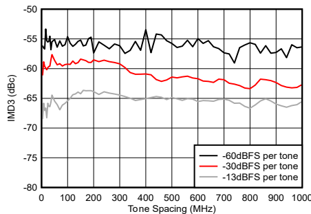
Figure 4-257. TX IMD3 vs Tone Spacing at 9.61 GHz
