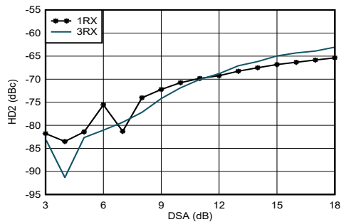
Figure 4-305. RX HD2 vs DSA Setting and Channel at 0.8 GHz
