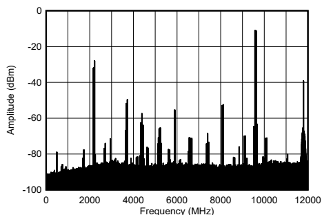
Figure 4-269. TX Single Tone Spectrum at 9.61 GHz and -12 dBFS (wideband)
