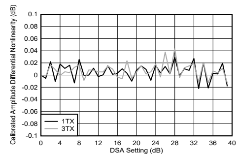
Figure 4-188. TX DSA Calibrated Amplitude Differential Nonlinearity at 8.11 GHz
