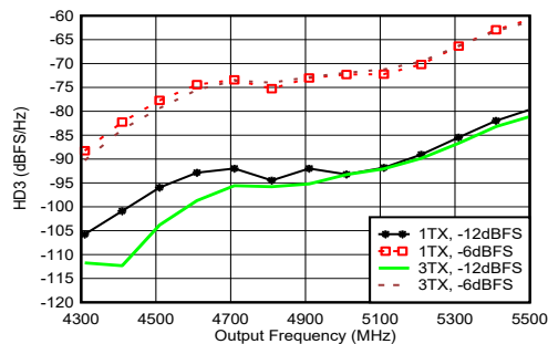
Figure 4-180. TX HD3 vs Digital Amplitude and Output Frequency at 4.9 GHz
