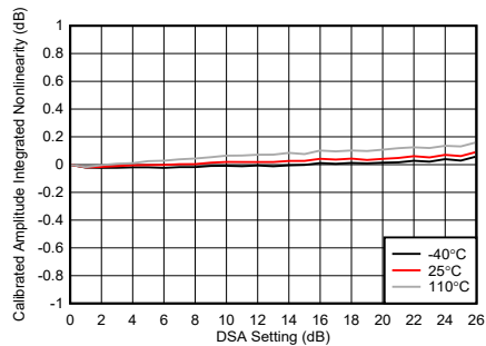
Figure 4-243. TX DSA Calibrated Amplitude Integrated Nonlinearity
