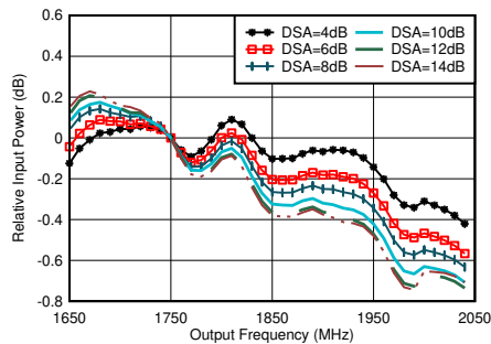
Figure 4-316. RX In-Band Gain Flatness, f_{\text{IN}} = 1750 \text{ MHz}
