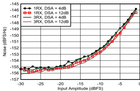
Figure 4-407. RX Noise Spectral Density vs Input Amplitude and Channel at 4.9 GHz
