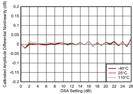
Figure 4-239. TX DSA Calibrated Amplitude Differential Nonlinearity
