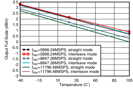
Figure 4-45. TX Output Power vs Temperature at 1.8 GHz
