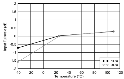
Figure 4-347. RX Input Fullscale vs Temperature and Channel at 2.6 GHz
