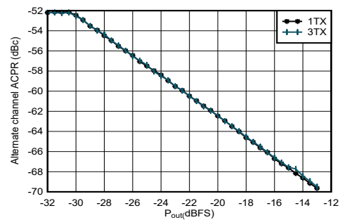
Figure 4-34. TX 20-MHz LTE alt-ACPR vs Digital Level at 0.85 GHz
