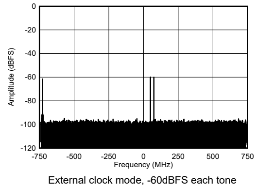
Figure 4-447. RX Dual Tone Output FFT at 8.11GHz
