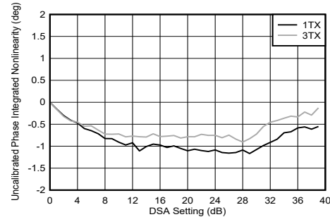
Figure 4-199. TX DSA Uncalibrated Phase Integrated Nonlinearity at 8.11 GHz
