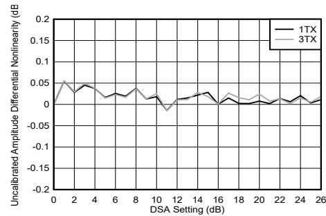
Figure 4-236. TX DSA Uncalibrated Amplitude Differential Nonlinearity
