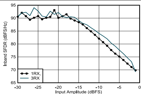
Figure 4-342. RX In-Band SFDR ( \pm 400\text{ MHz} ) vs Input Amplitude at 1.75 GHz
