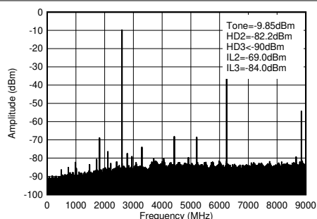
Figure 4-112. TX HD2 vs Digital Amplitude and Output Frequency at 2.6 GHz
