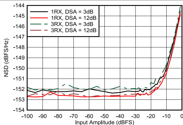
Figure 4-432. RX NSD vs Digital Amplitude at 8.1GHz
