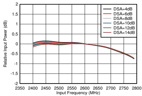
Figure 4-346. RX Inband Gain Flatness, f_{\text{IN}} = 2600 \text{ MHz}
