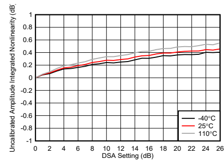
Figure 4-242. TX DSA Uncalibrated Amplitude Integrated Nonlinearity
