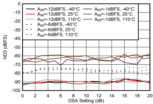
Figure 4-464. RX HD3 vs DSA Setting at 9.6 GHz
