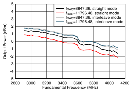
Figure 4-118. TX Output Power vs Frequency
