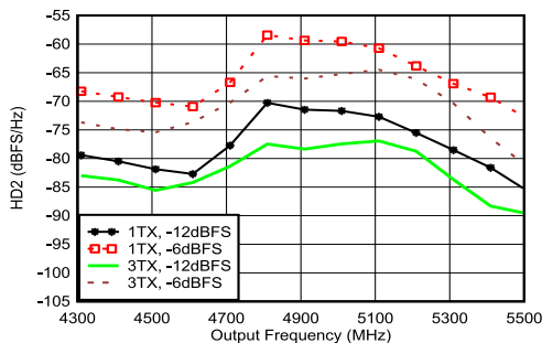
Figure 4-179. TX HD2 vs Digital Amplitude and Output Frequency at 4.9 GHz
