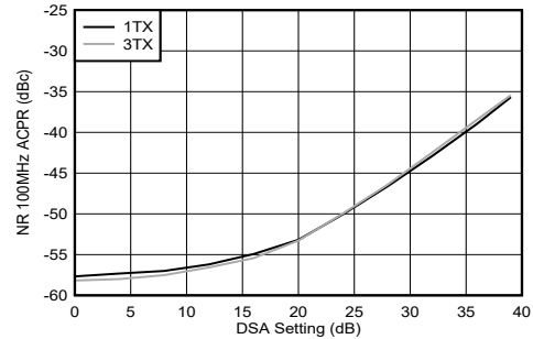
Figure 4-280. TX NR100 MHz ACPR vs DSA Setting at 9.61 GHz
