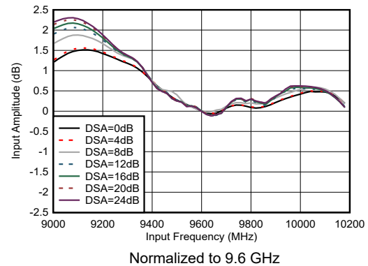
Figure 4-449. RX Input Amplitude vs Frequency at 9.6 GHz
