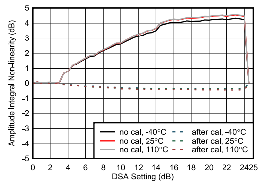
Figure 4-425. RX Amplitude Integrated Nonlinearity at 8.1GHz
