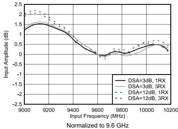
Figure 4-448. RX Input Amplitude vs Frequency
