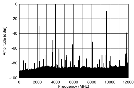
Figure 4-267. TX Single Tone Spectrum at 9.61 GHz and -6 dBFS (wideband)
