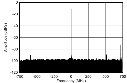
Figure 4-465. RX Single Tone Output FFT at 9.61 GHz
