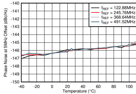
Figure 4-486. Phase Noise for 12-GHz VCO at 5-MHz Offset vs Temperature and f_{REF} at f_{OUT} = 2.6 GHz
