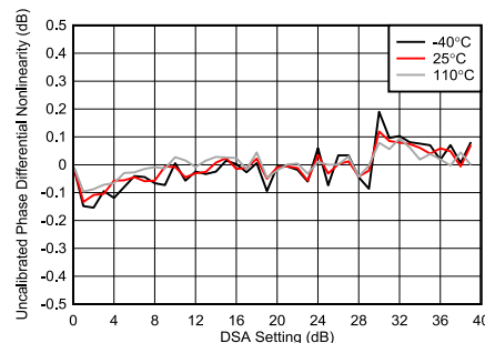
Figure 4-197. TX DSA Uncalibrated Phase Differential Nonlinearity at 8.11 GHz
