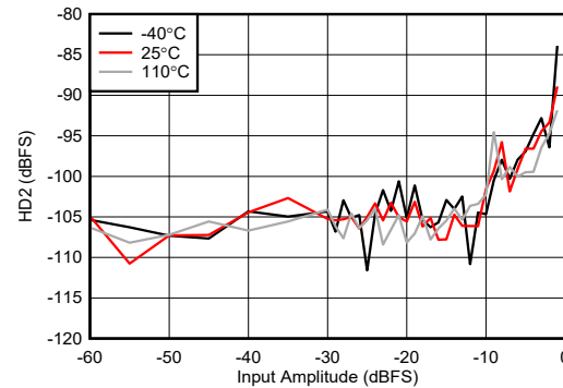
Figure 4-435. RX HD2 vs Digital Amplitude at 8.1GHz
