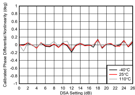
Figure 4-247. TX DSA Calibrated Phase Differential Nonlinearity
