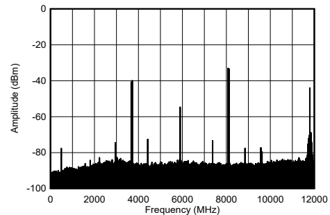
Figure 4-211. TX Dual Tone Output Spectrum at 8.11 GHz
