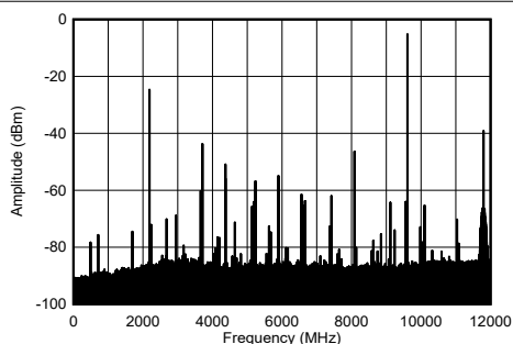
Figure 4-265. TX Single Tone Spectrum at 9.61 GHz and -1 dBFS (wideband)
