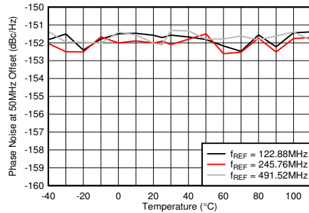
Figure 4-498. Phase Noise for 10-GHz VCO at 50 MHz vs Temperature and f_{REF} at f_{OUT} = 2.6 GHz
