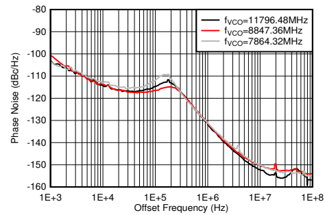
Figure 4-475. Phase Noise vs Offset Frequency and f_{\text{VCO}} at f_{\text{OUT}} = 2610 \text{ MHz}
