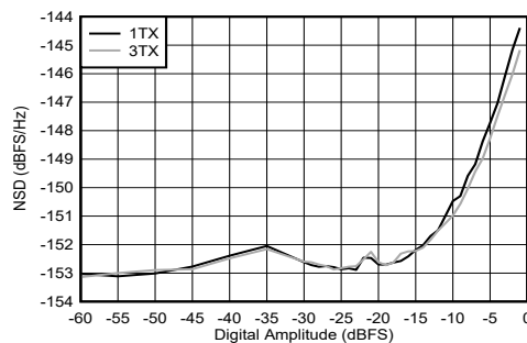
Figure 4-259. TX NSD vs Digital Amplitude at 9.61 GHz
