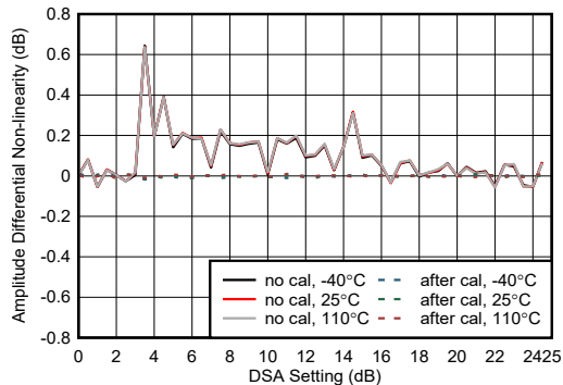
Figure 4-450. RX Amplitude Differential Non-Linearity at 9.6 GHz
