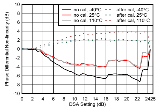
Figure 4-427. RX Phase Differential Nonlinearity at 8.1GHz
