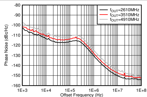
Figure 4-489. Phase Noise for 10-GHz VCO vs Offset Frequency and f_{OUT} at 25°C
