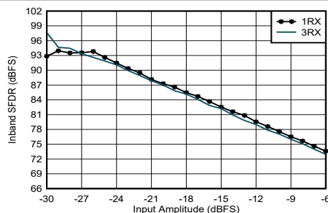
Figure 4-418. RX In-Band SFDR ( \pm 400\text{ MHz} ) vs Input Amplitude and Channel at 4.9 GHz
