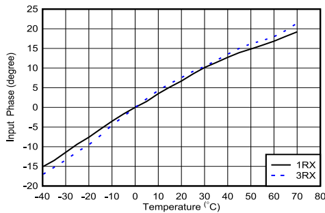
Figure 4-318. RX Input Phase vs Temperature and DSA at f_{\text{IN}} = 1.75 \text{ GHz}
