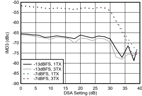
Figure 4-254. TX IMD3 vs DSA Setting at 9.61 GHz
