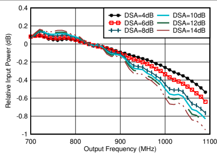
Figure 4-285. RX In-Band Gain Flatness for Channel 1RX, f_{\text{IN}} = 830 MHz
