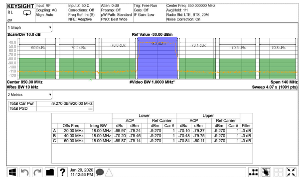
Figure 4-32. TX 20-MHz LTE Output Spectrum at 0.85 GHz
