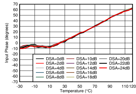
Figure 4-367. RX Input Phase vs Temperature at 3.6 GHz
