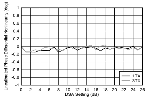
Figure 4-244. TX DSA Uncalibrated Phase Differential Nonlinearity
