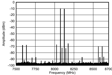
Figure 4-210. TX Dual Tone Output Spectrum at 8.11 GHz
