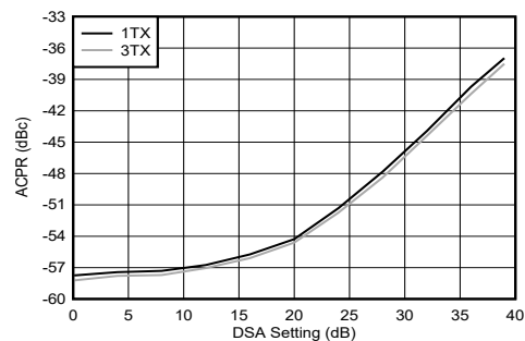
Figure 4-226. TX NR100MHz ACPR vs DSA Setting 8.1 GHz
