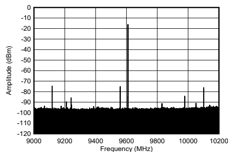
Figure 4-268. TX Single Tone Spectrum at 9.61 GHz and -6 dBFS (1.2 GHz BW)
