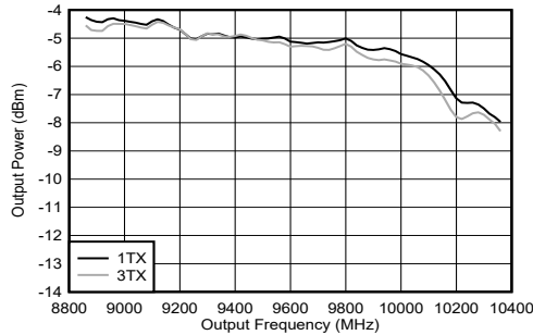
Figure 4-233. TX Output Power vs Frequency at 9.61 GHz
