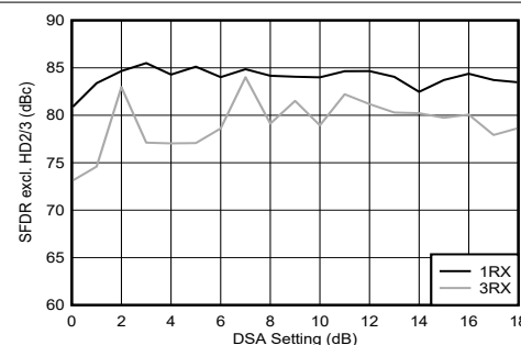
Figure 4-389. RX SFDR Excluding HD2/3 vs DSA Setting and Channel at 3.6 GHz
