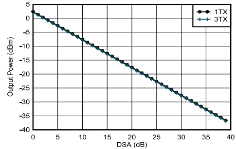
Figure 4-79. TX Output Power vs DSA Setting and Channel at 2.6 GHz
