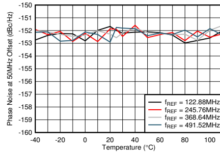
Figure 4-487. Phase Noise for 12-GHz VCO at 50-MHz Offset vs Temperature and f_{REF} at f_{OUT} = 2.6 GHz
