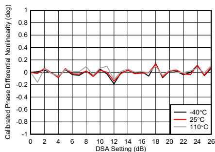
Figure 4-249. TX DSA Calibrated Phase Integrated Nonlinearity
