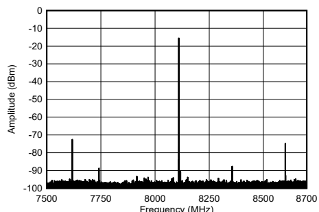
Figure 4-206. TX Single Tone Output Spectrum at 8.11 GHz
