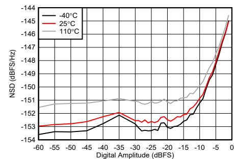
Figure 4-260. TX NSD vs Digital Amplitude at 9.61 GHz
