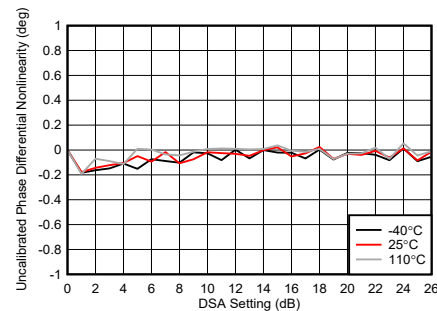
Figure 4-246. TX DSA Uncalibrated Phase Differential Nonlinearity
