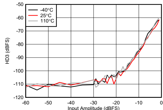
Figure 4-463. RX HD3 vs Digital Level at 9.6 GHz
