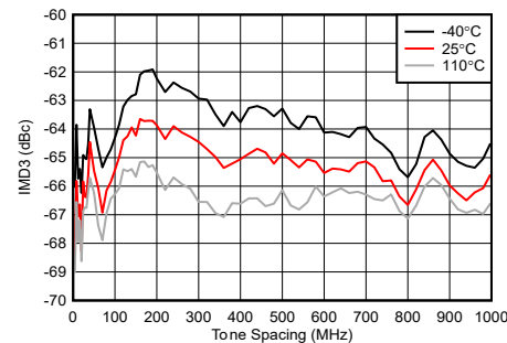
Figure 4-258. TX IMD3 vs Tone Spacing at 9.6 1GHz
