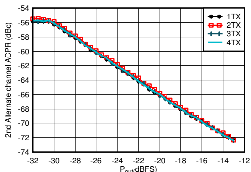
Figure 5-365. TX 20-MHz LTE ACPR vs Digital Level at 1.8425 GHz
