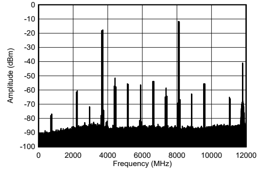
Figure 5-209. TX Dual Tone Output Spectrum at 8.11 GHz
