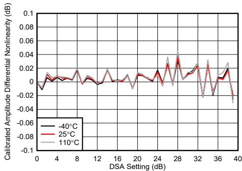
Figure 5-190. TX DSA Calibrated Amplitude Differential Nonlinearity at 8.1 GHz
