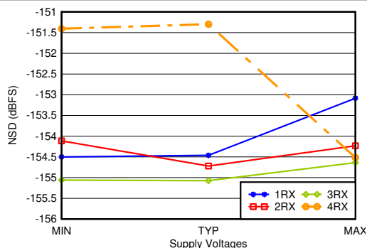
Figure 5-414. RX Noise Spectral Density vs Supply and Channel at 4.9 GHz
