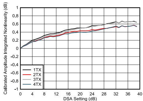
Figure 5-192. TX DSA Calibrated Amplitude Integrated Nonlinearity at 8.1 GHz
