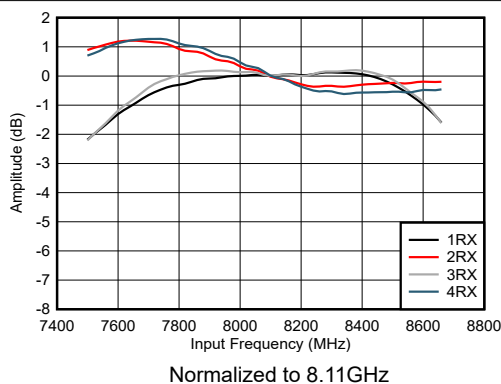
Figure 5-415. RX Amplitude vs Frequency and Channel
