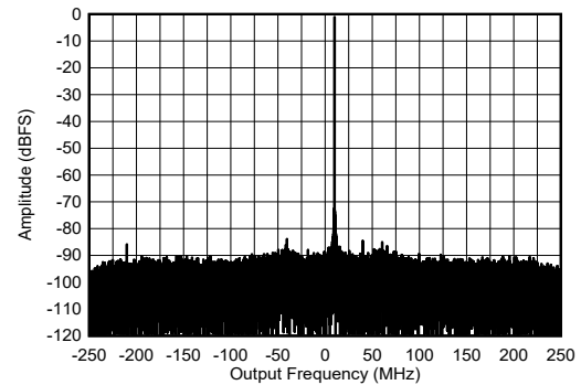
Figure 5-461. RX Single Tone Output FFT at 9.6 GHz
