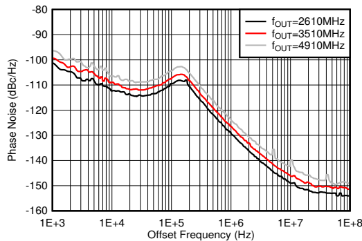
Figure 5-498. Phase Noise for 9-GHz VCO vs Offset Frequency and f_{OUT} at 25°C
