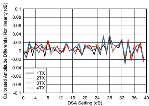
Figure 5-188. TX DSA Calibrated Amplitude Differential Nonlinearity at 8.11 GHz
