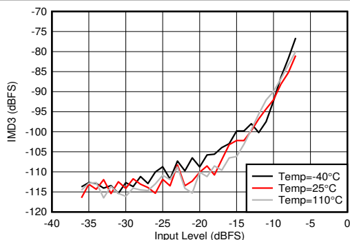
Figure 5-347. RX IMD3 vs Input Level and Temperature at 2.6 GHz
