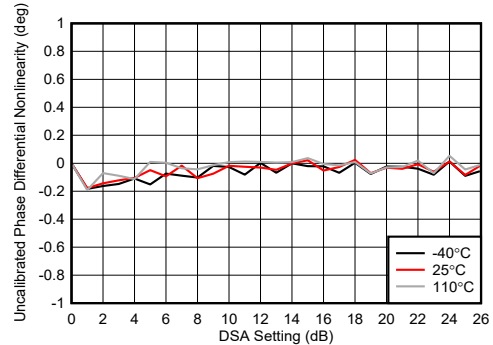
Figure 5-242. TX DSA Uncalibrated Phase Differential Nonlinearity
