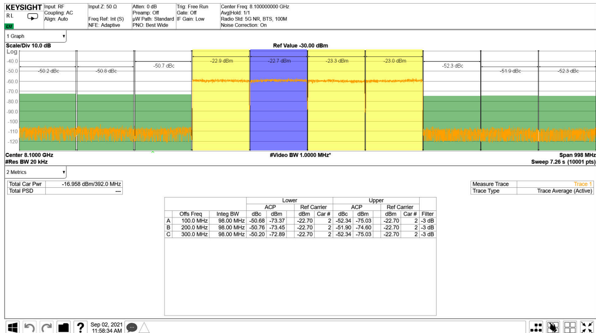
Figure 5-227. TX 4x100 MHz NR Output Spectrum 8.11 GHz
