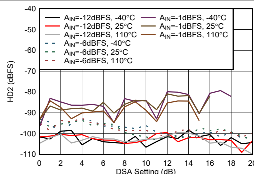
Figure 5-430. RX HD2 vs DSA Setting at 8.1 GHz
