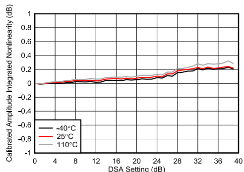
Figure 5-194. TX DSA Calibrated Amplitude Integrated Nonlinearity at 8.1 GHz
