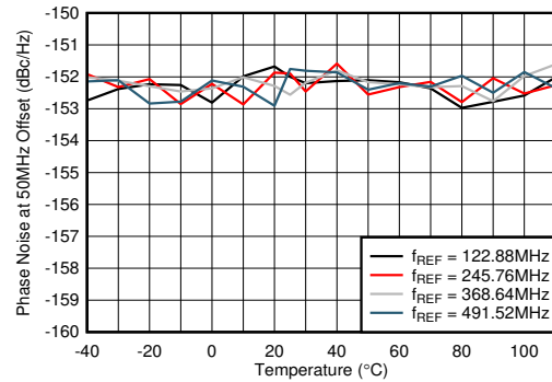
Figure 5-485. Phase Noise for 12-GHz VCO at 50-MHz Offset vs Temperature and f_{REF} at f_{OUT} = 2.6 GHz
