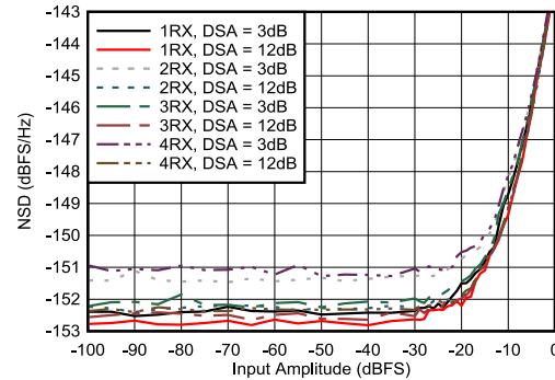
Figure 5-455. RX NSD vs Digital Amplitude at 9.6 GHz
