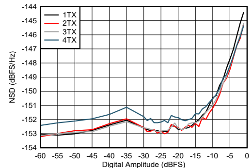
Figure 5-256. TX NSD vs Digital Amplitude at 9.61 GHz
