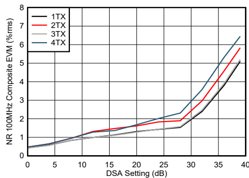
Figure 5-224. TX NR100MHz EVM vs DSA Setting 8.11 GHz
