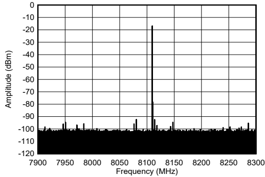
Figure 5-208. TX Single Tone Output Spectrum at 8.11 GHz
