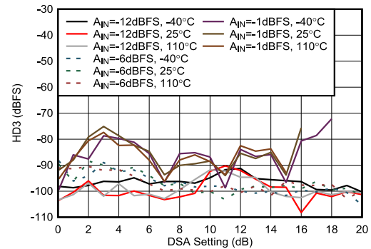
Figure 5-432. RX HD3 vs DSA Setting at 8.11 GHz
