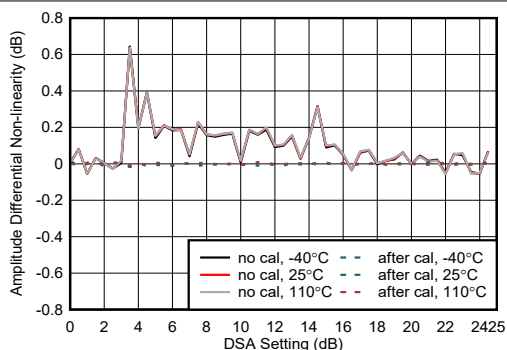
Figure 5-446. RX Amplitude Differential Non-linearity at 9.6 GHz
