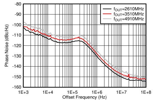
Figure 5-487. Phase Noise for 10-GHz VCO vs Offset Frequency and f_{OUT} at 25°C
