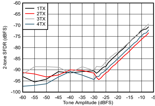
Figure 5-261. TX 2-tone SFDR vs Digital Amplitude at 9.61 GHz
