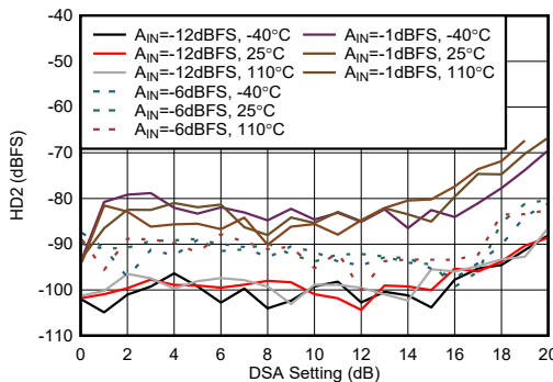
Figure 5-458. RX HD2 vs DSA Setting at 9.6 GHz
