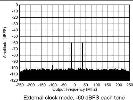
Figure 5-443. RX Dual Tone Output FFT at 8.11 GHz
