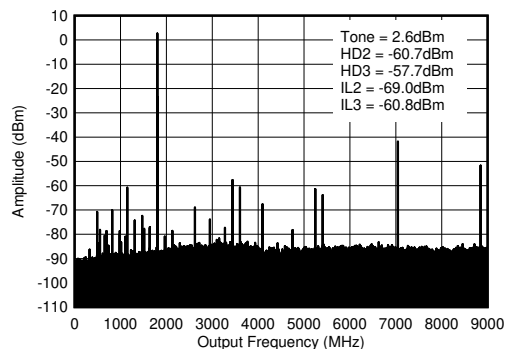
Figure 5-75. TX Single Tone (-12 dBFS) Output Spectrum at 1.8 GHz ( 0-f_{\text{DAC}} )
