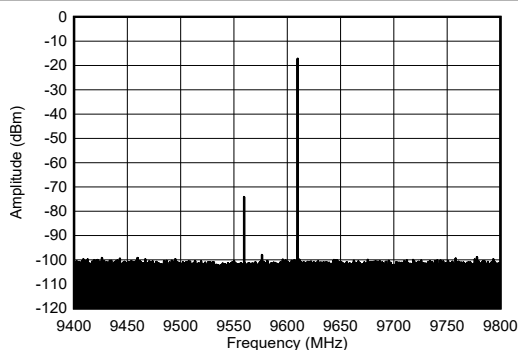
Figure 5-267. TX Single Tone Spectrum at 9.61 GHz and -12 dBFS (400 MHz BW)
