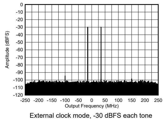
Figure 5-442. RX Dual Tone Output FFT at 8.11 GHz
