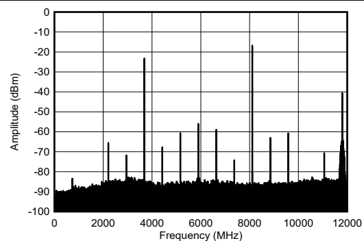
Figure 5-205. TX Single Tone Output Spectrum at 8.11 GHz
