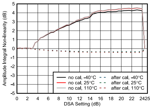
Figure 5-419. RX Amplitude Integrated Nonlinearity at 8.11 GHz
