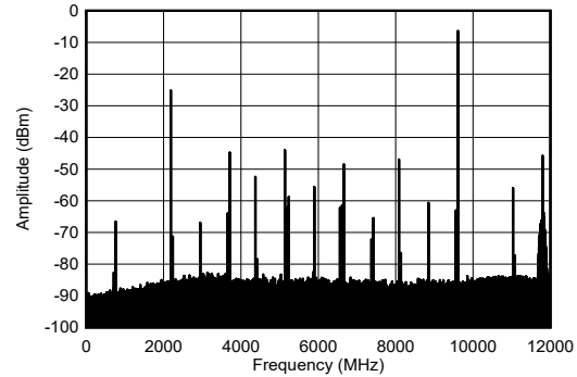
Figure 5-262. TX Single Tone Spectrum at 9.61 GHz and -1 dBFS (wideband)
