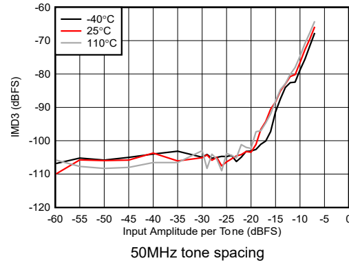
Figure 5-422. RX IMD3 vs Input Amplitude at 8.11 GHz
