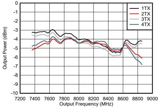
Figure 5-184. TX Output Power vs Frequency at 8.11 GHz
