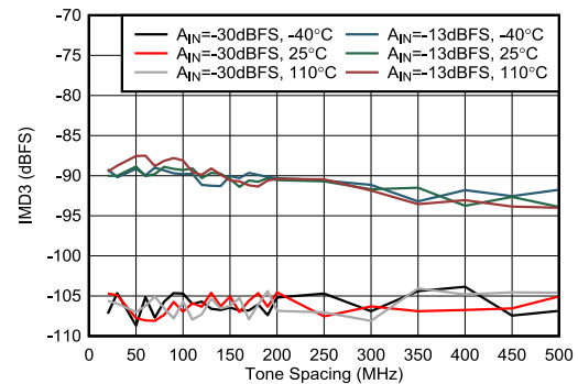
Figure 5-424. RX IMD3 vs Tone Spacing at 8.11 GHz
