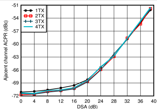
Figure 5-106. TX 20-MHz LTE ACPR vs DSA at 2.6 GHz
