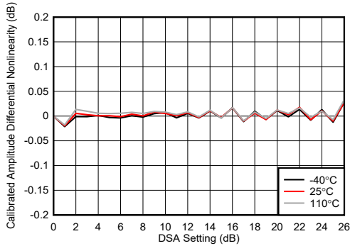
Figure 5-235. TX DSA Calibrated Amplitude Differential Nonlinearity
