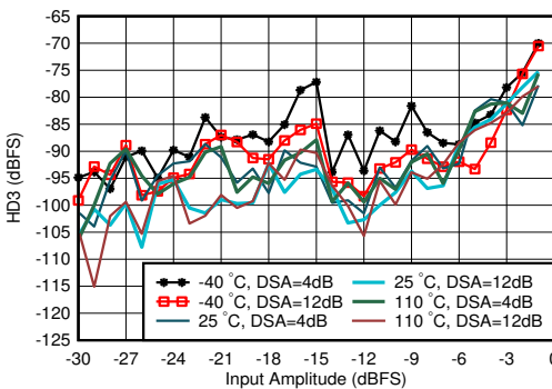
Figure 5-302. RX HD3 vs DSA Setting and Temperature at 0.8 GHz
