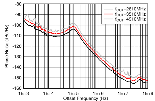
Figure 5-475. Phase Noise for 12-GHz VCO vs Offset Frequency and f_{\text{OUT}} at 25°C
