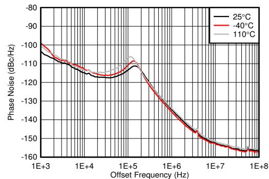
Figure 5-472. Phase Noise vs Offset Frequency for PLL and External Clock at 12 GHz
