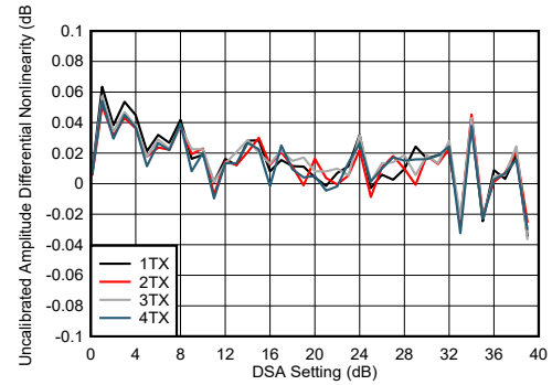
Figure 5-187. TX DSA Uncalibrated Amplitude Differential Nonlinearity at 8.11 GHz
