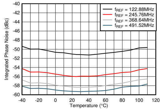
Figure 5-479. Integrated Phase Noise for 12-GHz VCO vs Temperature and f_{REF} at f_{OUT} = 2.6 GHz
