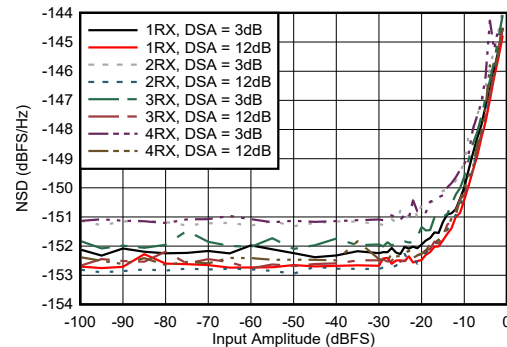
Figure 5-426. RX NSD vs Digital Amplitude at 8.1 GHz
