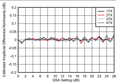
Figure 5-233. TX DSA Calibrated Amplitude Differential Nonlinearity
