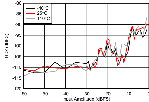
Figure 5-457. RX HD2 vs Digital Level at 9.6 GHz
