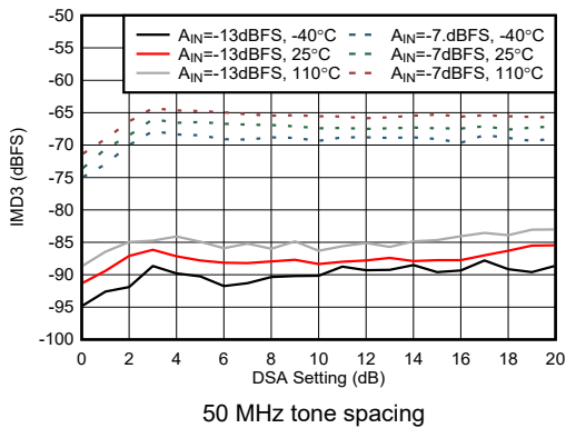
Figure 5-423. RX IMD3 vs DSA Setting at 8.11 GHz
