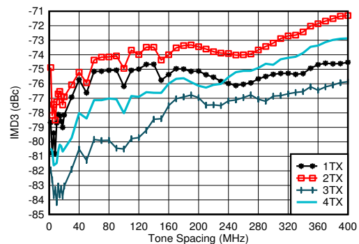
Figure 5-22. TX IMD3 vs Tone Spacing and Channel at 0.85 GHz
