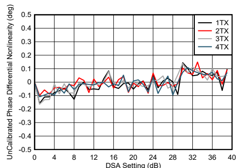
Figure 5-195. TX DSA Uncalibrated Phase Differential Nonlinearity at 8.1 GHz
