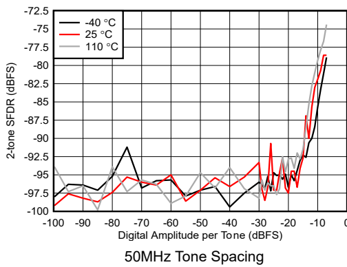
Figure 5-433. RX 2-tone SFDR vs Digital Amplitude at 8.11 GHz
