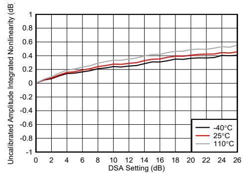
Figure 5-238. TX DSA Uncalibrated Amplitude Integrated Nonlinearity
