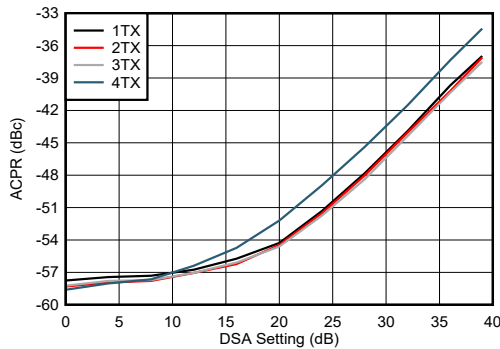
Figure 5-222. TX NR100MHz ACPR vs DSA Setting 8.11 GHz
