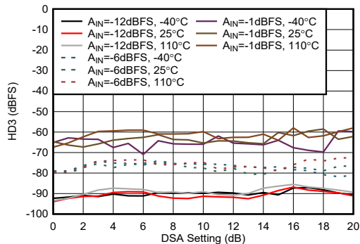
Figure 5-460. RX HD3 vs DSA Setting at 9.6 GHz
