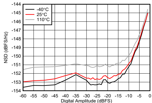
Figure 5-257. TX NSD vs Digital Amplitude at 9.61 GHz
