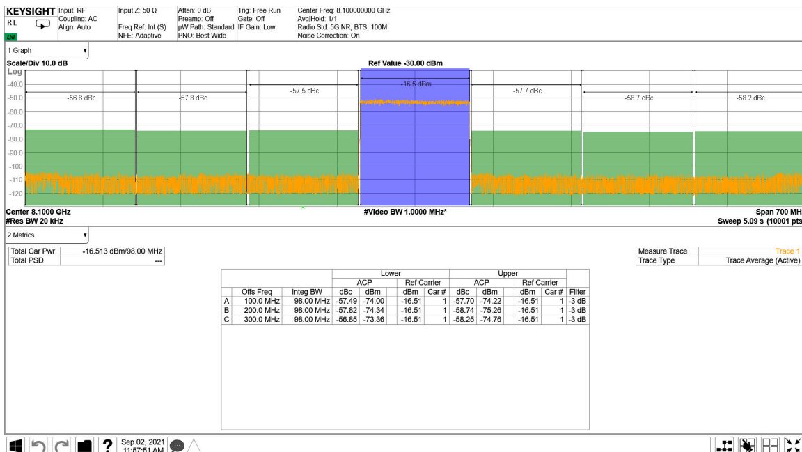
Figure 5-225. TX 100 MHz NR Output Spectrum at 8.11 GHz
