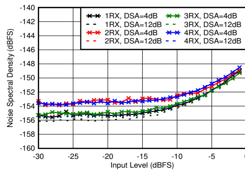
Figure 5-380. RX Noise Spectral Density vs Input Level and DSA Setting at 3.6 GHz
