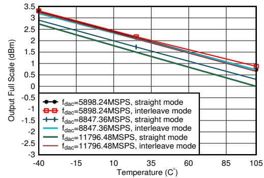
Figure 5-45. TX Output Power vs Temperature at 1.8 GHz
