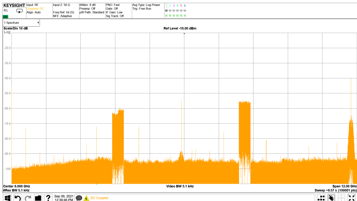
Figure 5-228. TX 4x100 MHz NR Output Spectrum 8.11 GHz
