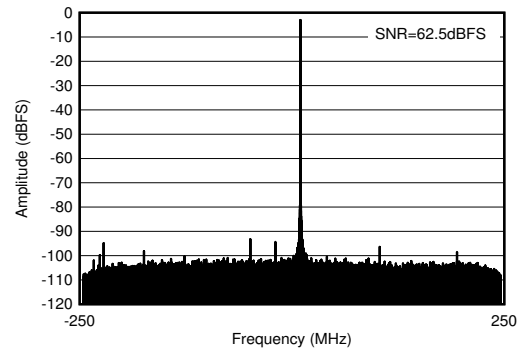
Figure 5-342. RX Output FFT at 2.6 GHz
