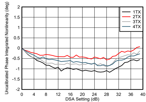
Figure 5-199. TX DSA Uncalibrated Phase Integrated Nonlinearity at 8.11 GHz
