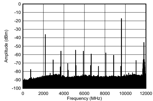
Figure 5-264. TX Single Tone Spectrum at 9.61 GHz and -6 dBFS (wideband)
