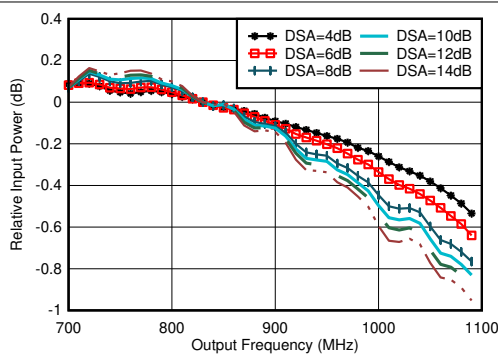
Figure 5-278. RX In-Band Gain Flatness for Channel 1RX, f_{\text{IN}} = 830 MHz
