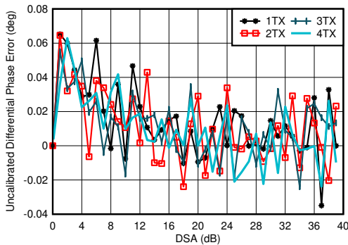
Figure 5-124. TX Uncalibrated Differential Phase Error vs DSA Setting and Channel at 3.5 GHz
