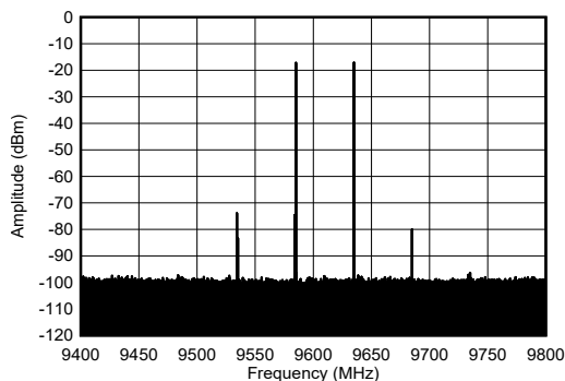
Figure 5-269. TX 2-Tone Spectrum at 9.61 GHz and -7 dBFS (400 MHz BW)
