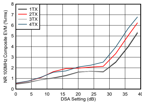
Figure 5-275. TX NR100MHz EVM vs DSA Setting at 9.61 GHz
