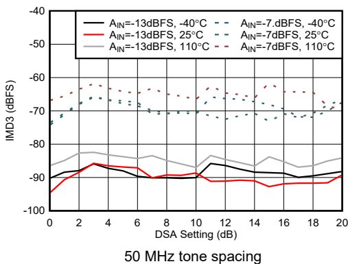
Figure 5-452. RX IMD3 vs DSA Setting at 9.6 GHz
