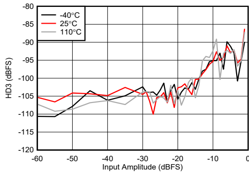
Figure 5-431. RX HD3 vs Digital Amplitude at 8.11 GHz
