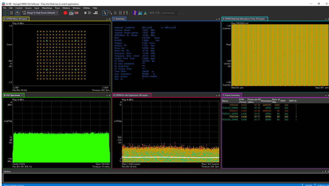
Figure 5-226. TX 100 MHz NR EVM at 8.11 GHz
