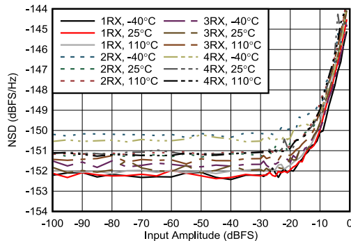
Figure 5-425. RX NSD vs Digital Amplitude at 8.1 GHz
