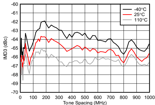
Figure 5-255. TX IMD3 vs Tone Spacing at 9.61 GHz
