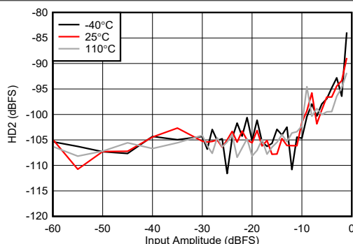
Figure 5-429. RX HD2 vs Digital Amplitude at 8.1 GHz
