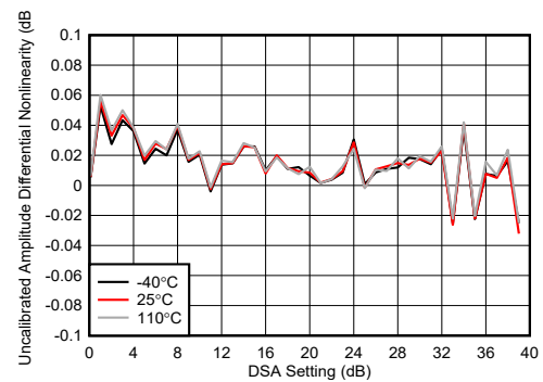
Figure 5-189. TX DSA Uncalibrated Amplitude Differential Nonlinearity at 8.11 GHz
