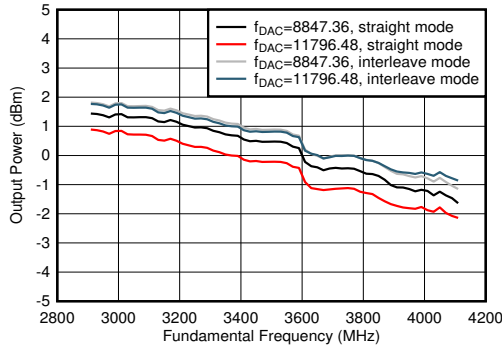
Figure 5-118. TX Output Power vs Frequency
