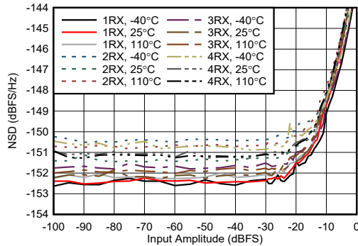
Figure 5-454. RX NSD vs Digital Amplitude at 9.6 GHz
