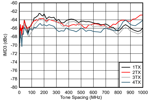
Figure 5-253. TX IMD3 vs Tone Spacing at 9.61 GHz
