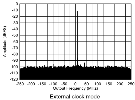
Figure 5-437. RX Single Tone Output FFT at 8.11 GHz, -12 dBFS
