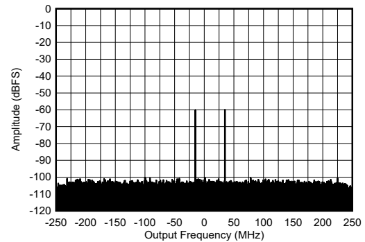
Figure 5-469. RX Two Tone Output FFT at 9.61 GHz
