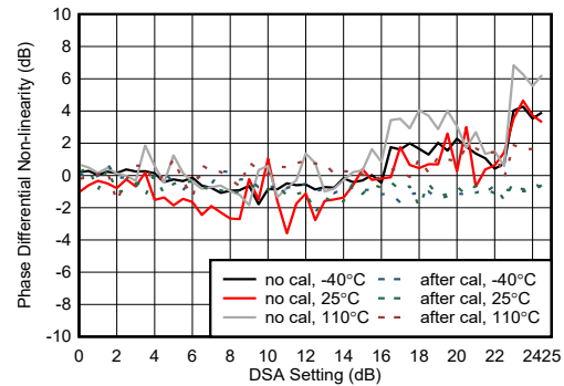
Figure 5-449. RX Phase Integrated Non-linearity at 9.6 GHz
