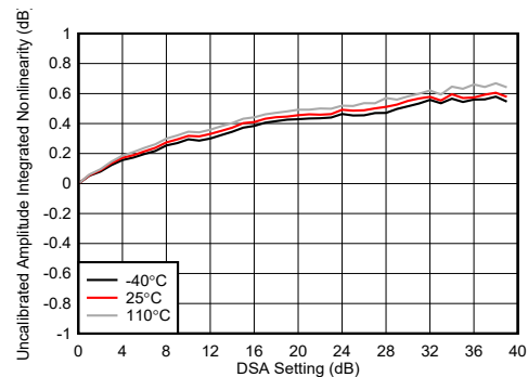
Figure 5-193. TX DSA Uncalibrated Amplitude Integrated Nonlinearity at 8.1 GHz
