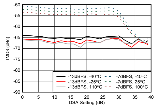
Figure 5-250. TX IMD3 vs DSA Setting at 9.61 GHz
