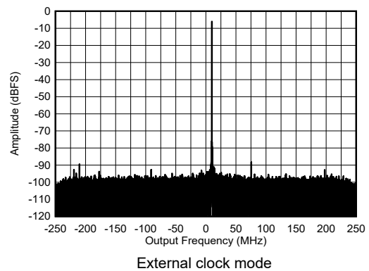
Figure 5-436. RX Single Tone Output FFT at 8.11 GHz, -6 dBFS
