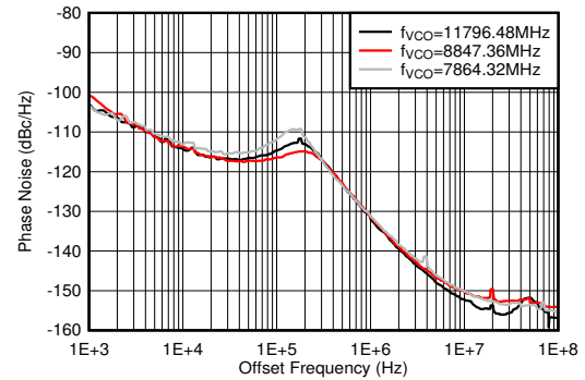
Figure 5-473. Phase Noise vs Offset Frequency and f_{\text{VCO}} at f_{\text{OUT}} = 2610 MHz
