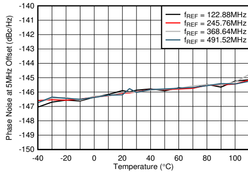
Figure 5-484. Phase Noise for 12-GHz VCO at 5-MHz Offset vs Temperature and f_{REF} at f_{OUT} = 2.6 GHz
