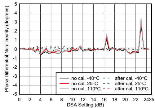
Figure 5-420. RX Phase Differential Nonlinearity at 8.11 GHz
