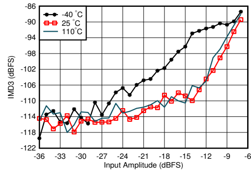
Figure 5-295. RX IMD3 vs Input Level and Temperature at 0.8 GHz
