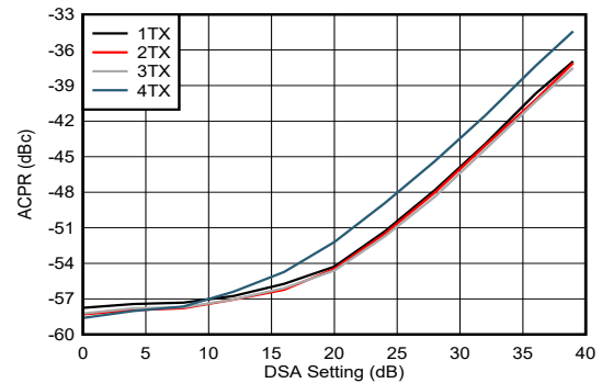
Figure 5-223. TX NR100MHz alt-ACPR vs DSA Setting 8.11 GHz
