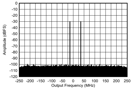
Figure 5-468. RX Two Tone Output FFT at 9.61 GHz
