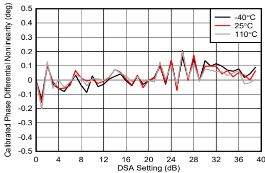
Figure 5-198. TX DSA Calibrated Phase Differential Nonlinearity at 8.11 GHz
