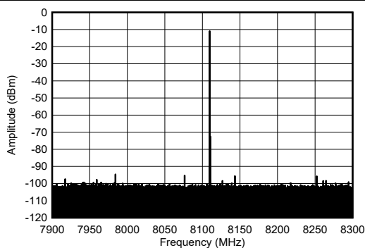
Figure 5-204. TX Single Tone Output Spectrum at 8.11 GHz
