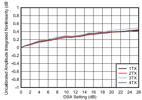
Figure 5-236. TX DSA Uncalibrated Amplitude Integrated Nonlinearity
