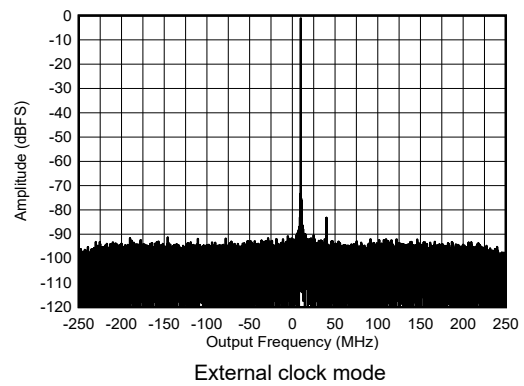
Figure 5-434. RX Single Tone Output FFT at 8.11 GHz, -1 dBFS
