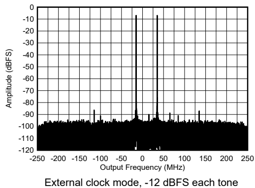
Figure 5-441. RX Dual Tone Output FFT at 8.11 GHz
