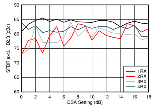
Figure 5-382. RX SFDR Excluding HD2/3 vs DSA Setting and Channel at 3.6 GHz
