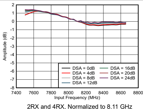
Figure 5-417. RX Amplitude vs Frequency and DSA Setting
