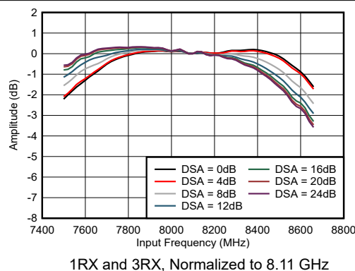
Figure 5-416. RX Amplitude vs Frequency and DSA Setting
