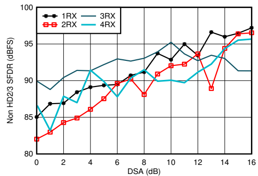
Figure 5-305. RX Non-HD2/3 vs DSA Setting at 0.8 GHz
