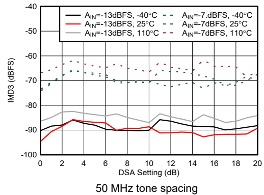
Figure 5-451. RX IMD3 vs DSA Setting at 9.6 GHz
