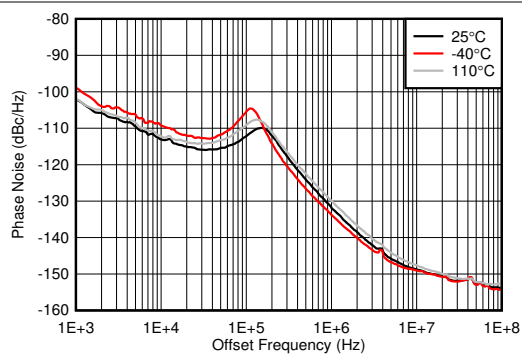
Figure 5-502. Phase Noise for 8-GHz VCO vs Offset Frequency and Temperature at f_{OUT} = 1910 MHz
