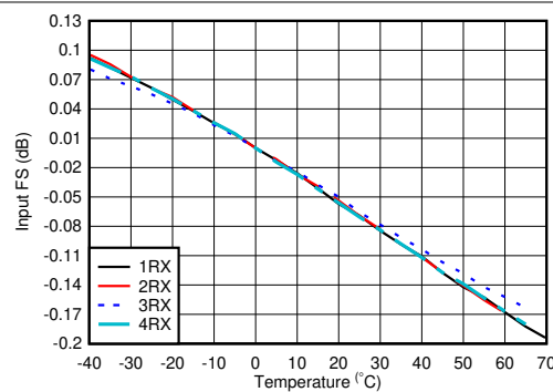
Figure 5-279. RX Input Fullscale vs Temperature and Channel at 800 MHz
