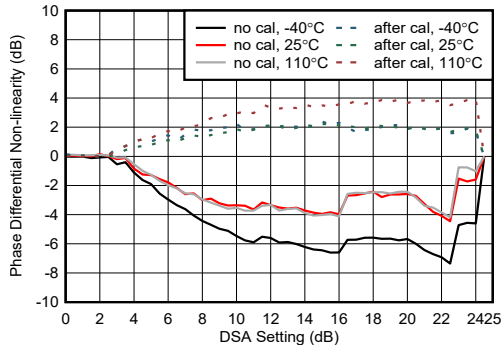
Figure 5-421. RX Phase Differential Nonlinearity at 8.11 GHz
