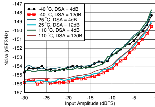
Figure 5-291. RX Noise Spectral Density vs Input Amplitude and Temperature at 0.8 GHz
