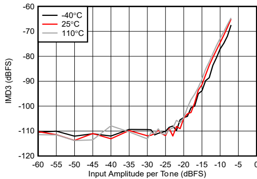
Figure 5-450. RX IMD3 vs Digital Amplitude at 9.6 GHz
