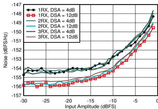
Figure 5-292. RX Noise Spectral Density vs Input Amplitude and Channel at 0.8 GHz
