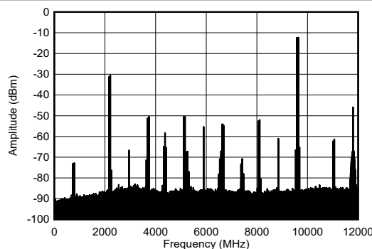
Figure 5-268. TX 2-Tone Spectrum at 9.61 GHz and -7 dBFS (wideband)
