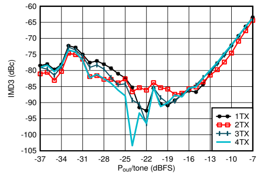
Figure 5-28. TX IMD3 vs Digital Level at 0.85 GHz
