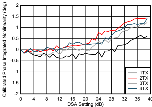
Figure 5-200. TX DSA Calibrated Phase Integrated Nonlinearity at 8.11 GHz
