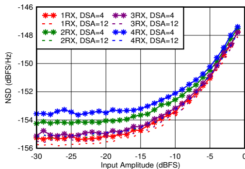
Figure 5-345. RX Noise Spectral Density vs Input Amplitude and Channel at 2.6 GHz
