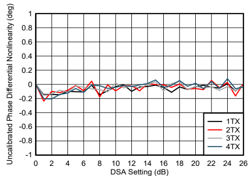
Figure 5-240. TX DSA Uncalibrated Phase Differential Nonlinearity
