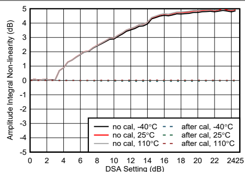
Figure 5-447. RX Amplitude Integrated Non-linearity at 9.6 GHz
