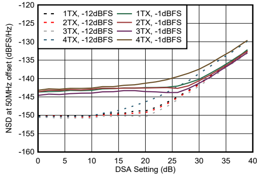
Figure 5-220. TX NSD vs DSA Setting at 8.11 GHz
