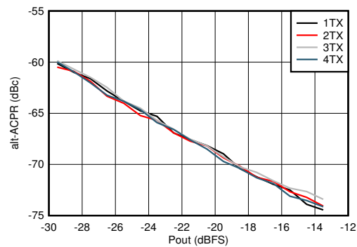
Figure 5-105. TX 20-MHz LTE alt-ACPR vs Digital Level at 2.6 GHz
