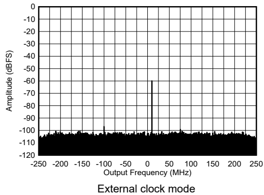
Figure 5-439. RX Single Tone Output FFT at 8.11 GHz, -60 dBFS
