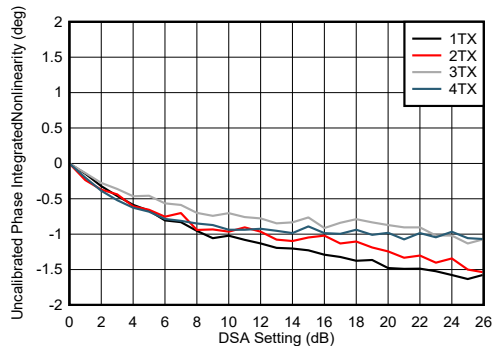
Figure 5-244. TX DSA Uncalibrated Phase Integrated Nonlinearity
