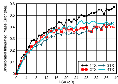
Figure 5-126. TX Uncalibrated Integrated Phase Error vs DSA Setting and Channel at 3.5 GHz
