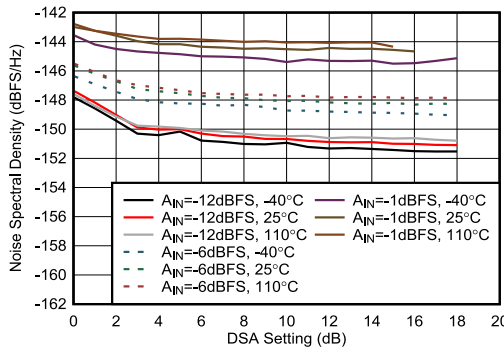
Figure 5-427. RX NSD vs DSA Setting at 8.1 GHz
