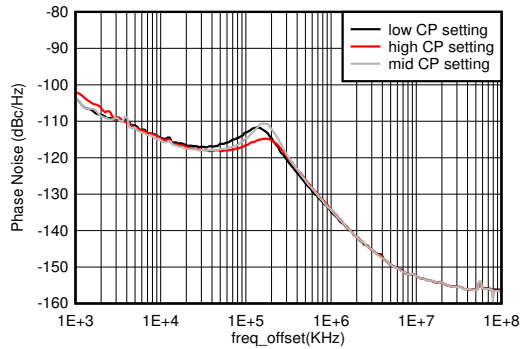
Figure 5-478. Phase Noise for 12-GHz VCO vs Offset Frequency and CP Setting at f_{OUT} = 2.6 GHz
