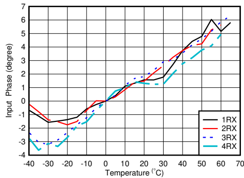
Figure 5-280. RX Input Phase vs Temperature and DSA at f_{\text{OUT}} = 0.8 \text{ GHz}
