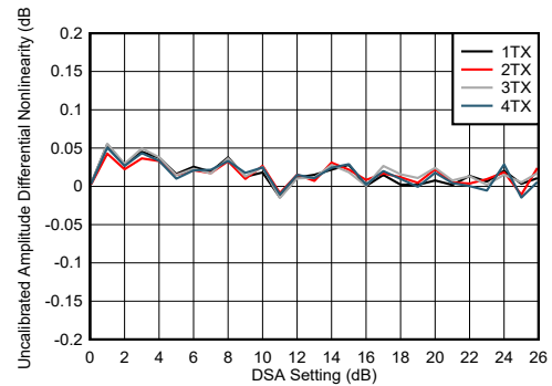
Figure 5-232. TX DSA Uncalibrated Amplitude Differential Nonlinearity
