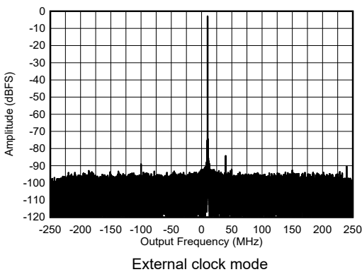
Figure 5-435. RX Single Tone Output FFT at 8.11 GHz, -3 dBFS
