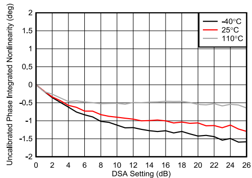
Figure 5-246. TX DSA Uncalibrated Phase Integrated Nonlinearity
