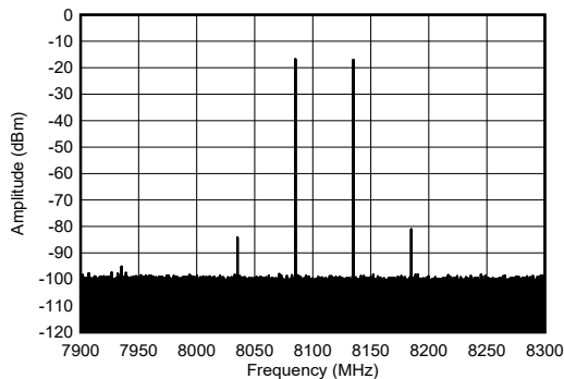
Figure 5-210. TX Dual Tone Output Spectrum at 8.11 GHz
