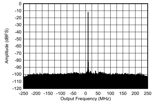
Figure 5-463. RX Single Tone Output FFT at 9.6 GHz
