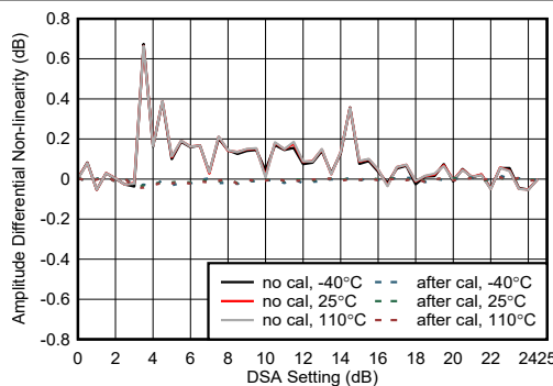
Figure 5-418. RX Amplitude Differential Nonlinearity at 8.1 GHz
