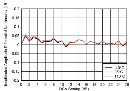
Figure 5-234. TX DSA Uncalibrated Amplitude Differential Nonlinearity
