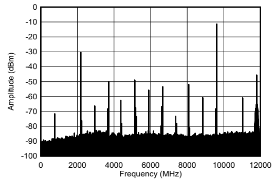
Figure 5-262. TX Single Tone Spectrum at 9.61 GHz and -1 dBFS (wideband)
