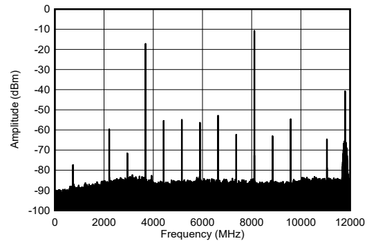
Figure 5-203. TX Single Tone Output Spectrum at 8.11 GHz
