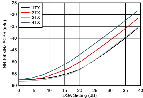
Figure 5-273. TX NR100MHz ACPR vs DSA Setting at 9.61 GHz
