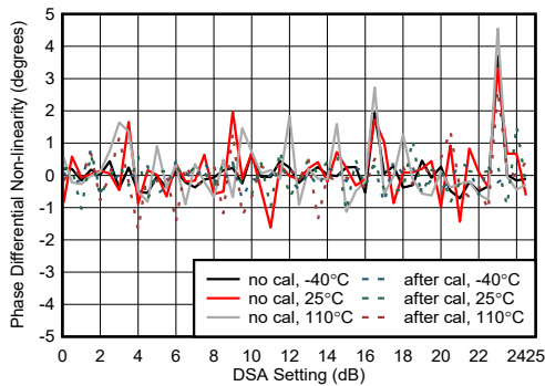
Figure 5-448. RX Phase Differential Non-linearity at 9.6 GHz
