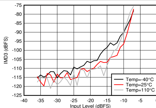
Figure 5-348. RX IMD3 vs Input Level and Temperature at 2.6 GHz
