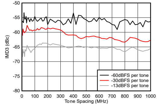
Figure 5-254. TX IMD3 vs Tone Spacing at 9.61 GHz
