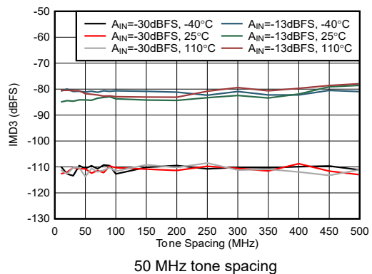
Figure 5-453. RX IMD3 vs Tone Spacing at 9.6 GHz
