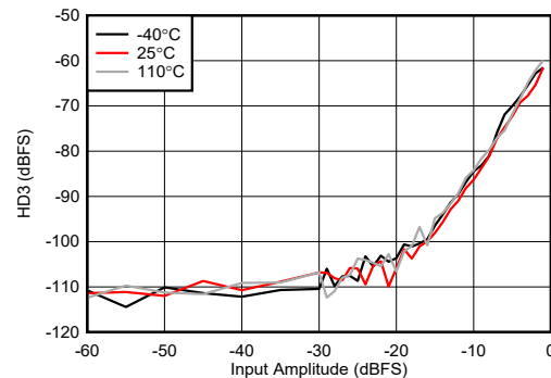
Figure 5-459. RX HD3 vs Digital Level at 9.6 GHz
