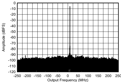
Figure 5-462. RX Single Tone Output FFT at 9.6 GHz
