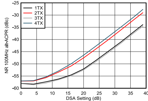
Figure 5-274. TX NR100MHz alt-ACPR vs DSA Setting at 9.61 GHz
