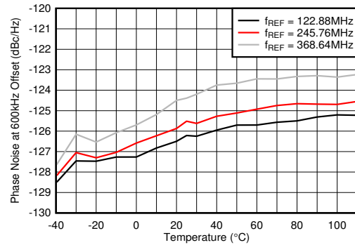
Figure 5-491. Phase Noise for 10-GHz VCO at 600 kHz vs Temperature and f_{REF} at f_{OUT} = 2.6 GHz
