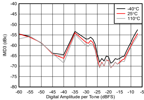
Figure 5-214. TX IMD3 vs Digital Amplitude at 8.11 GHz
