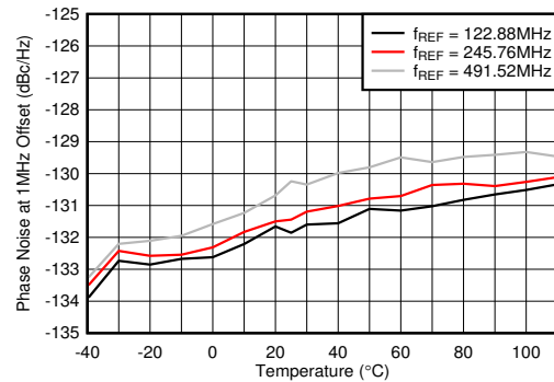
Figure 5-493. Phase Noise for 10-GHz VCO at 1 MHz vs Temperature and f_{REF} at f_{OUT} = 2.6 GHz
