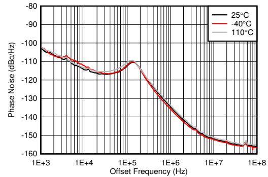
Figure 5-497. Phase Noise for 9-GHz VCO vs Offset Frequency and Temperature at f_{OUT} = 1910 MHz
