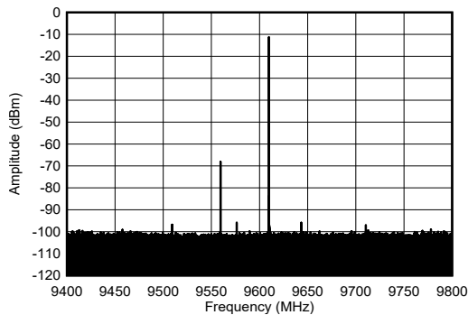
Figure 5-263. TX Single Tone Spectrum at 9.61 GHz and -1 dBFS (400 MHz BW)
