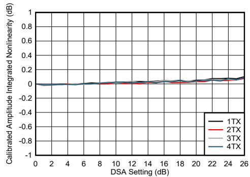
Figure 5-237. TX DSA Calibrated Amplitude Integrated Nonlinearity
