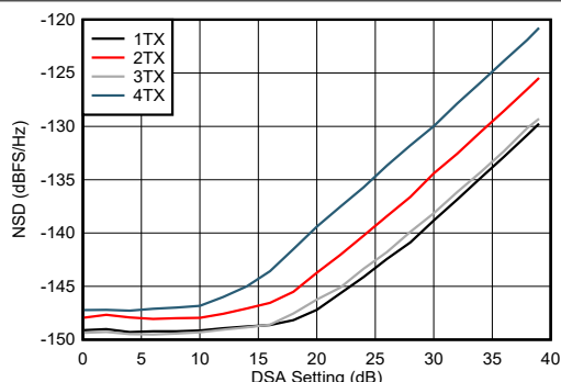
Figure 5-259. TX NSD vs DSA Setting at 9.61 GHz
