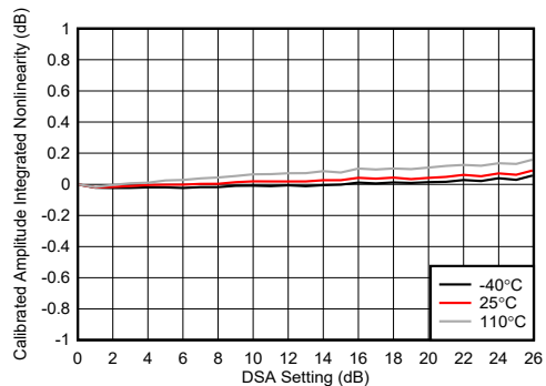
Figure 5-239. TX DSA Calibrated Amplitude Integrated Nonlinearity
