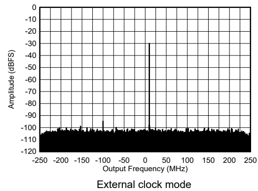
Figure 5-438. RX Single Tone Output FFT at 8.11 GHz, -30 dBFS
