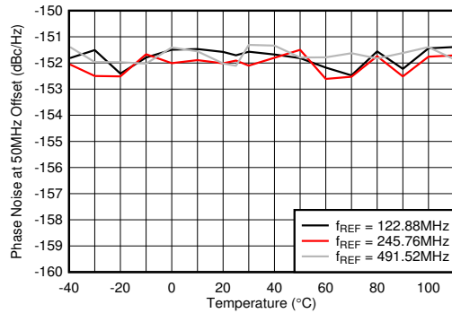
Figure 5-496. Phase Noise for 10-GHz VCO at 50 MHz vs Temperature and f_{REF} at f_{OUT} = 2.6 GHz
