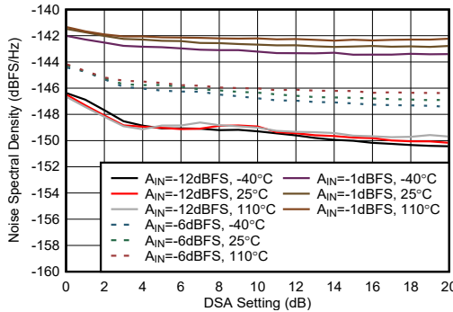
Figure 5-456. RX NSD vs DSA Setting at 9.6 GHz
