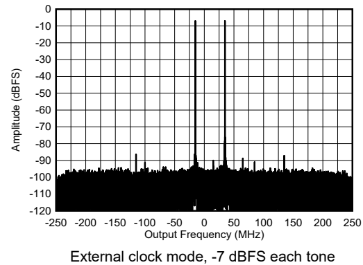
Figure 5-440. RX Dual Tone Output FFT at 8.11 GHz
