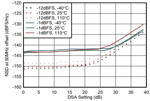
Figure 5-221. TX NSD vs DSA Setting at 8.11 GHz
