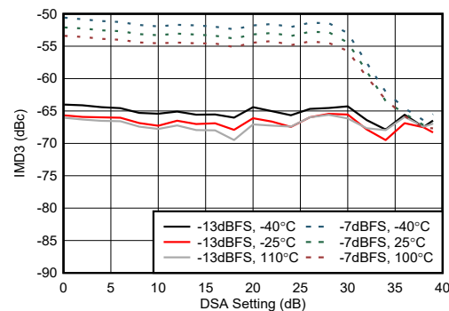
Figure 5-250. TX IMD3 vs DSA Setting at 9.61 GHz
