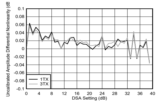
Figure 4-185. TX DSA Uncalibrated Amplitude Differential Nonlinearity at 8.11 GHz
