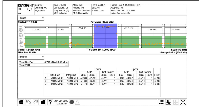
Figure 4-66. TX 20-MHz LTE Output Spectrum at 1.8425 GHz
