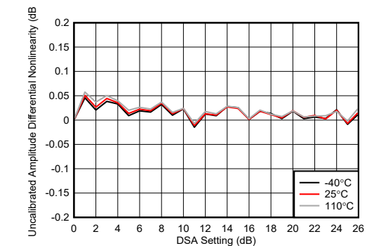
Figure 4-232. TX DSA Uncalibrated Amplitude Differential Nonlinearity
