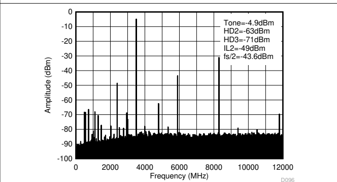
Matching at 3.5 GHz, f_{DAC} = 11.79648 GSPS, interleave mode.
