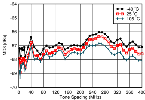
f_{\text{DAC}} = 11796.48 MSPS, interleaved mode, matching at 4.9 GHz, f_{\text{CENTER}} = 4.9\text{GHz} , -13 dBFS each tone, worst channel
