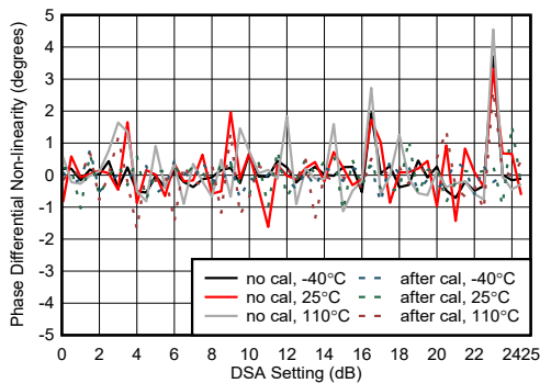
Figure 4-444. RX Phase Differential Non-linearity at 9.6 GHz
