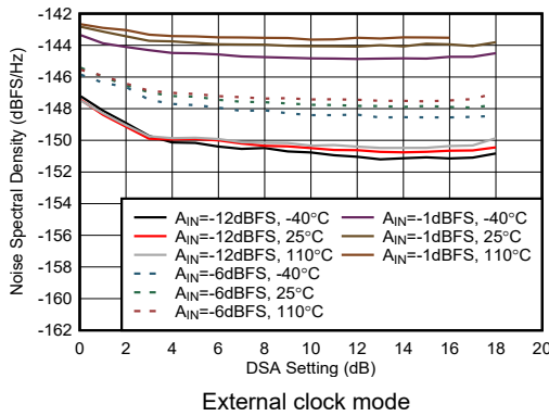
Figure 4-424. RX NSD vs DSA Setting at 8.11 GHz
