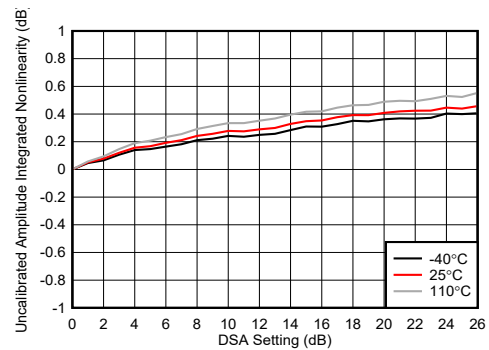
Figure 4-236. TX DSA Uncalibrated Amplitude Integrated Nonlinearity
