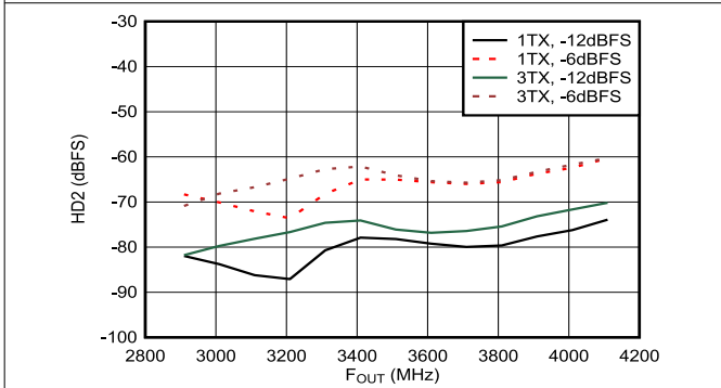
Matching at 3.5 GHz, f_{DAC} = 11.79648 GSPS, interleave mode, normalized to output power at harmonic frequency
