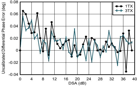
3.5 GHz Matching, included PCB and cable losses
