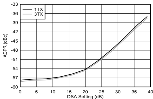
Figure 4-220. TX NR100MHz ACPR vs DSA Setting 8.11 GHz
