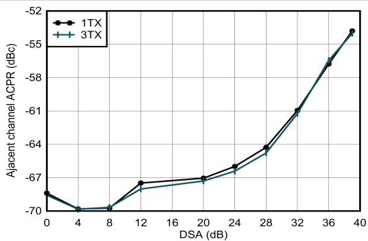
Figure 4-33. TX 20-MHz LTE ACPR vs DSA at 0.85 GHz
