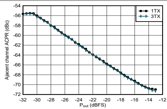
Figure 4-67. TX 20-MHz LTE ACPR vs Digital Level at 1.8425 GHz
