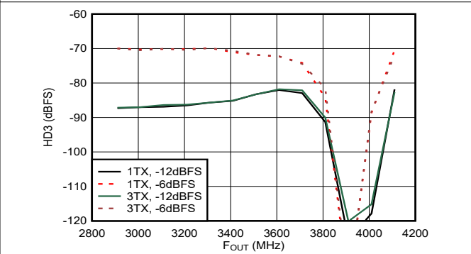
Matching at 3.5 GHz, f_{DAC} = 11.79648 GSPS, interleave mode, normalized to output power at harmonic frequency. Dip is due to HD3 falling near DC.
