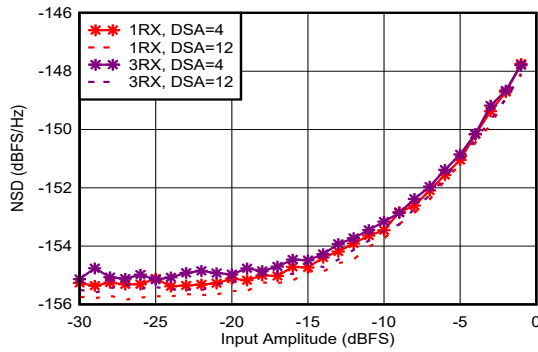
Figure 4-369. RX Noise Spectral Density vs Input Amplitude and Channel at 2.6 GHz
