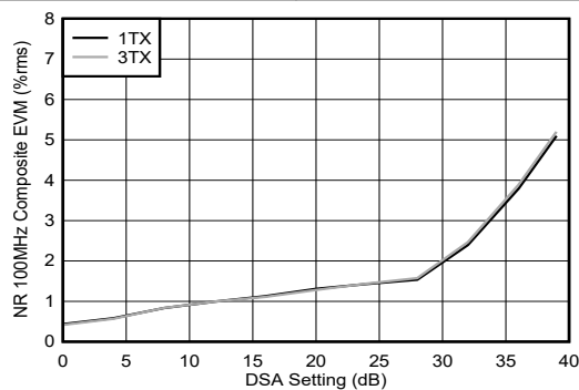
Figure 4-222. TX NR100 MHz EVM vs DSA Setting 8.11 GHz
