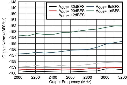
Matching at 2.6 GHz, Single tone, f_{DAC} = 11.79648\text{GSPPS} , interleave mode, 40-MHz offset
