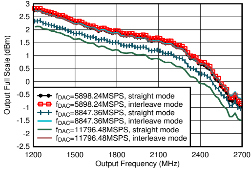
Figure 4-42. TX Output Fullscale vs Output Frequency
