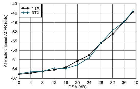
Figure 4-221. TX NR100 MHz alt-ACPR vs DSA Setting 8.11 GHz
