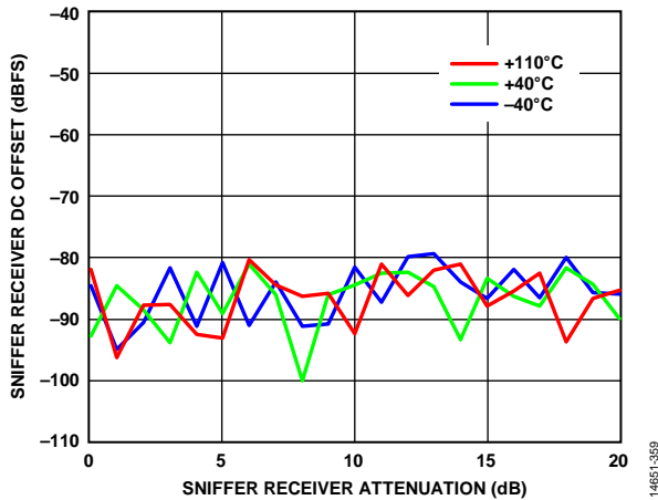
Figure 59. Sniffer Receiver DC Offset vs. Sniffer Receiver Attenuation, 600 MHz LO, CS Signal 3 MHz Offset, -35 dBm at 0 dB Attenuation, Input Power Increasing Decibel for Decibel with Attenuation, 20 MHz RF Bandwidth, 30.72 MSPS Sample Rate
