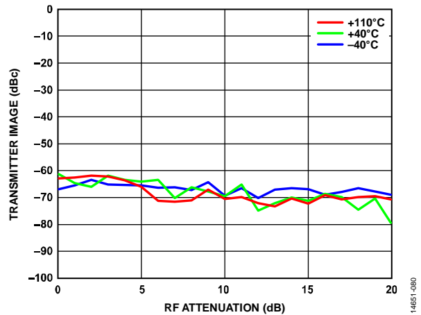
Figure 139. Transmitter Image vs. RF Attenuation, 100 MHz RF Bandwidth, 3550 MHz LO, Transmitter Quadrature Error Correction (QEC) Tracking Run with Two 20 MHz LTE Downlink Carriers, Then Image Measured with CW 10 MHz Offset from LO, 6 dB Digital Backoff, 307.2 MSPS Sample Rate
