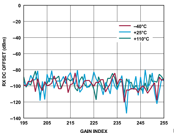
Figure 91. Receiver DC Offset vs. Gain Index, Baseband Frequency = 5.6 MHz, ADC = High Performance
