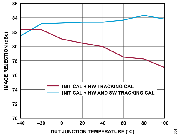
Figure 46. Receiver Image Rejection vs. DUT Junction Temperature (Low to High), Tone 1 Baseband Frequency = -5.1MHz, Tone 2 Baseband Frequency = 13.9 MHz, ADC = High Performance, P_{OUT} = -11.1 dBFS
