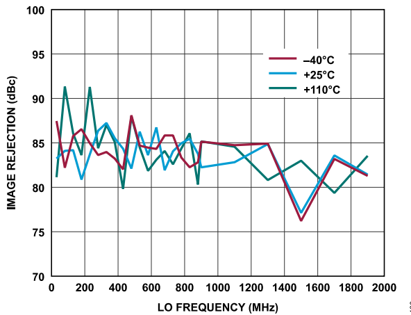
Figure 10. Receiver Image Rejection vs. LO Frequency, Baseband Frequency = 5.6 MHz, ADC = High Performance, Initialization Calibration and Hardware Tracking Calibration Only
