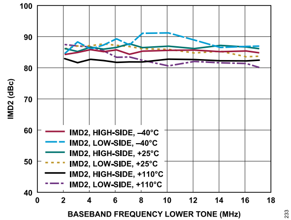
Figure 139. Transmitter IMD2 vs. Baseband Frequency, Transmitter Attenuation Code = 0, f_1 = Baseband Frequency, f_2 = Baseband Frequency + 1 MHz
