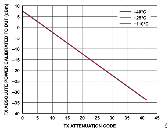
Figure 324. Transmitter Absolute Power Calibrated to DUT vs. Transmitter Attenuation Code, Baseband Frequency = 2.1 kHz, Backoff = 0.2 dBFS
