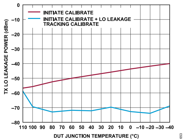
Figure 72. Transmitter LO Leakage Power vs. DUT Junction Temperature (High to Low), Baseband Frequency = 4 MHz, Backoff = 0.5 dBFS, Attenuation Code = 0
