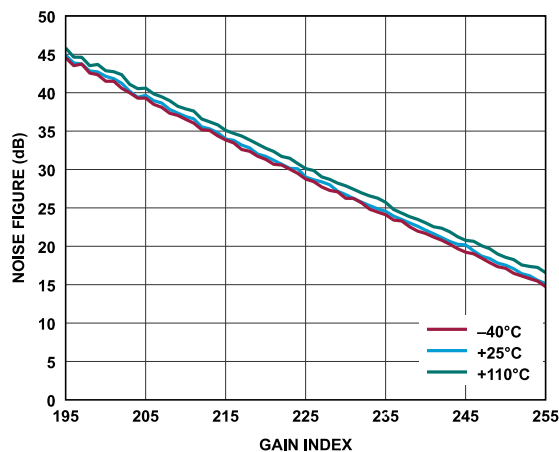
Figure 286. Receiver Noise Figure vs. Gain Index, Baseband Frequency = 2.1 kHz, ADC = Low Power
