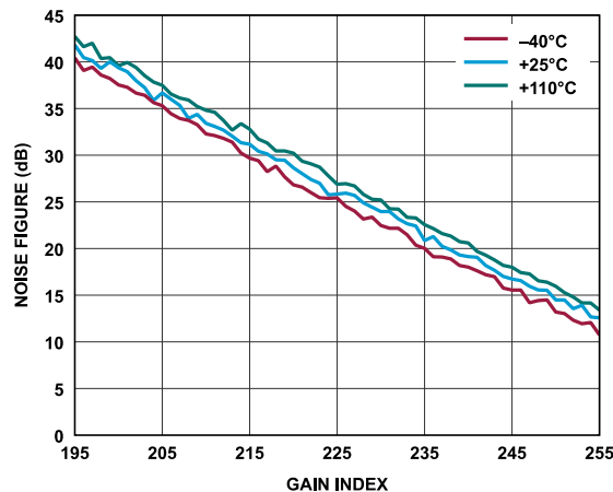
Figure 111. Receiver Noise Figure vs. Gain Index, Baseband Frequency = 5.6 MHz, ADC = Low Power
