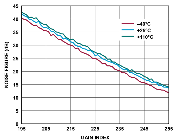
Figure 146. Receiver Noise Figure vs. Gain Index, Baseband Frequency = 5.6 MHz, ADC = Low Power
