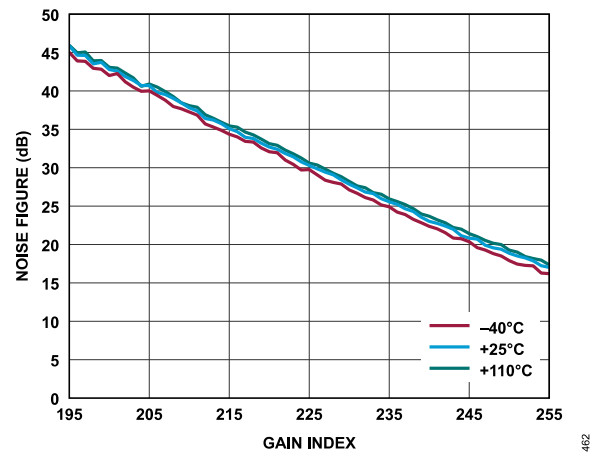
Figure 310. Receiver Noise Figure vs. Gain Index, Baseband Frequency = 2.1 kHz, ADC = Low Power
