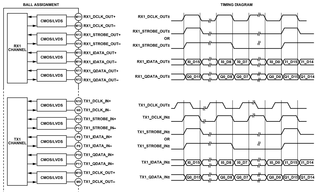
Figure 365. LSSI in 2-Lane Data Mode, DDR
