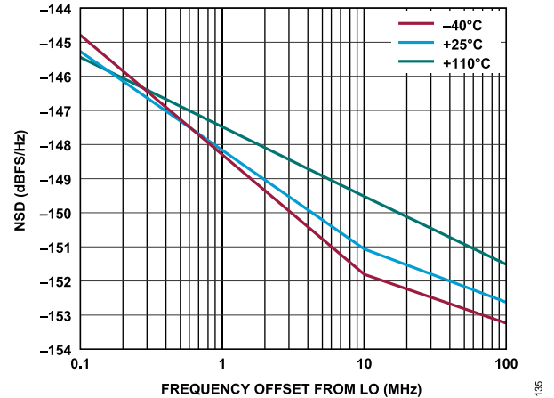
Figure 42. Transmitter NSD vs. Frequency Offset from LO, Baseband Frequency = 5.6 MHz, Transmitter Channel = Channel 1
