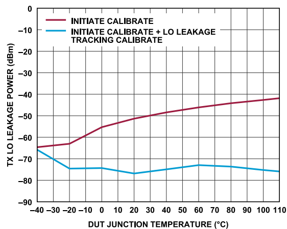
Figure 71. Transmitter LO Leakage Power vs. DUT Junction Temperature (Low to High), Baseband Frequency = 4 MHz, Backoff = 0.5 dBFS, Attenuation Code = 0
