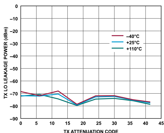
Figure 259. Transmitter LO Leakage Power vs. Transmitter Attenuation Code, Baseband Frequency = 2.1 kHz, Backoff = 6 dBFS, Initialization Calibration Only
