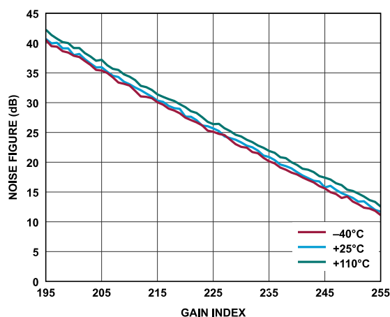
Figure 285. Receiver Noise Figure vs. Gain Index, Baseband Frequency = 2.1 kHz, ADC = High Performance
