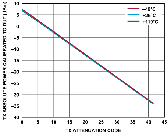
Figure 142. Transmitter Absolute Power Calibrated to DUT vs. Transmitter Attenuation Code, Baseband Frequency = 18 MHz, Backoff = 0.2 dBFS
