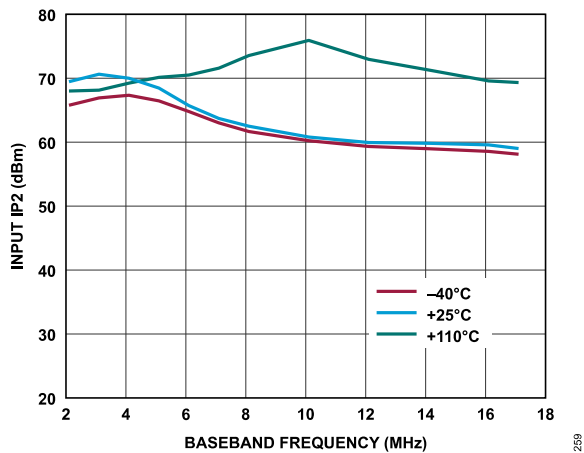
Figure 116. Receiver Input IP2 vs. Baseband Frequency, ADC = Low Power, f_1 = Baseband Frequency, f_2 = Baseband Frequency + 1 MHz, Gain Index = 255
