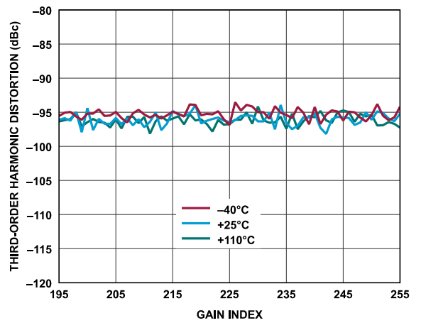
Figure 176. Receiver Third-Order Harmonic Distortion vs. Gain Index, Baseband Frequency = 2.1 kHz, ADC = Low Power
