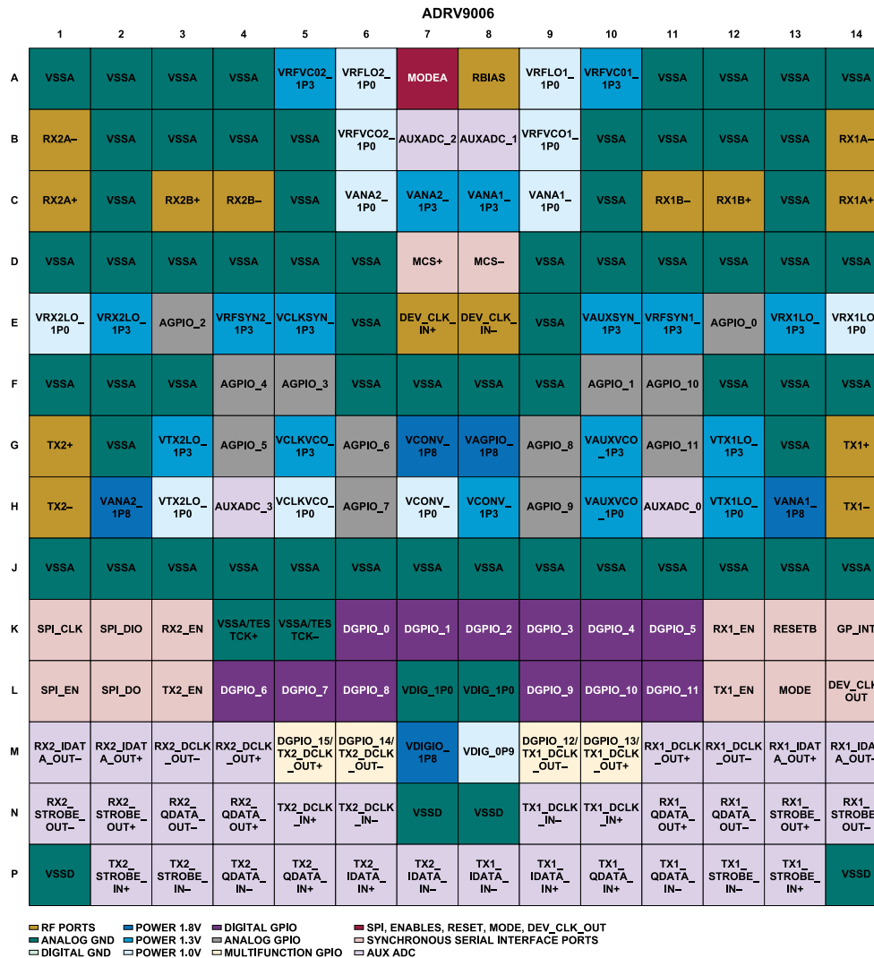
Figure 3. Pin Configuration
