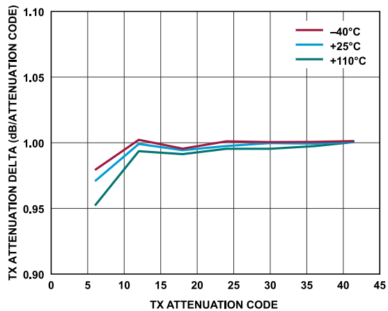
Figure 143. Transmitter Attenuation Delta vs. Transmitter Attenuation Code, Baseband Frequency = 18 MHz, Backoff = 0.2 dBFS
