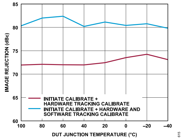
Figure 83. Receiver Image Rejection vs. DUT Junction Temperature (High to Low), Tone 1 Baseband Frequency = -5.1 MHz, Tone 2 Baseband Frequency = 13.9 MHz, ADC = Low Power, P_{OUT} = -11.1 dBFS
