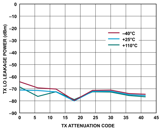
Figure 234. Transmitter LO Leakage Power vs. Transmitter Attenuation Code, Baseband Frequency = 2.1 kHz, Backoff = 6 dBFS, Initialization Calibration Only
