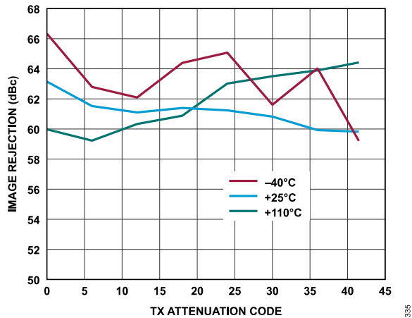
Figure 167. Transmitter Image Rejection vs. Transmitter Attenuation Code, Baseband Frequency = 2.1 kHz, Backoff = 0.2 dBFS
