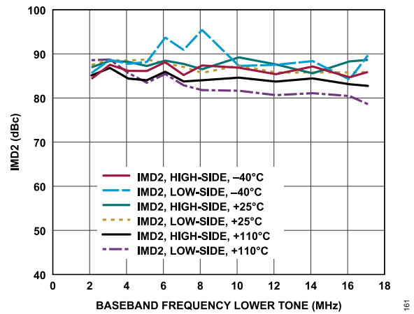
Figure 53. Transmitter IMD2 vs. Baseband Frequency, Transmitter Attenuation Code = 0, f_1 = Baseband Frequency, f_2 = Baseband Frequency + 1 MHz
