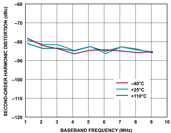
Figure 111. Receiver Second-Order Harmonic Distortion vs. Baseband Frequency, Gain Index = 255, ADC = Low Power
