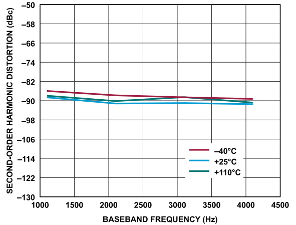
Figure 191. Receiver Second-Order Harmonic Distortion vs. Baseband Frequency, Gain Index = 255, ADC = Low Power
