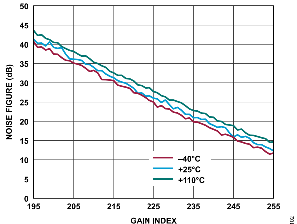
Figure 6. Receiver Noise Figure vs. Gain Index, Baseband Frequency = 5.6 MHz, ADC = Low Power
