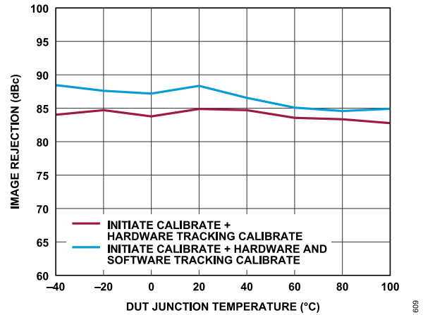
Figure 58. Receiver Image Rejection vs. DUT Junction Temperature (Low to High), Tone 1 Baseband Frequency = -5.1 MHz, Tone 2 Baseband Frequency = 13.9 MHz, ADC = Low Power, P_{OUT} = -11.1 dBFS
