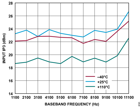
Figure 179. Receiver Input IP3 vs. Baseband Frequency, ADC = Low Power, f_1 = Baseband Frequency + 1 MHz, f_2 = Baseband Frequency + 2 MHz, Gain Index = 255, First-Order TIA with f_{1dB} = 4 MHz, P_{OUT} = -13.6 dBFS at -40°C and +25°C, P_{OUT} = -16.6 dBFS at +110°C
