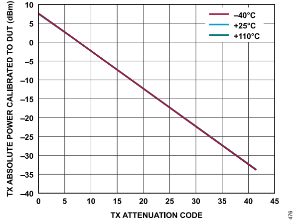
Figure 229. Transmitter Absolute Power Calibration to DUT vs. Transmitter Attenuation Code, Baseband Frequency = 2.1 kHz, Backoff = 0.2 dBFS
