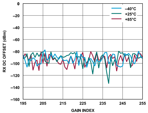
Figure 114. Receiver DC Offset vs. Gain Index, Baseband Frequency = 5.6 MHz, ADC = Low Power
