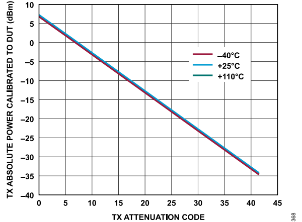
Figure 181. Transmitter Absolute Power Calibrated to DUT vs. Transmitter Attenuation Code, Baseband Frequency = 2.1 kHz, Backoff = 0.2 dBFS
