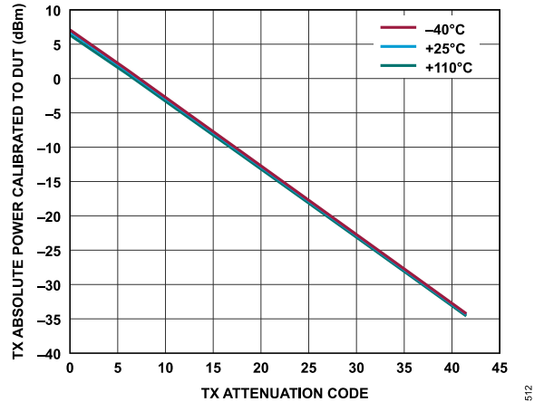
Figure 245. Transmitter Absolute Power Calibrated to DUT vs. Transmitter Attenuation Code, Baseband Frequency = 2.1 kHz, Backoff = 0.2 dBFS
