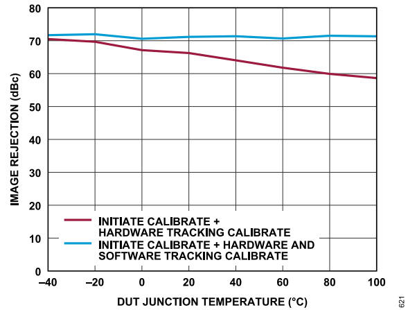
Figure 133. Receiver Image Rejection vs. DUT Junction Temperature (Low to High), Tone 1 Baseband Frequency = -5.1 MHz, Tone 2 Baseband Frequency = 13.9 MHz, ADC = Low Power, P_{OUT} = -11.1 dBFS
