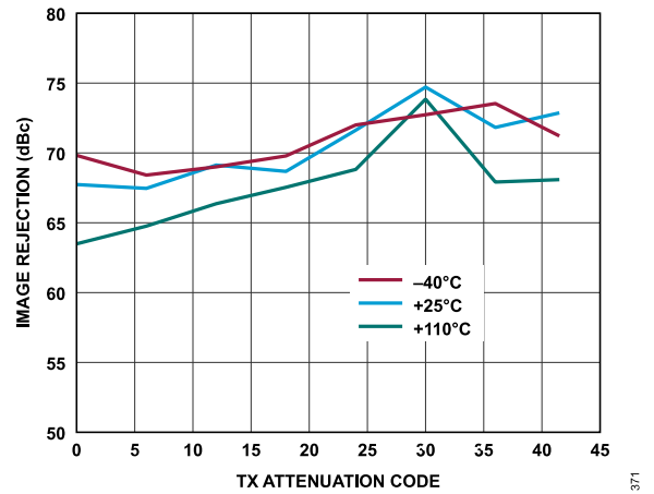
Figure 183. Transmitter Image Rejection vs. Transmitter Attenuation Code, Baseband Frequency = 2.1 kHz, Backoff = 0.2 dBFS, Initialization Calibration Only
