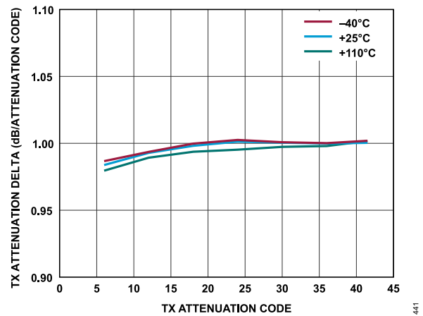
Figure 214. Transmitter Attenuation Delta vs. Transmitter Attenuation Code, Baseband Frequency = 2.1 kHz, Backoff = 0.2 dBFS
