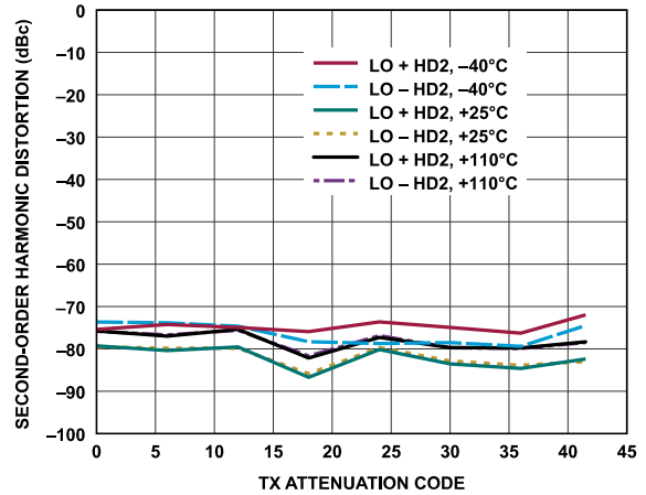
Figure 169. Transmitter Second-Order Harmonic Distortion vs. Transmitter Attenuation Code, Baseband Frequency = 2.1 kHz, Backoff = 0.2 dBFS
