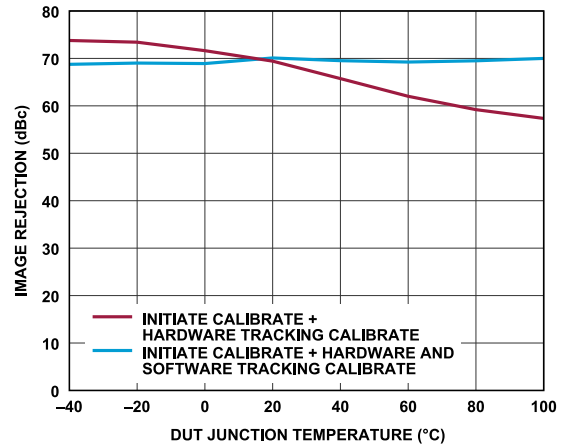
Figure 108. Receiver Image Rejection vs. DUT Junction Temperature (Low to High), Tone 1 Baseband Frequency = -5.1 MHz, Tone 2 Baseband Frequency = 13.9 MHz, ADC = Low Power, P_{OUT} = -11.1 dBFS
