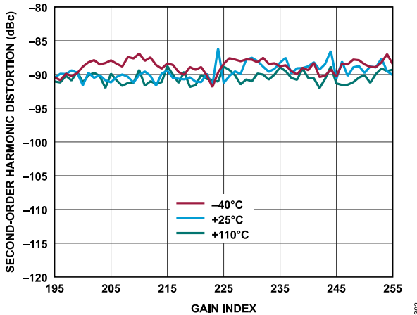
Figure 190. Receiver Second-Order Harmonic Distortion vs. Gain Index, Baseband Frequency = 2.1 kHz, ADC = Low Power
