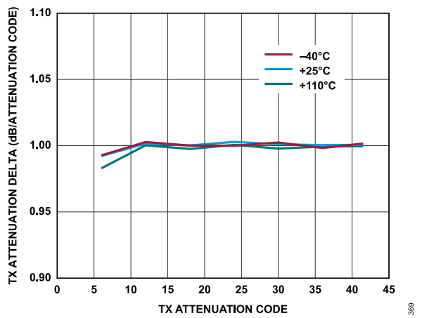
Figure 182. Transmitter Attenuation Delta vs. Transmitter Attenuation Code, Baseband Frequency = 2.1 kHz, Backoff = 0.2 dBFS
