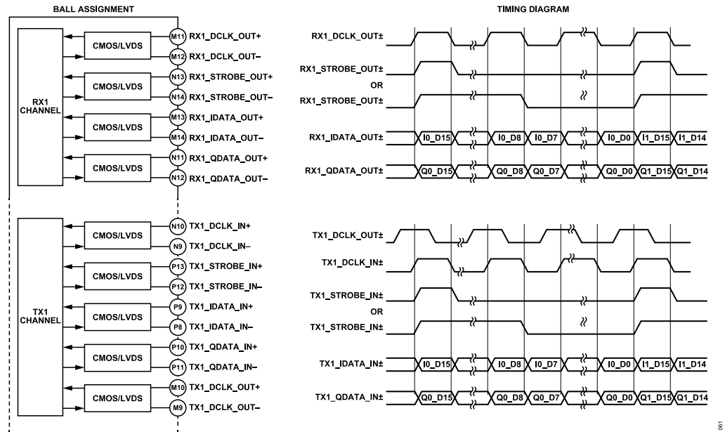
Figure 263. LSSI in 2-Lane Data Mode, DDR
