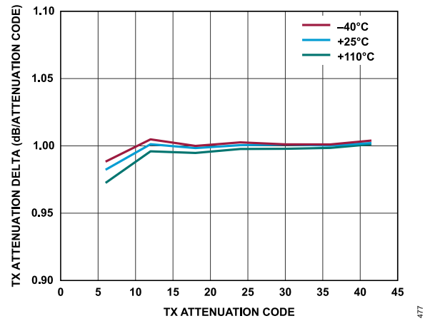
Figure 230. Transmitter Attenuation Delta vs. Transmitter Attenuation Code, Baseband Frequency = 2.1 kHz, Backoff = 0.2 dBFS
