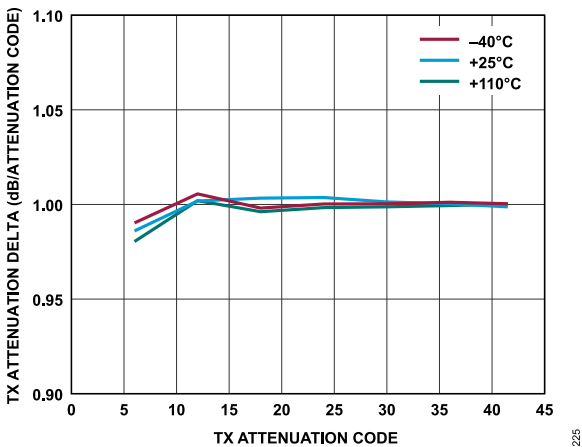
Figure 92. Transmitter Attenuation Delta vs. Transmitter Attenuation Code, Baseband Frequency = 18 MHz, Backoff = 0.2 dBFS
