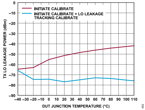
Figure 51. Transmitter LO Leakage Power vs. DUT Junction Temperature (Low to High), Baseband Frequency = 4 MHz, Backoff = 0.5 dBFS, Attenuation Code = 0
