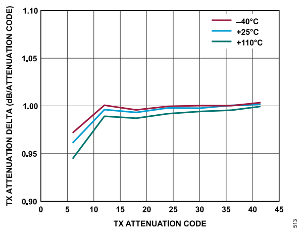
Figure 246. Transmitter Attenuation Delta vs. Transmitter Attenuation Code, Baseband Frequency = 2.1 kHz, Backoff = 0.2 dBFS
