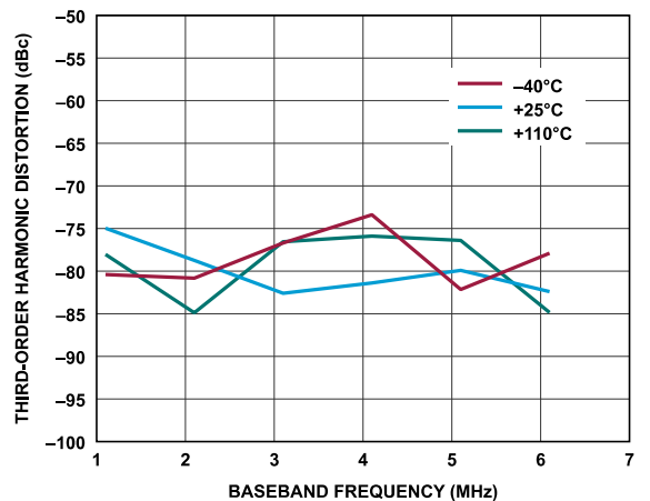
Figure 113. Receiver Third-Order Harmonic Distortion vs. Baseband Frequency, Gain index = 255, ADC = Low Power
