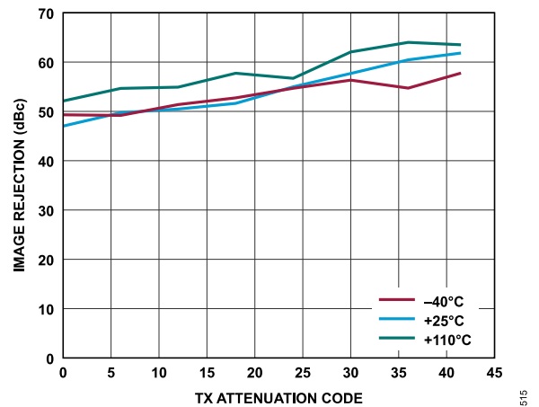
Figure 247. Transmitter Image Rejection vs. Transmitter Attenuation Code, Baseband Frequency = 2.1 kHz, Backoff = 0.2 dBFS, Initialization Calibration Only
