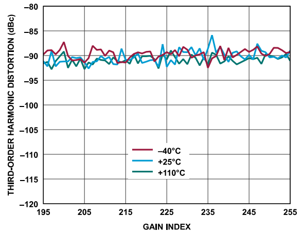
Figure 192. Receiver Third-Order Harmonic Distortion vs. Gain Index, Baseband Frequency = 2.1 kHz, ADC = Low Power
