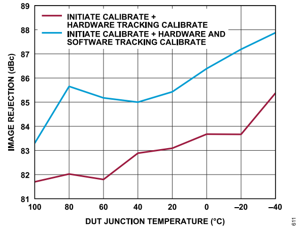
Figure 59. Receiver Image Rejection vs. DUT Junction Temperature (High to Low), Tone 1 Baseband Frequency = -5.1 MHz, Tone 2 Baseband Frequency = 13.9 MHz, ADC = Low Power, P_{OUT} = -11.1 dBFS
