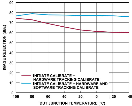
Figure 109. Receiver Image Rejection vs. DUT Junction Temperature (High to Low), Tone 1 Baseband Frequency = -5.1 MHz, Tone 2 Baseband Frequency = 13.9 MHz, ADC = Low Power, P_{OUT} = -11.1 dBFS
