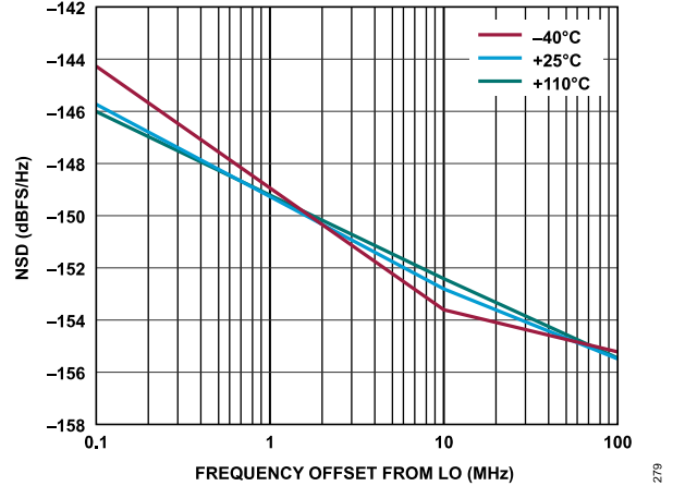
Figure 130. Transmitter NSD vs. Frequency Offset from LO, Baseband Frequency = 5.6 MHz, Transmitter Channel = Channel 1
