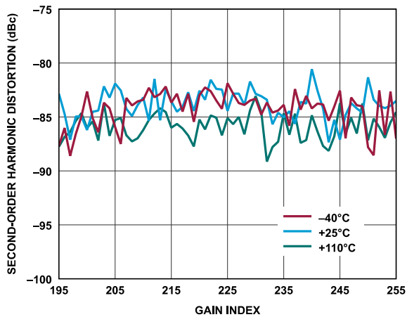
Figure 110. Receiver Second-Order Harmonic Distortion vs. Gain Index, Baseband Frequency = 5.6 MHz, ADC = Low Power
