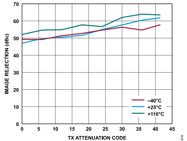
Figure 231. Transmitter Image Rejection vs. Transmitter Attenuation Code, Baseband Frequency = 2.1 kHz, Backoff = 0.2 dBFS, Initialization Calibration Only
