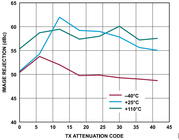
Figure 122. Transmitter Image Rejection vs. Transmitter Attenuation Code, Baseband Frequency = 18 MHz, Backoff = 0.2 dBFS, Initialization Calibration Only
