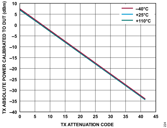
Figure 91. Transmitter Absolute Power Calibrated to DUT vs. Transmitter Attenuation Code, Baseband Frequency = 18 MHz, Backoff = 0.2 dBFS
