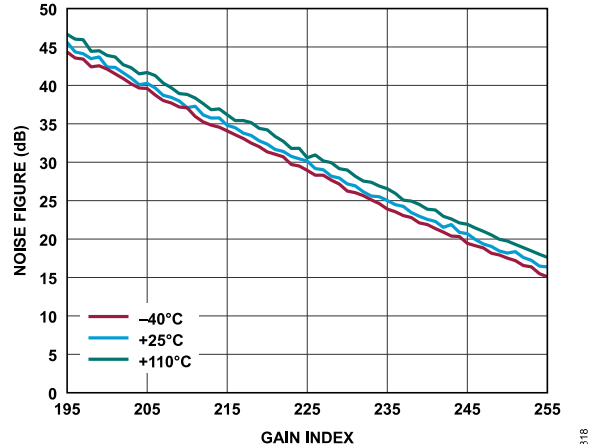
Figure 157. Receiver Noise Figure vs. Gain Index, Baseband Frequency = 2.1 kHz, ADC = Low Power
