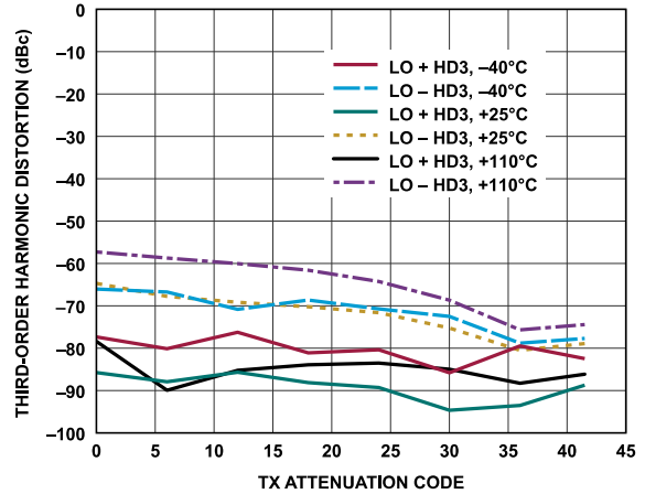
Figure 168. Transmitter Third-Order Harmonic Distortion vs. Transmitter Attenuation Code, Baseband Frequency = 2.1 kHz, Backoff = 0.2 dBFS, Initialization Calibration Only
