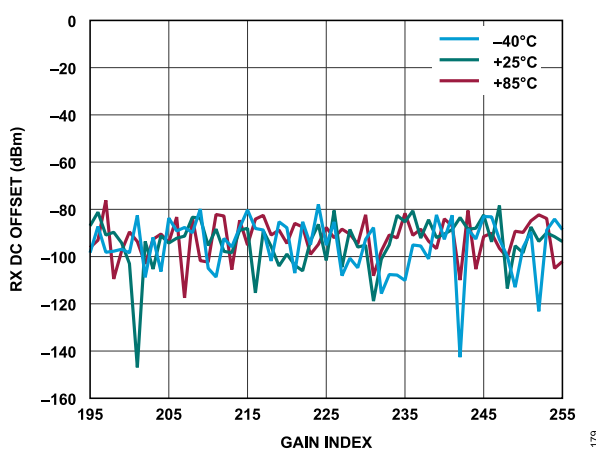
Figure 64. Receiver DC Offset vs. Gain Index, Baseband Frequency = 5.6 MHz, ADC = Low Power
