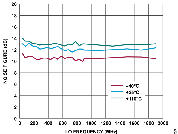
Figure 7. Receiver Noise Figure vs. LO Frequency, Baseband Frequency = 5.6 MHz, ADC = Low Power
