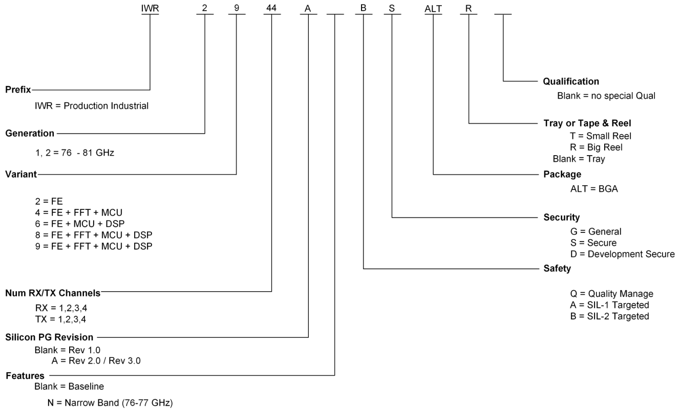
Figure 10-1. Device Nomenclature
