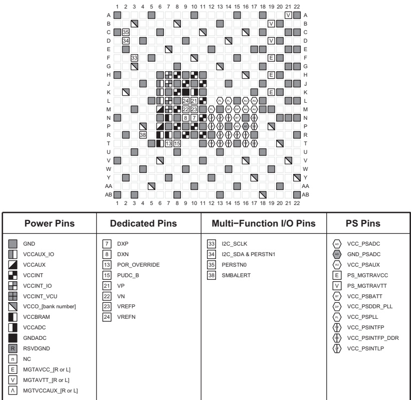
Figure 4-4: SBVA484 Package—XCZU2CG, XCZU2EG, XCZU3CG, XCZU3EG, XAZU2EG, and XAZU3EG Power, Dedicated, and Multi-function Pin Diagram
