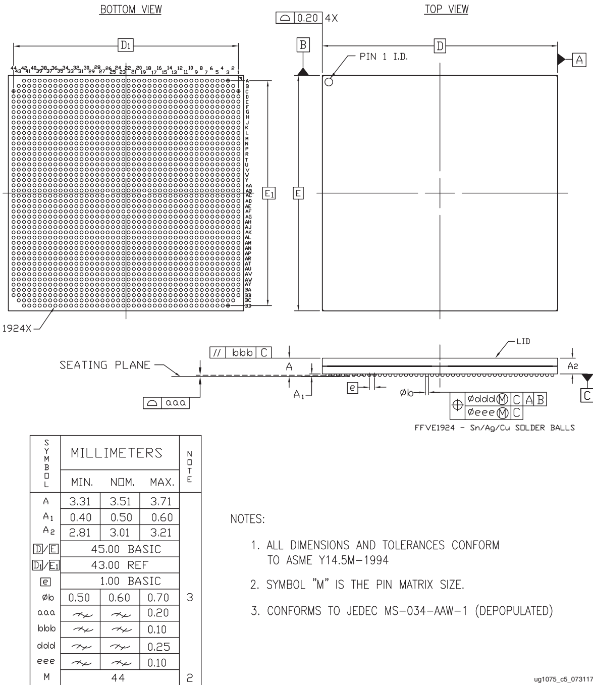
Figure 5-36: Package Dimensions for FFVE1924 (XCZU17EG and XCZU19EG)
