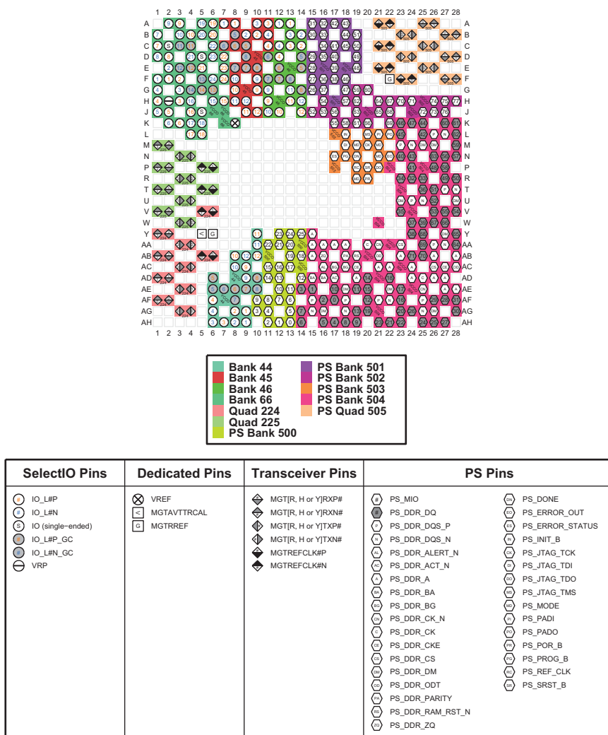
Figure 4-19: SFVD784 Package—XCZU3TCG and XCZU3TEG I/O Bank Diagram
