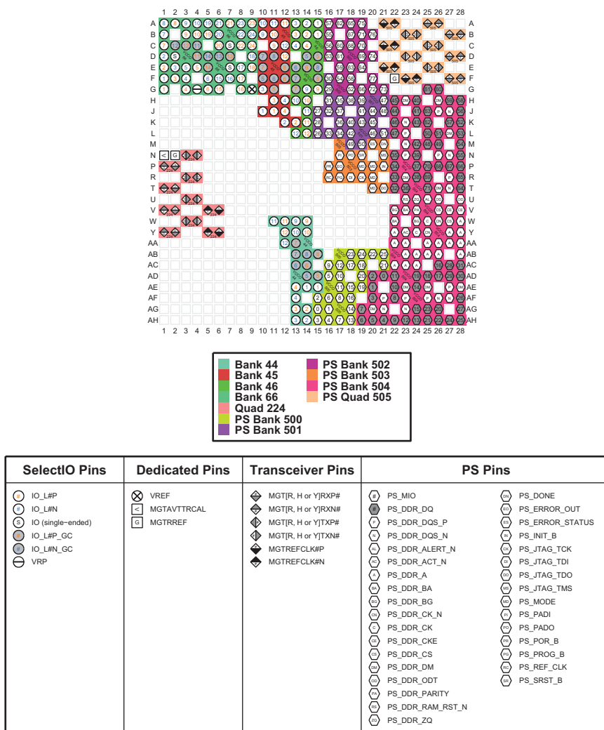
Figure 4-17: SFVC784 Package—XCZU3TCG and XCZU3TEG I/O Bank Diagram
