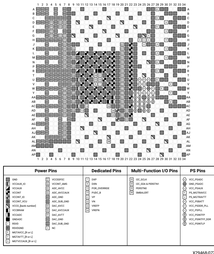
Figure 4-60: FFVE1156 and FSVE1156 Packages—XCZU48DR and XQZU48DR Power, Dedicated, and Multi-function Pin Diagram
