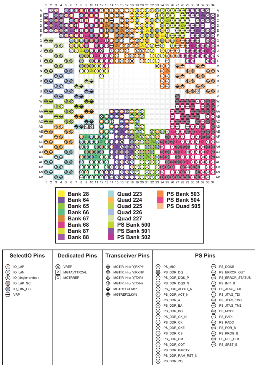
Figure 4-43: FFVC1156 Package—XCZU7EV I/O Bank Diagram
