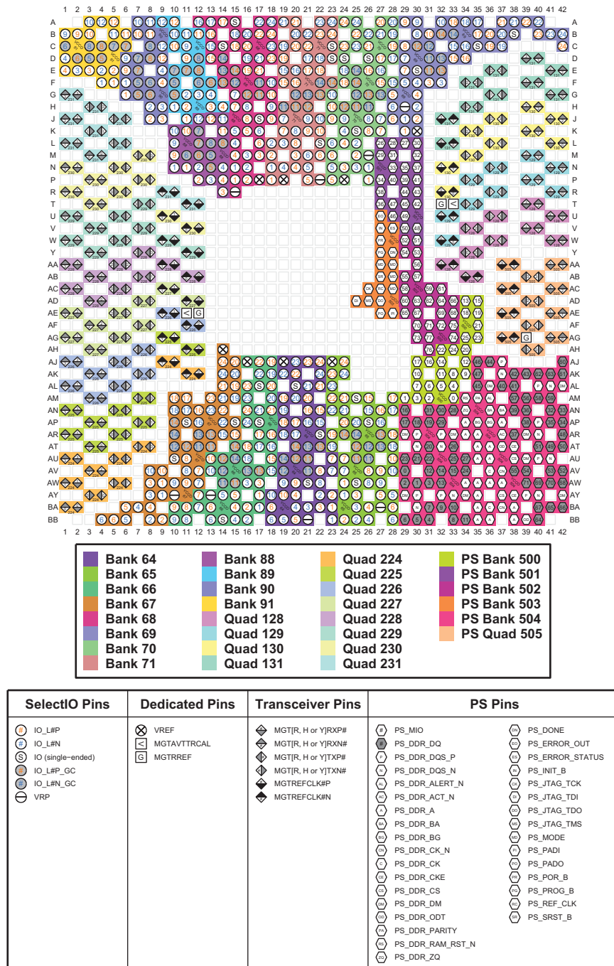
Figure 4-89: FFVC1760 Package—XCZU11EG I/O Bank Diagram
