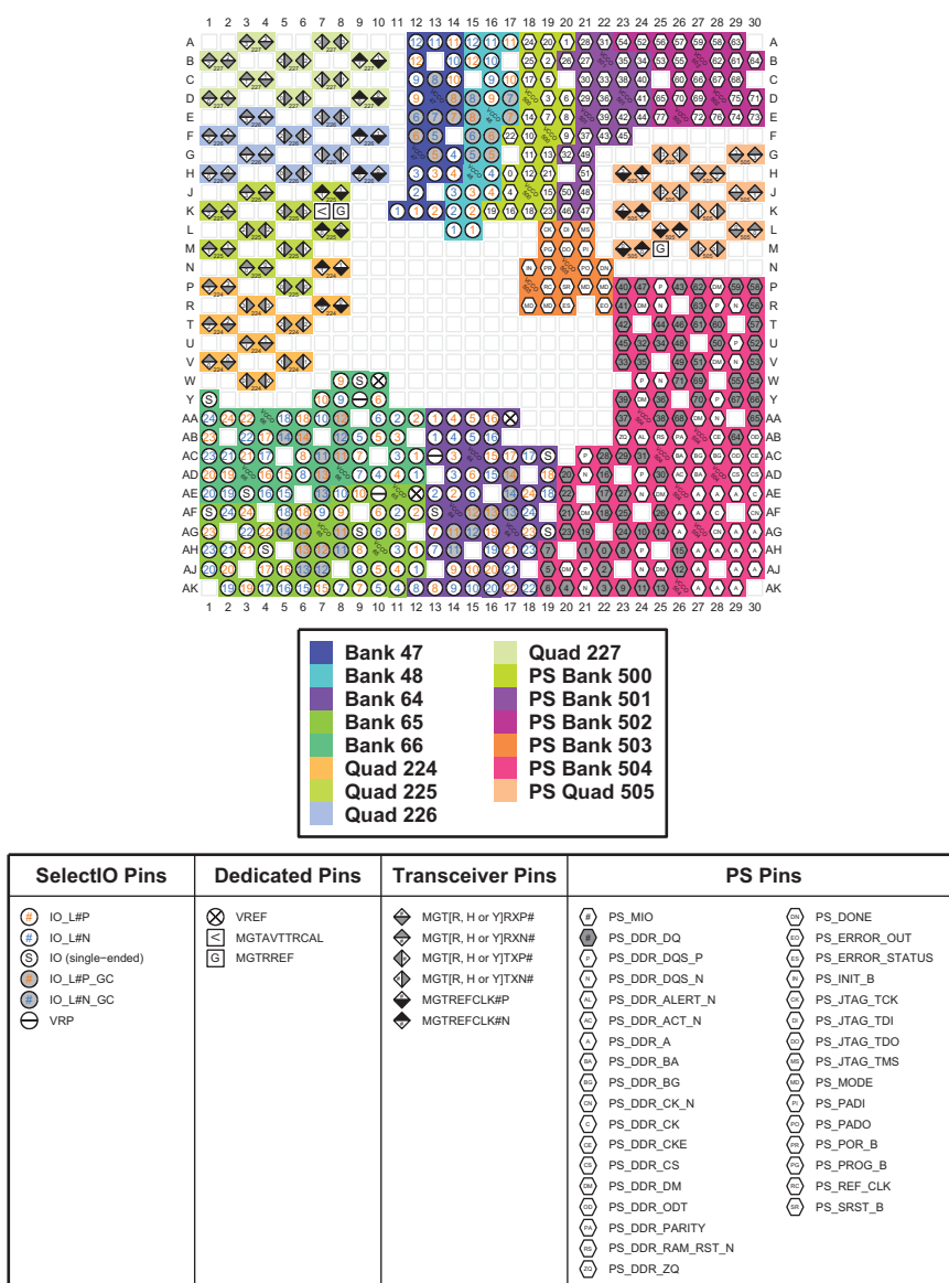
Figure 4-35: FBVB900 Package—XCZU7EV I/O Bank Diagram
