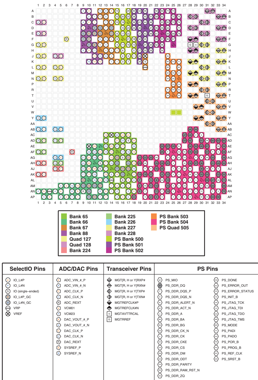
Figure 4-65: FFVE1156 and FSVE1156 Packages—XCZU65DR I/O Bank Diagram
