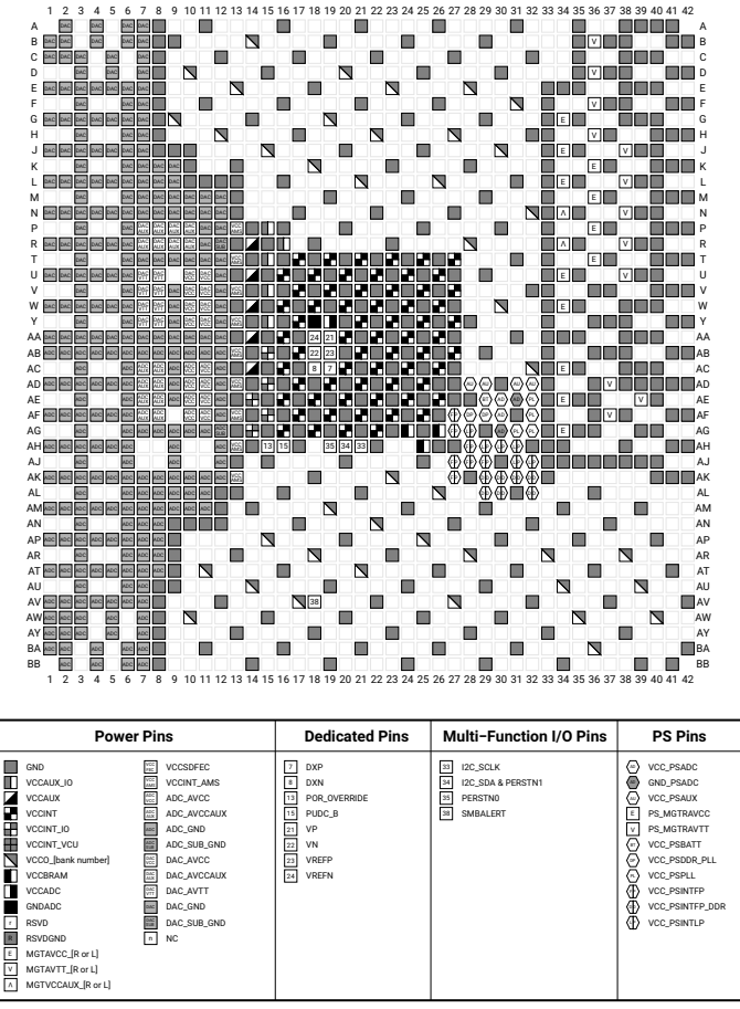
Figure 4-98: FFFV1760, FSFV1760, FSFV1760 Packages—XCZU49DR, XQZU49DR Power, Dedicated, and Multi-function Pin Diagram
