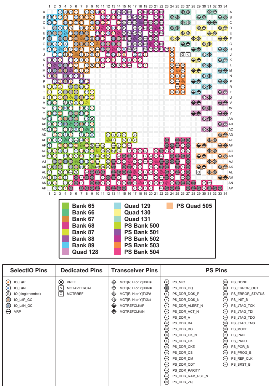
Figure 4-47: FFVD1156 Package—XCZU21DR I/O Bank Diagram
