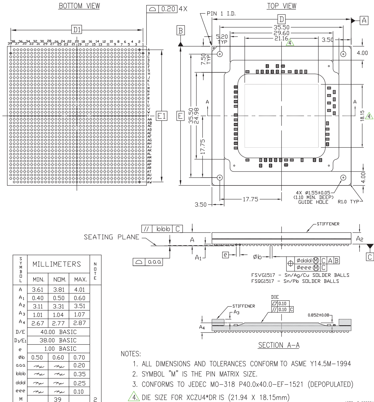
Figure 5-29: Package Dimensions for FSVG1517 (XCZU25DR, XCZU27DR, XCZU28DR, XCZU43DR, XCZU47DR, XCZU48DR)
