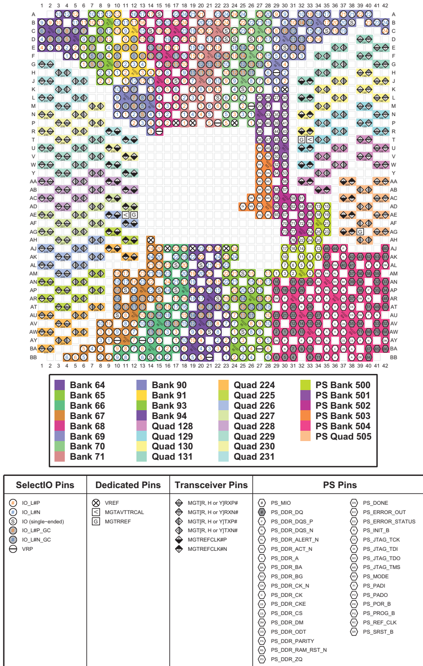
Figure 4-91: FFVC1760 Package—XCZU17EG and XCZU19EG I/O Bank Diagram
