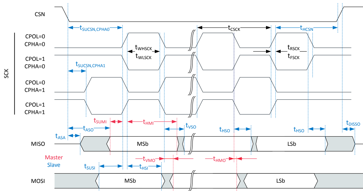
Figure 80: Common SPI and SPIM timing diagram
