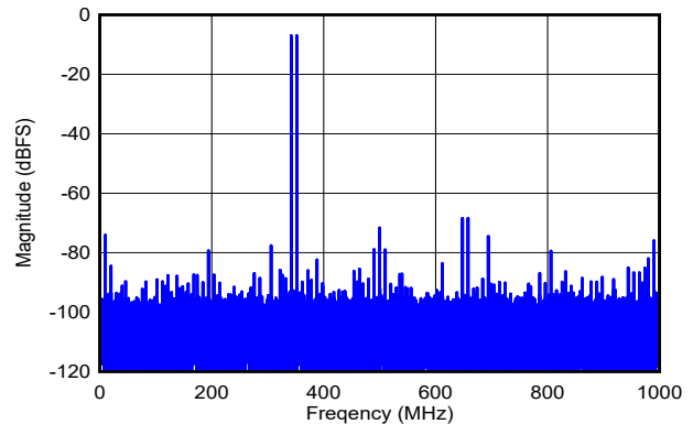
DES_EN = 1, f_s = 2000\text{MHz} , FG calibration, f_1 = 342\text{MHz} , f_2 = 352\text{MHz} , A_{\text{IN}} = -7\text{dBFS} per tone, SFDR = -68dBFS, IMD3 = -89dBFS, IMD2 = -74dBFS
