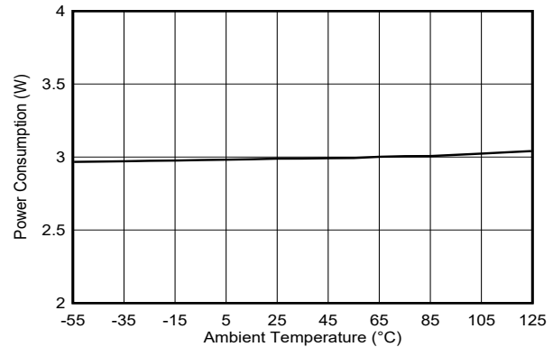
Figure 5-277. Power Consumption vs Temperature
