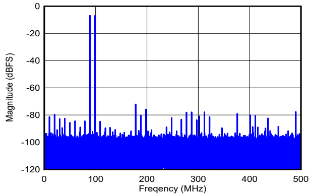
DES_EN = 0, f_s = 1000\text{MHz} , FG calibration, f_1 = 89\text{MHz} , f_2 = 99\text{MHz} , A_{\text{IN}} = -7\text{dBFS} per tone, SFDR = -72dBFS, IMD3 = -85dBFS, IMD2 = -81dBFS
