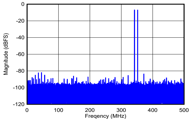
DES_EN = 0, f_s = 1000\text{MHz} , FG calibration, f_1 = 342\text{MHz} , f_2 = 352\text{MHz} , A_{\text{IN}} = -7\text{dBFS} per tone, SFDR = -82dBFS, IMD3 = -96dBFS, IMD2 = -89dBFS
