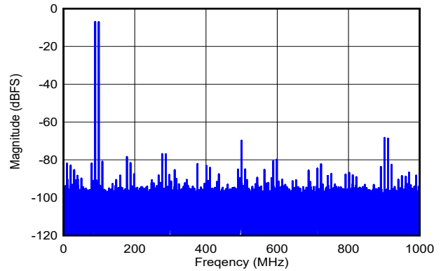
DES_EN = 1, f_s = 2000\text{MHz} , FG calibration, f_1 = 89\text{MHz} , f_2 = 99\text{MHz} , A_{\text{IN}} = -7\text{dBFS} per tone, SFDR = -68dBFS, IMD3 = -81dBFS, IMD2 = -82dBFS
