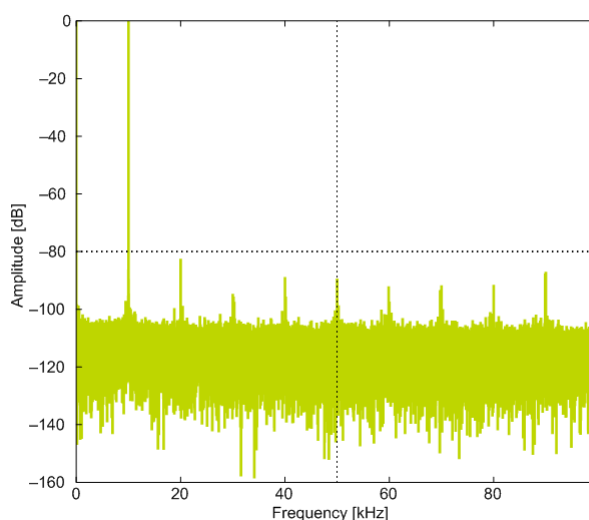
5VDIFF Reference
