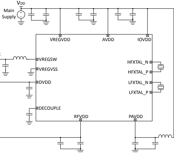
Figure 5.3. EFR32MG1 Typical Application Circuit: Configuration with DC-DC converter (PAVDD from VDD)
