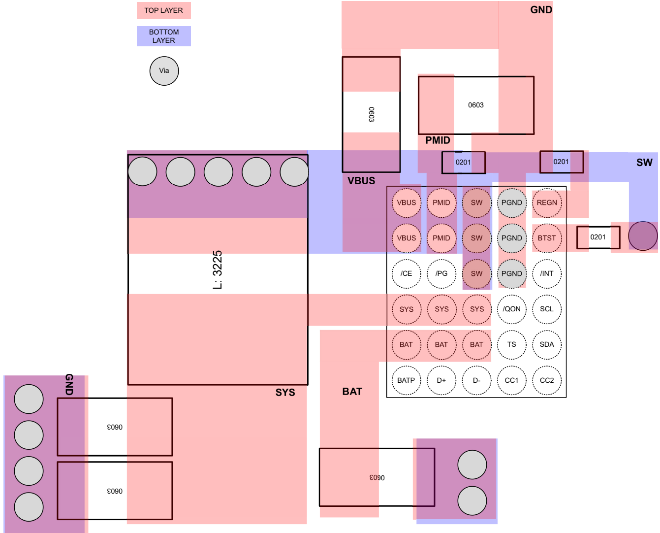
Figure 9-15. Layout
