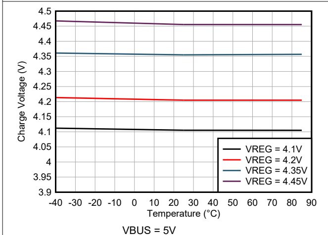
Figure 7-7. BAT Regulation Voltage vs Temperature VBUS = 5V
