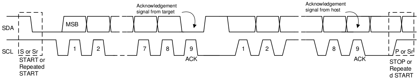
Figure 8-13. Data Transfer on the I 2 C Bus
