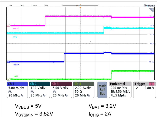
Figure 9-5. Power-Up Sequence
