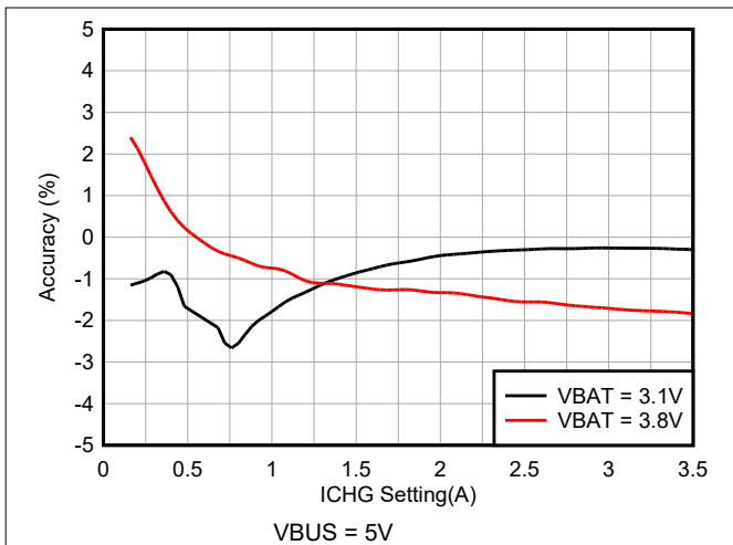
Figure 7-5. Charge Current Accuracy vs Charge Current I 2 C Setting VBUS = 5V
