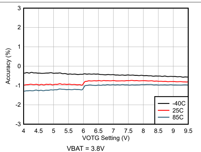
Figure 7-6. Boost Mode Voltage Accuracy vs VOTG I 2 C Setting VBAT = 3.8V
