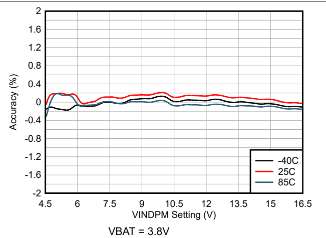
Figure 7-8. Input Voltage Limit vs VINDPM I 2 C Setting VBAT = 3.8V
