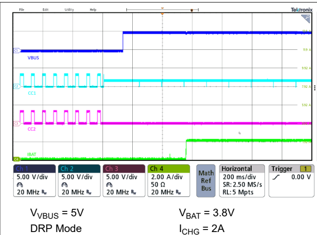
Figure 9-3. USB-C Adapter Plug-In, DRP Mode
