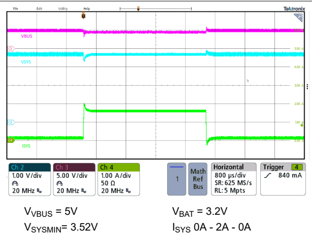
Figure 9-11. SYS Transient
