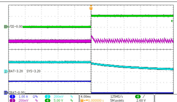
Figure 9-4. Power-Down
