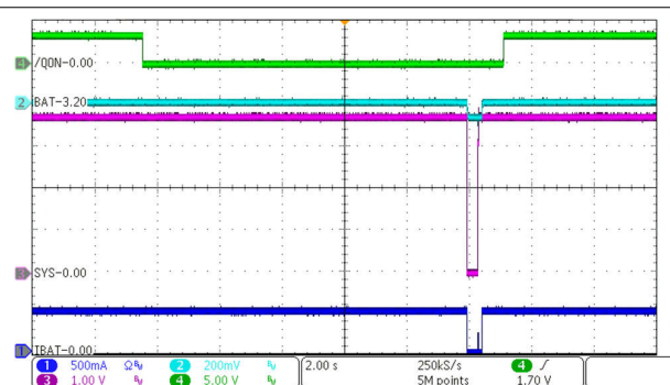
Figure 9-6. Charge Disable
