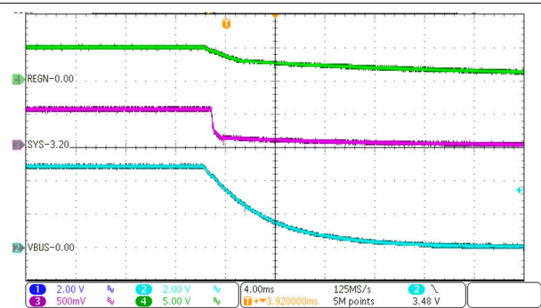
Figure 9-4. Power-Down
